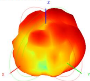
2450.0MHz H+V, Eff: 54.0%
