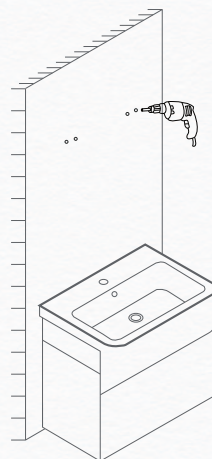
3. Drill the marks with an electric drill.
