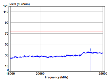
BLE 1M_TX_CH_M_Vertical
