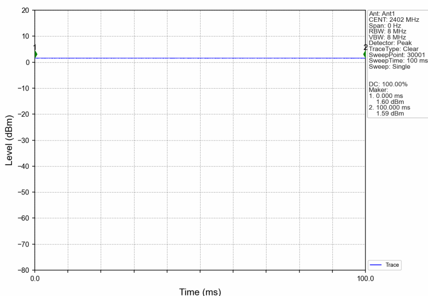
2M_LCH_2402MHz_Ant1_NTNV
