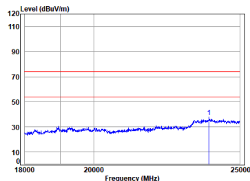
BLE 2M_TX_CH_M_Vertical
