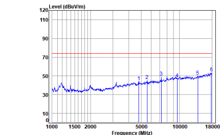
BLE_1M_TX_CH_00_Vertical-Peak
