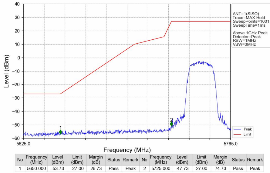
802.11a_LCH_5745MHz_Ant1_NTNV
