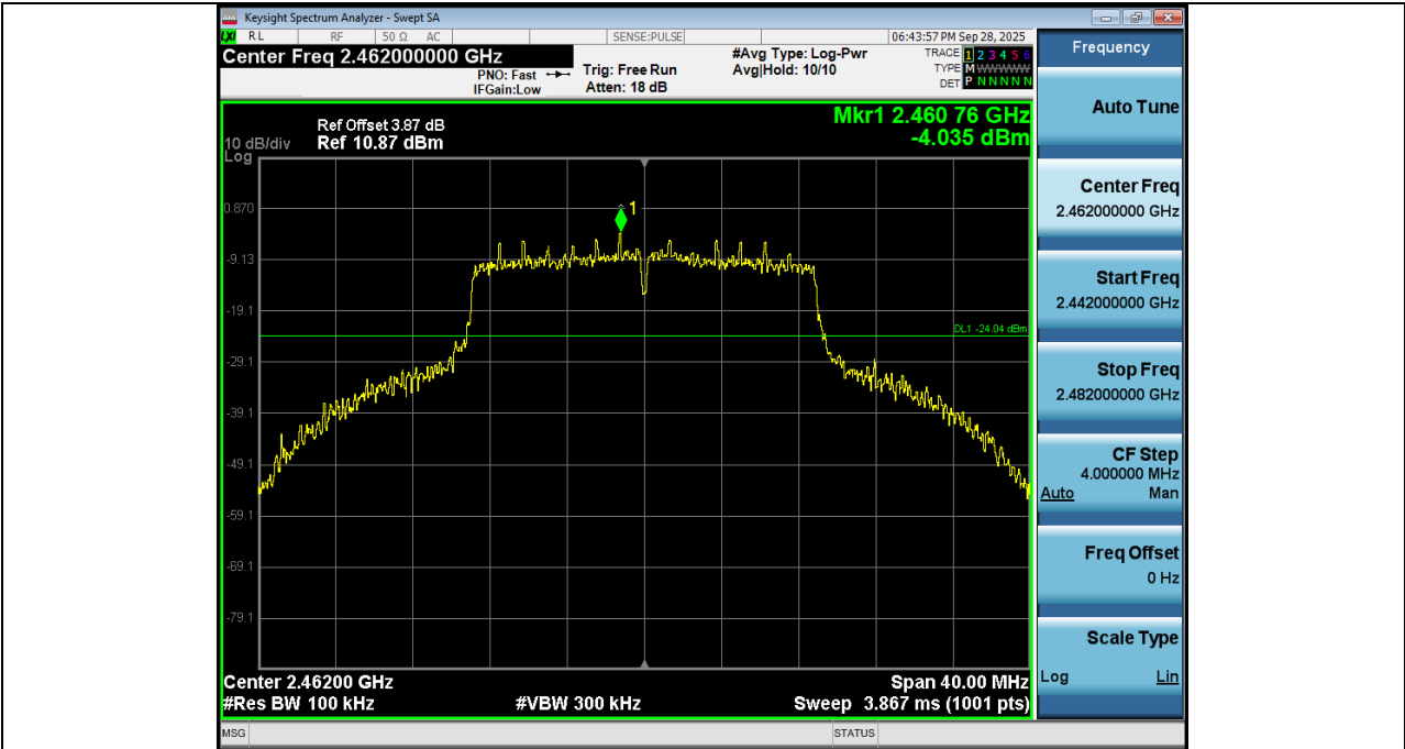
2. Bandedge NVNT_ANT1_802_11n(HT20)_2462
