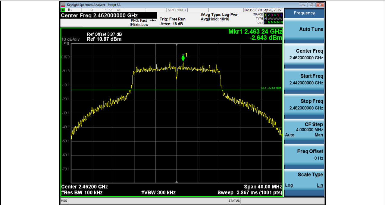
2. Bandedge NVNT_ANT1_802_11g_2462
