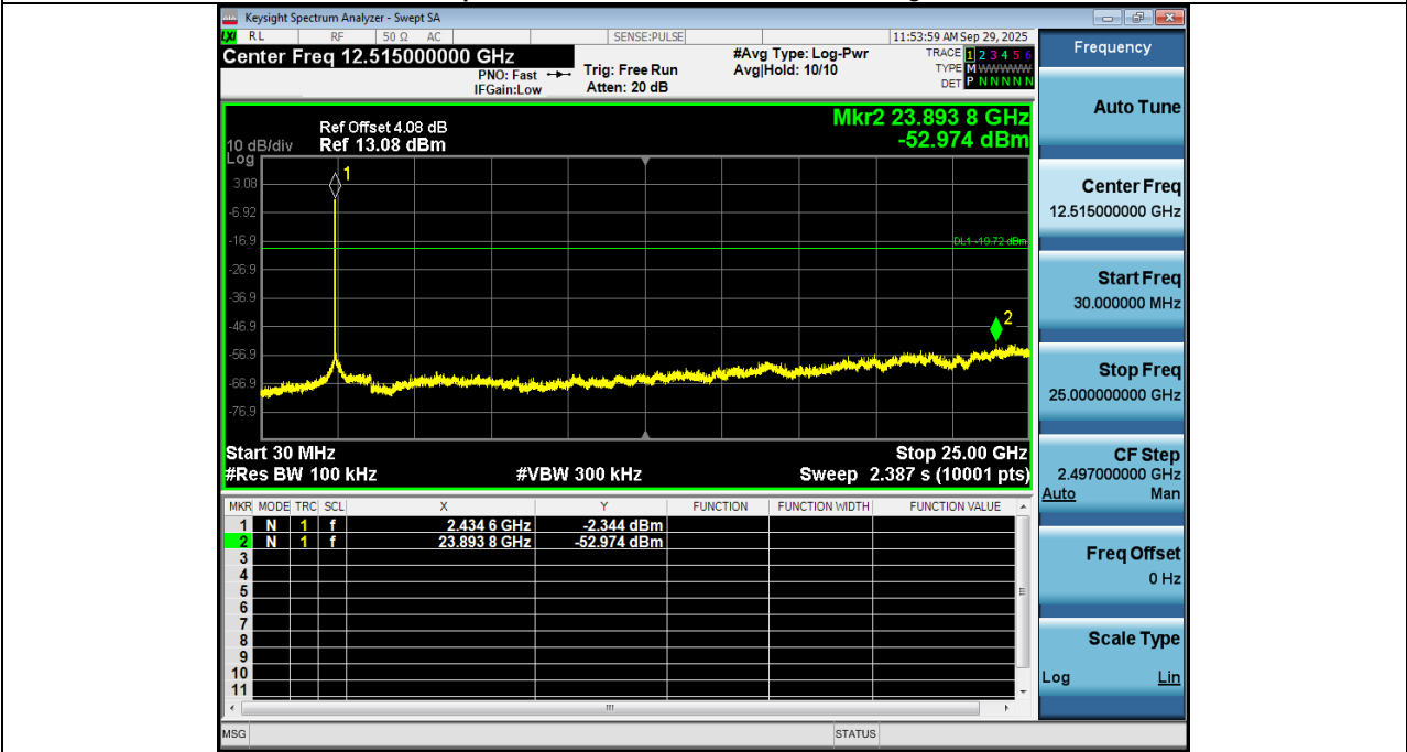
2. Spurious Emission NVNT_ANT1_802_11g_2437
