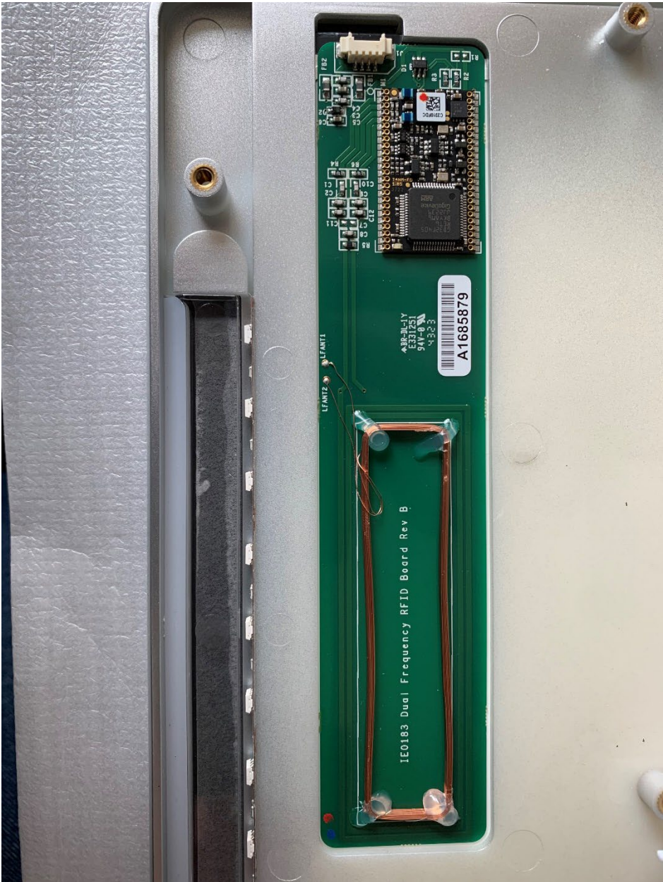
Top View PCB 3, with Coil
