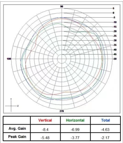
Radiation Pattern:
