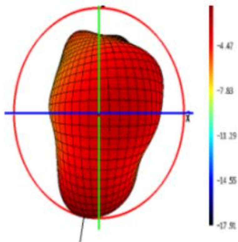
Phi=0 freq=1575.42004394531MHz
