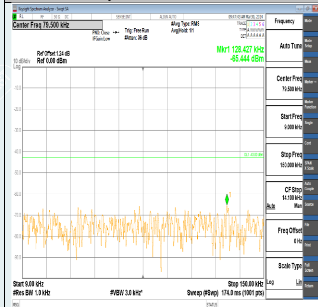
Band2-5MHz-16QAM-19175-1RB#0-0.009~0.15-PASS
