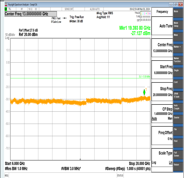
Band2-5MHz-16QAM-18625-25RB#0-6000~20000-PASS
