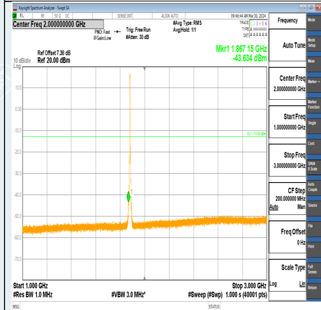
Band2-5MHz-16QAM-18900-25RB#0-1000~3000-PASS
