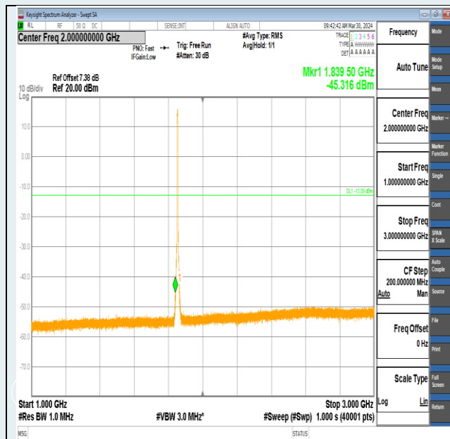
Band2-5MHz-16QAM-18625-25RB#0-1000~3000-PASS
