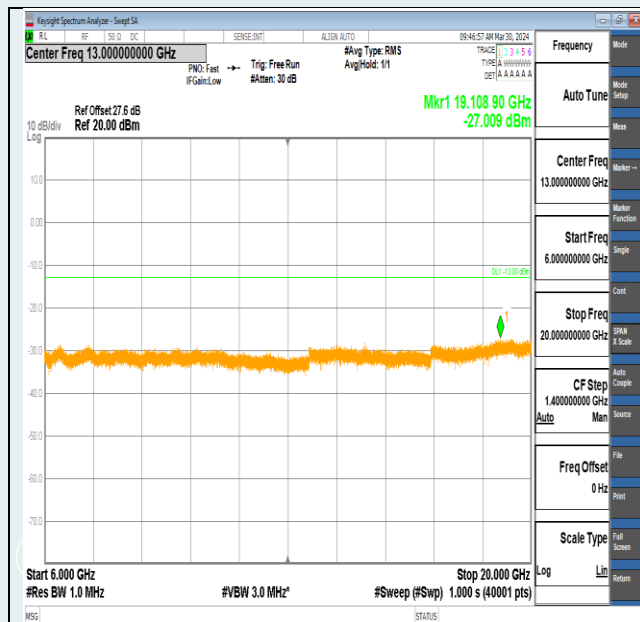
Band2-5MHz-16QAM-18900-25RB#0-6000~20000-PASS
