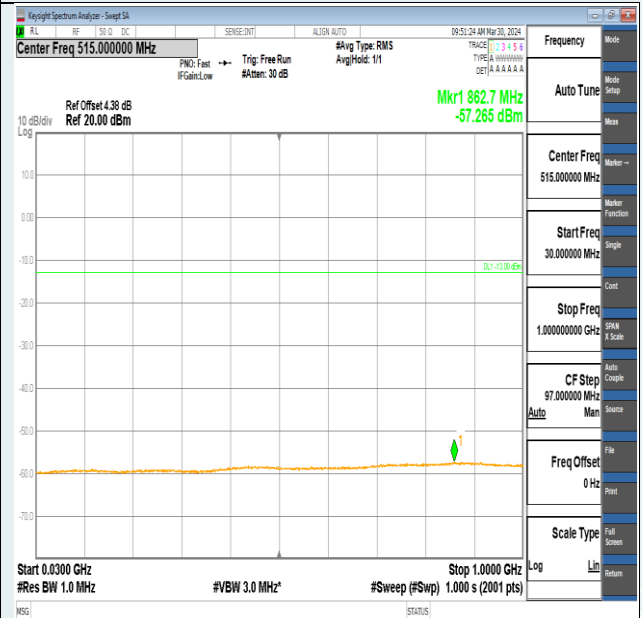
Band2-5MHz-QPSK-19175-25RB#0-30~1000-PASS
