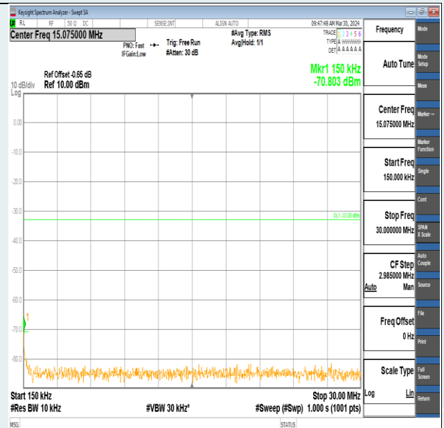
Band2-5MHz-16QAM-19175-1RB#0-0.15~30-PASS
