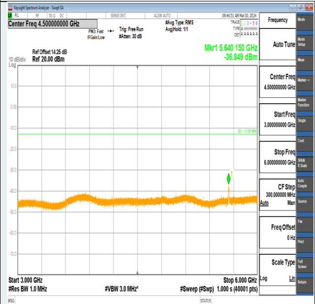
Band2-5MHz-16QAM-18900-25RB#0-3000~6000-PASS
