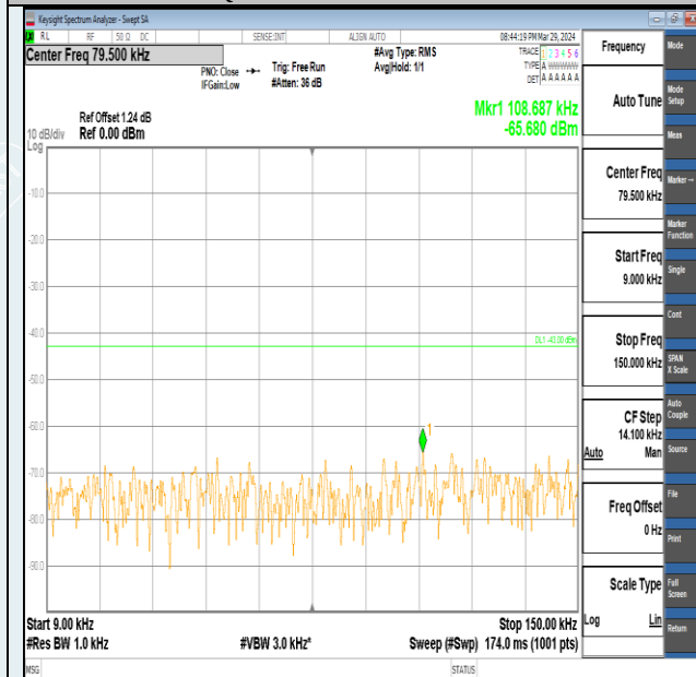
Band2-10MHz-QPSK-18900-50RB#0-0.009~0.15-PASS
