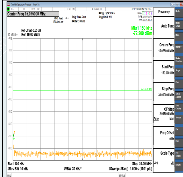
Band2-10MHz-QPSK-19150-1RB#0-0.15~30-PASS
