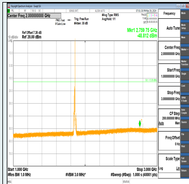
Band2-10MHz-QPSK-18650-1RB#49-1000~3000-PASS
