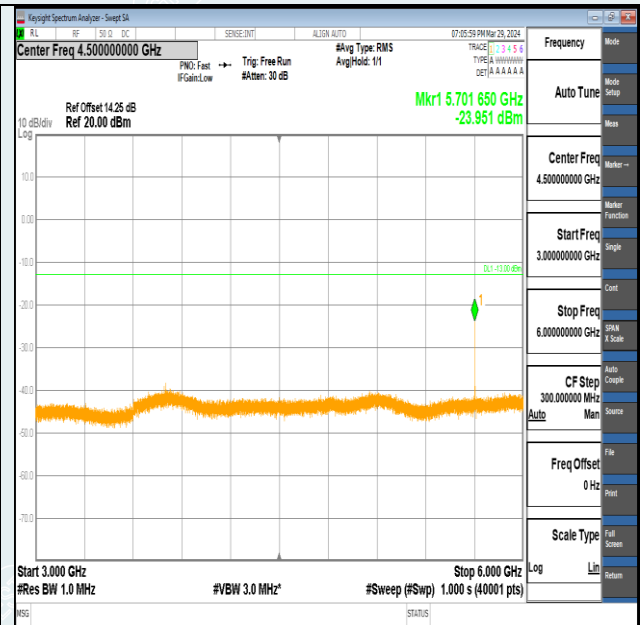
Band2-10MHz-QPSK-19150-1RB#0-3000~6000-PASS
