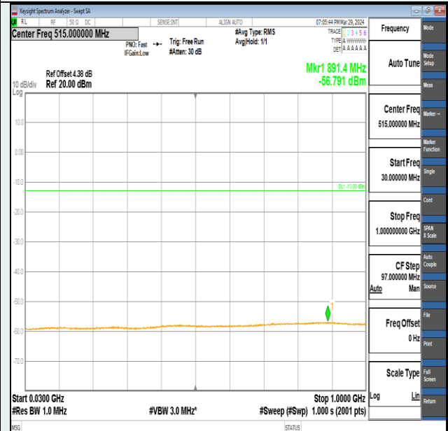
Band2-10MHz-QPSK-19150-1RB#0-30~1000-PASS
