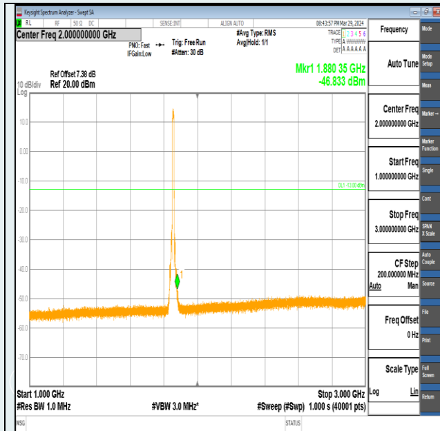
Band2-10MHz-QPSK-18650-50RB#0-1000~3000-PASS
