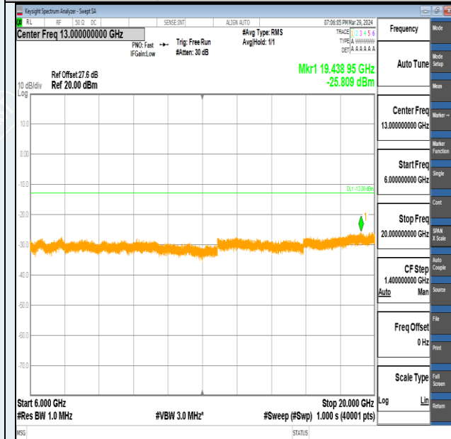
Band2-10MHz-QPSK-19150-1RB#0-6000~20000-PASS
