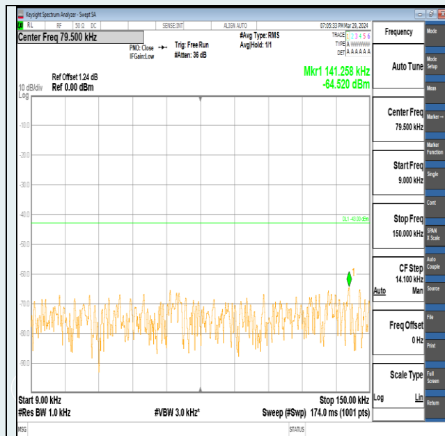
Band2-10MHz-QPSK-19150-1RB#0-0.009~0.15-PASS
