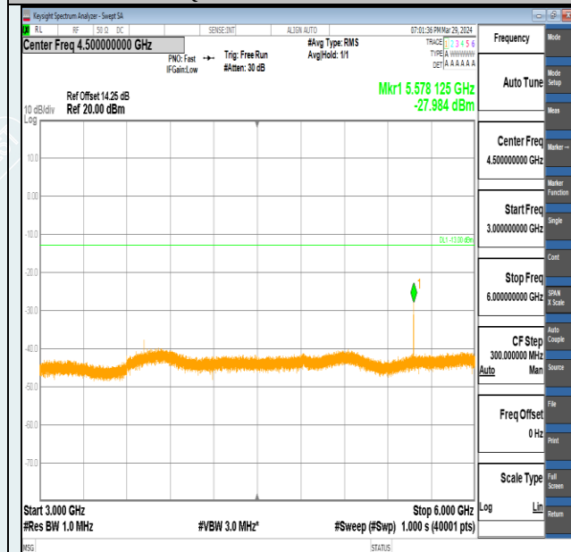
Band2-10MHz-QPSK-18650-1RB#49-3000~6000-PASS
