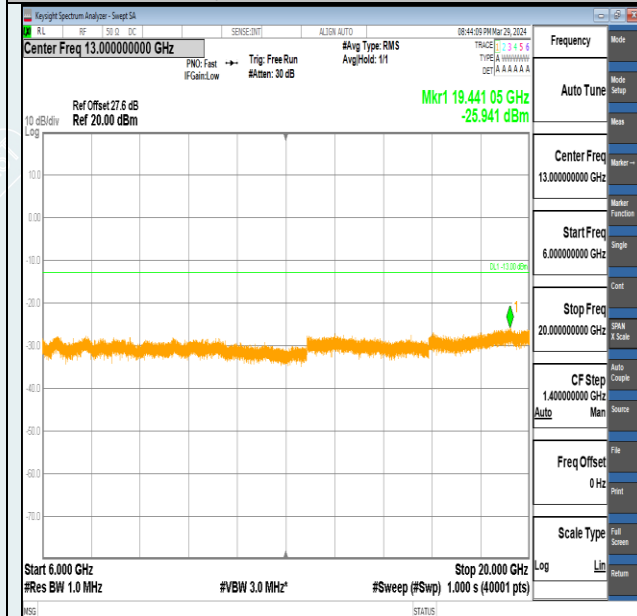
Band2-10MHz-QPSK-18650-50RB#0-6000~20000-PASS
