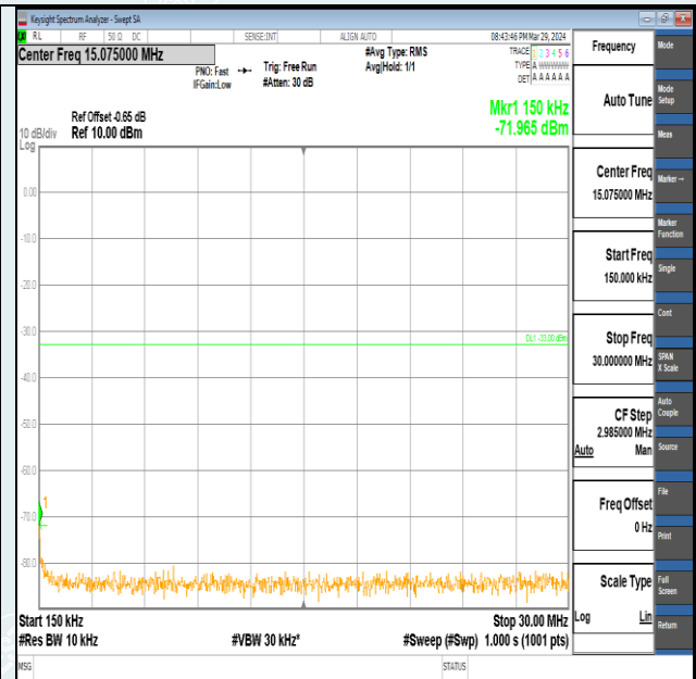
Band2-10MHz-QPSK-18650-50RB#0-0.15~30-PASS
