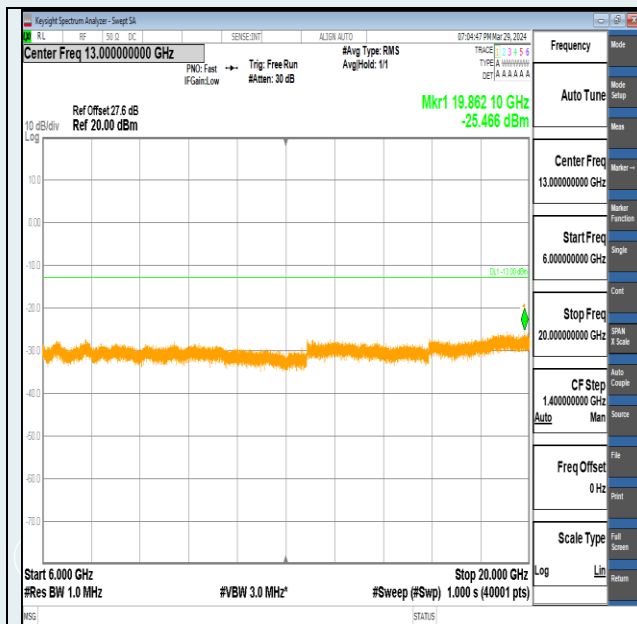
Band2-10MHz-QPSK-18900-1RB#49-6000~20000-PASS
