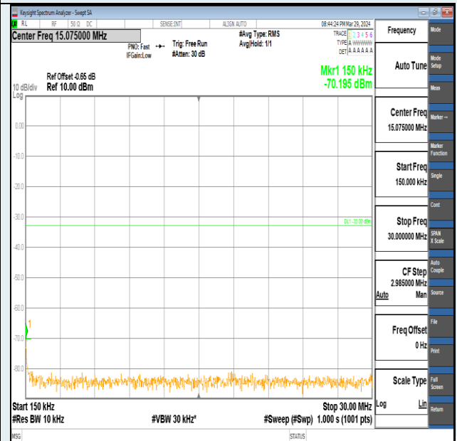
Band2-10MHz-QPSK-18900-50RB#0-0.15~30-PASS
