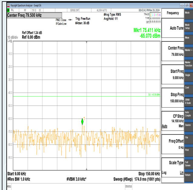
Band2-10MHz-QPSK-18650-50RB#0-0.009~0.15-PASS
