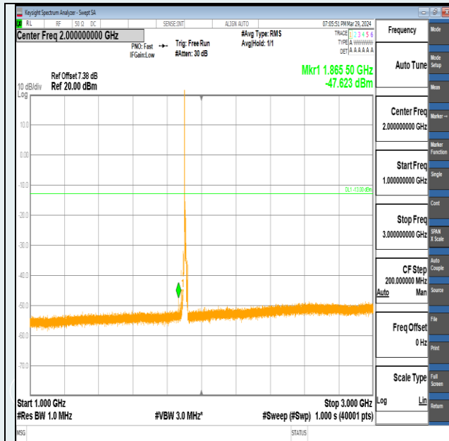
Band2-10MHz-QPSK-19150-1RB#0-1000~3000-PASS
