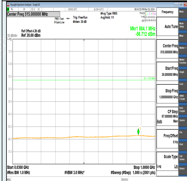
Band2-10MHz-QPSK-18650-50RB#0-30~1000-PASS
