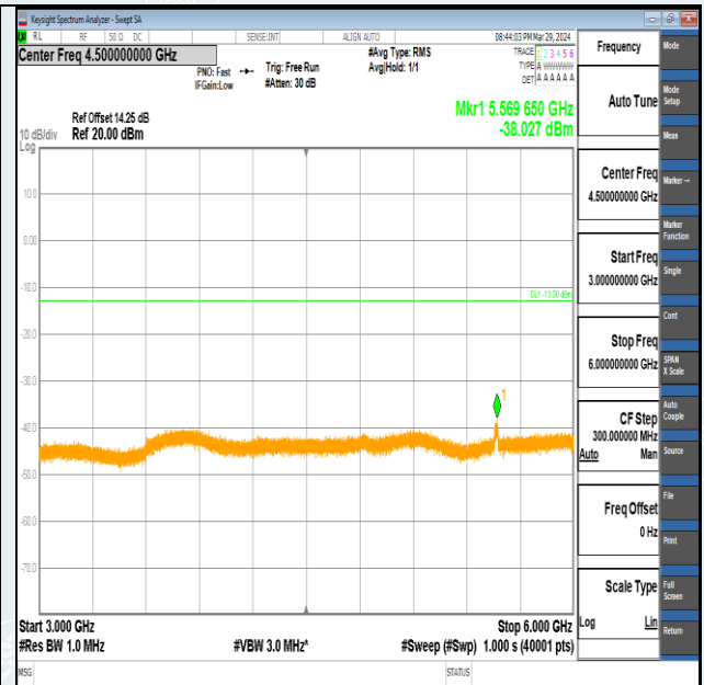
Band2-10MHz-QPSK-18650-50RB#0-3000~6000-PASS
