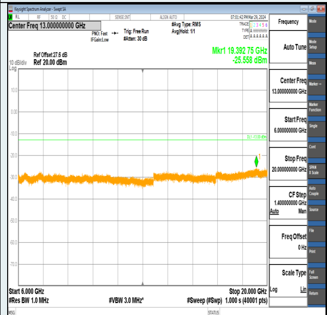
Band2-10MHz-QPSK-18650-1RB#49-6000~20000-PASS
