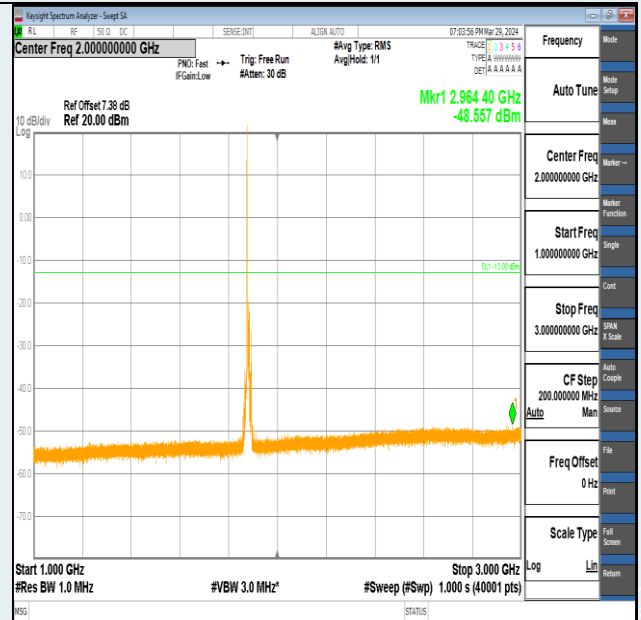
Band2-10MHz-16QAM-18900-1RB#0-1000~3000-PASS
