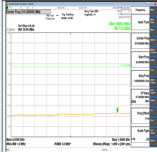
Band2-10MHz-16QAM-18900-1RB#0-30~1000-PASS
