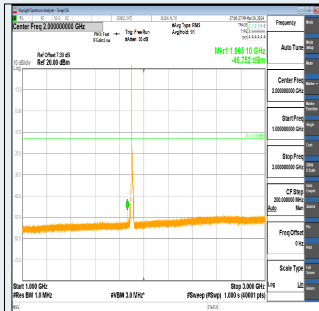
Band2-10MHz-16QAM-19150-1RB#0-1000~3000-PASS
