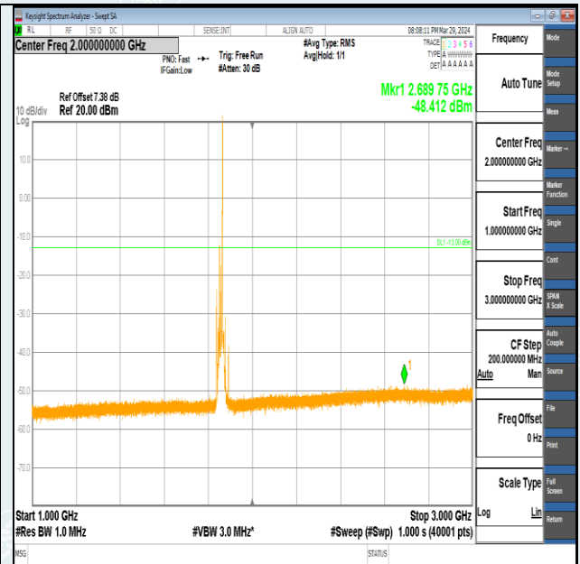
Band2-15MHz-QPSK-18675-1RB#74-1000~3000-PASS
