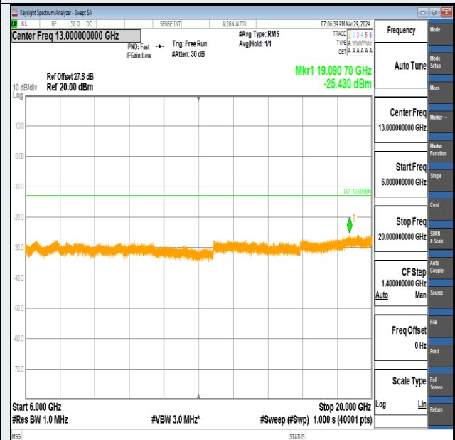
Band2-10MHz-16QAM-19150-1RB#0-6000~20000-PASS
