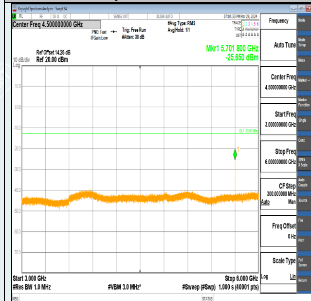
Band2-10MHz-16QAM-19150-1RB#0-3000~6000-PASS
