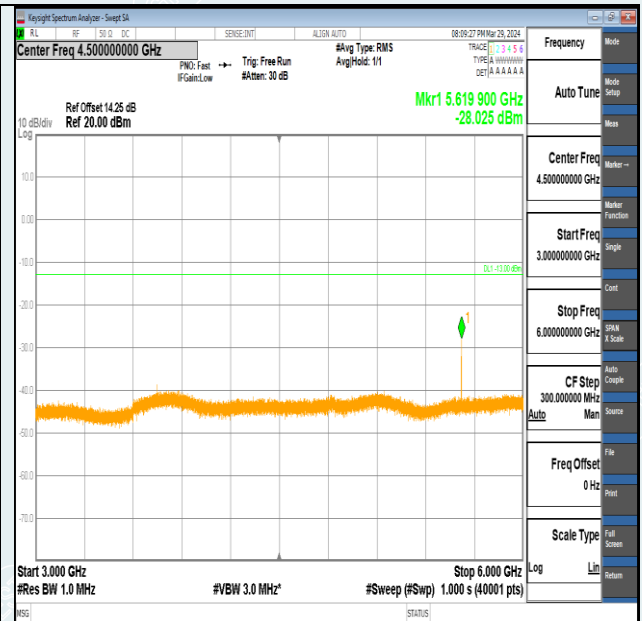
Band2-15MHz-QPSK-18900-1RB#0-3000~6000-PASS
