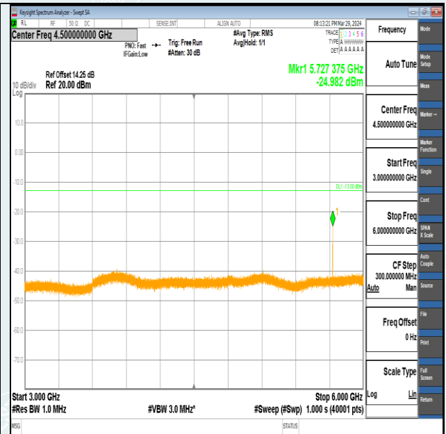
Band2-15MHz-QPSK-19125-1RB#74-3000~6000-PASS
