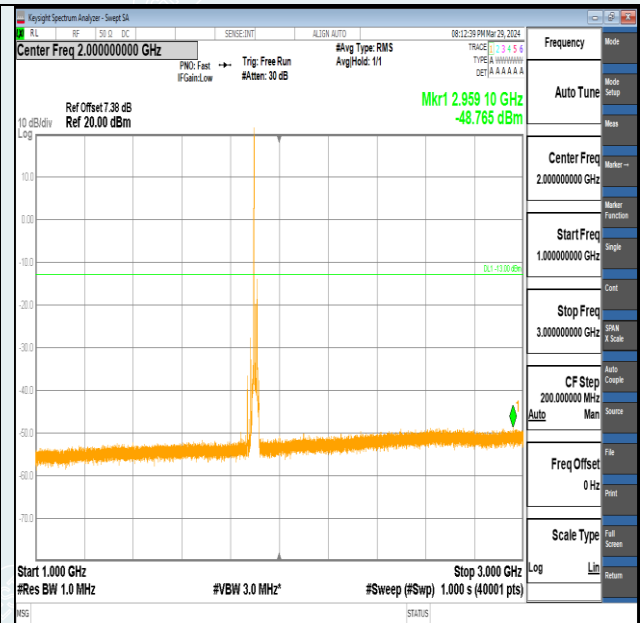
Band2-15MHz-16QAM-19125-1RB#0-1000~3000-PASS
