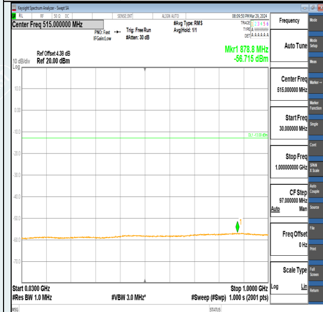
Band2-15MHz-16QAM-18900-1RB#0-30~1000-PASS
