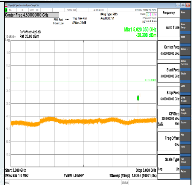
Band2-15MHz-16QAM-18900-1RB#0-3000~6000-PASS
