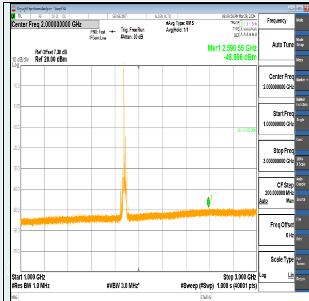
Band2-15MHz-16QAM-18900-1RB#0-1000~3000-PASS
