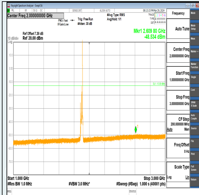
Band2-15MHz-QPSK-19125-1RB#74-1000~3000-PASS
