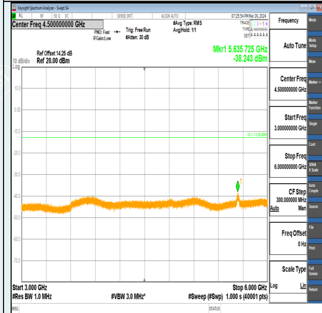
Band2-15MHz-QPSK-18900-75RB#0-3000~6000-PASS
