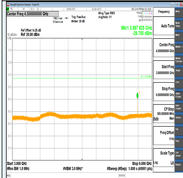
Band2-15MHz-16QAM-19125-1RB#0-3000~6000-PASS
