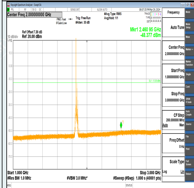
Band2-15MHz-16QAM-18675-1RB#0-1000~3000-PASS
