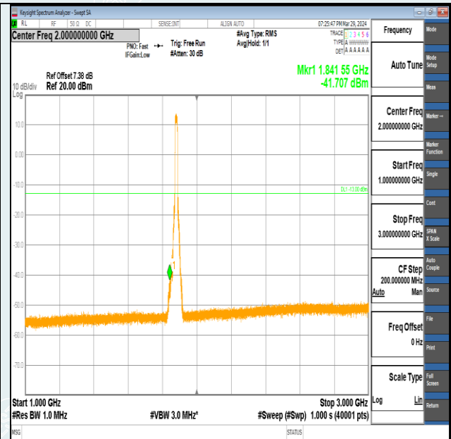
Band2-15MHz-QPSK-18900-75RB#0-1000~3000-PASS
