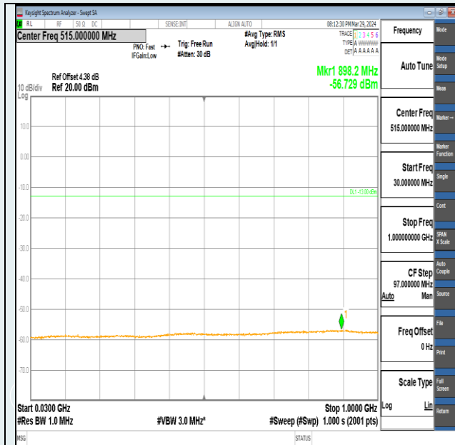
Band2-15MHz-16QAM-19125-1RB#0-30~1000-PASS
