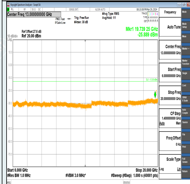
Band2-15MHz-16QAM-18900-1RB#0-6000~20000-PASS
