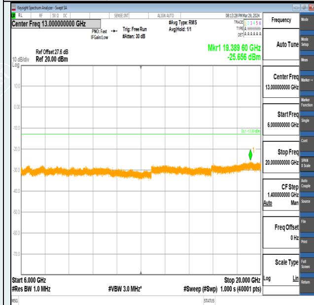
Band2-15MHz-QPSK-19125-1RB#74-6000~20000-PASS
