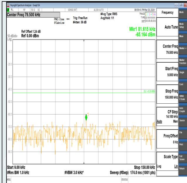
Band2-15MHz-16QAM-18900-1RB#0-0.009~0.15-PASS
