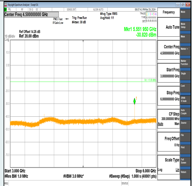
Band2-15MHz-16QAM-18675-1RB#0-3000~6000-PASS
