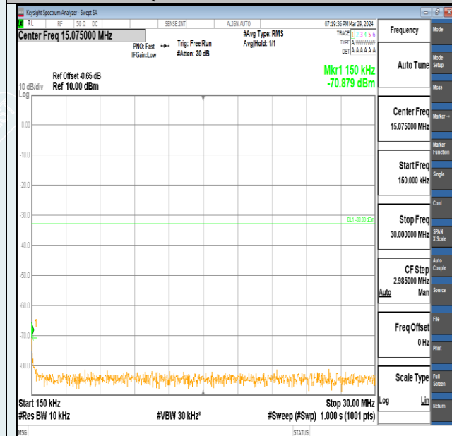
Band2-20MHz-QPSK-18900-1RB#99-0.15~30-PASS
