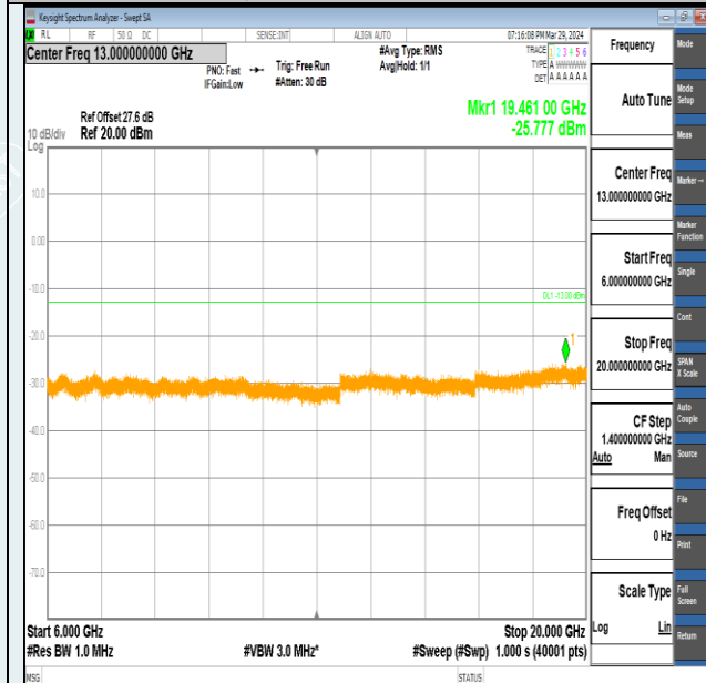
Band2-20MHz-QPSK-18700-1RB#0-6000~20000-PASS
