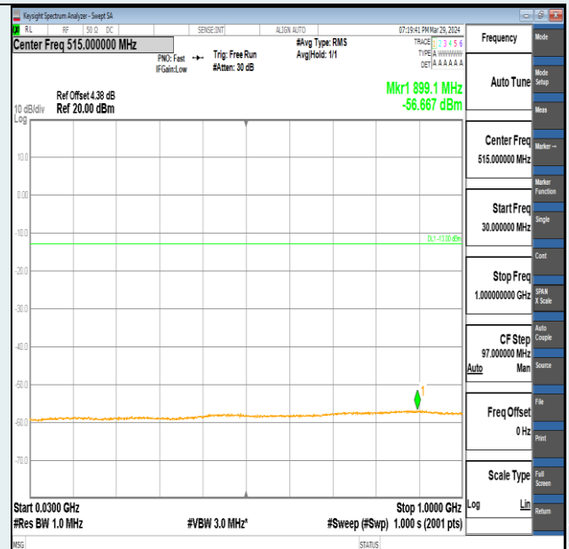
Band2-20MHz-QPSK-18900-1RB#99-30~1000-PASS
