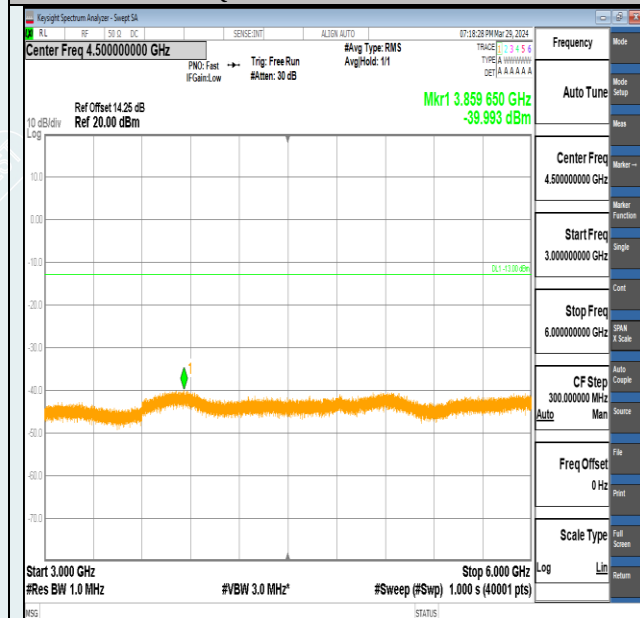
Band2-20MHz-QPSK-18900-1RB#0-3000~6000-PASS
