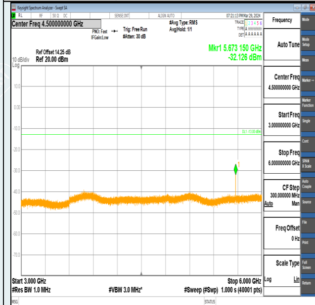
Band2-20MHz-QPSK-19100-1RB#0-3000~6000-PASS
