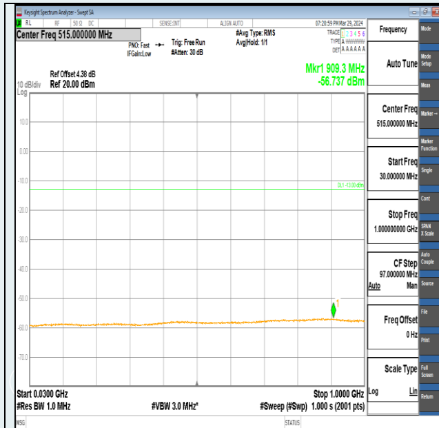
Band2-20MHz-QPSK-19100-1RB#0-30~1000-PASS
