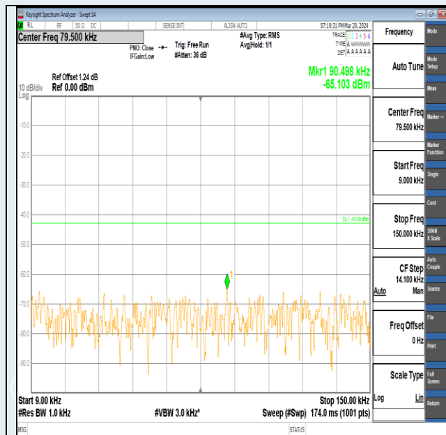
Band2-20MHz-QPSK-18900-1RB#99-0.009~0.15-PASS
