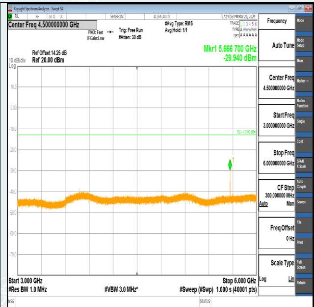
Band2-20MHz-QPSK-18900-1RB#99-3000~6000-PASS
