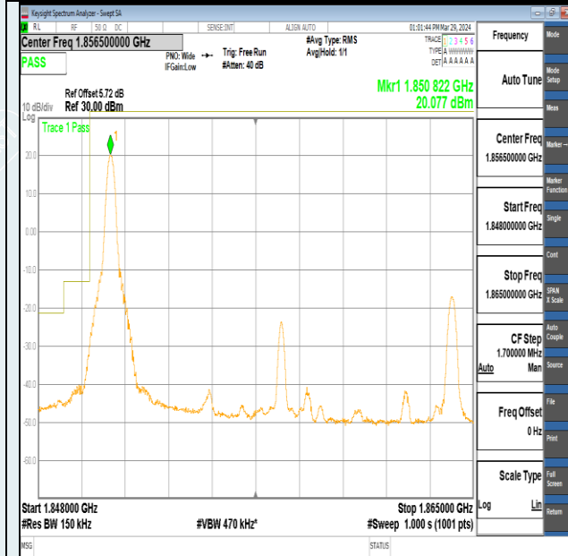
Band2-15MHz-16QAM-18675-1RB#0-PASS
