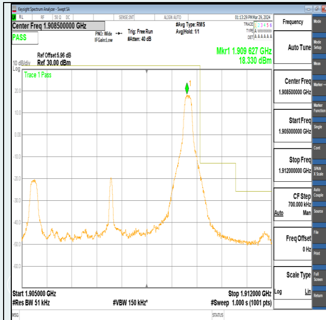
Band2-5MHz-16QAM-19175-1RB#24-PASS
