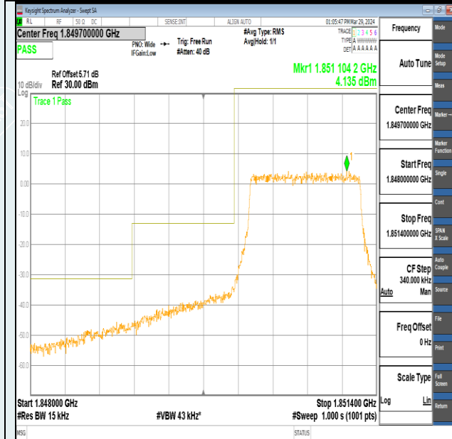
Band2-1.4MHz-16QAM-18607-6RB#0-PASS
