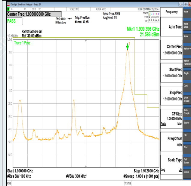
Band2-10MHz-QPSK-19150-1RB#49-PASS
