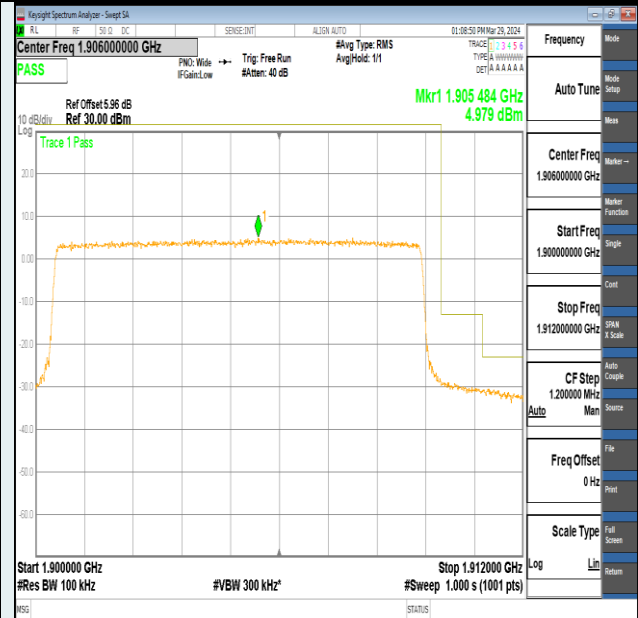
Band2-10MHz-QPSK-19150-50RB#0-PASS
