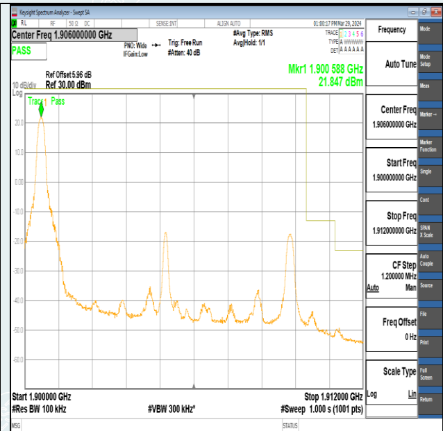
Band2-10MHz-QPSK-19150-1RB#0-PASS
