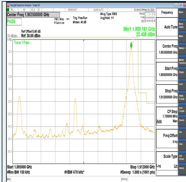
Band2-15MHz-QPSK-19125-1RB#74-PASS
