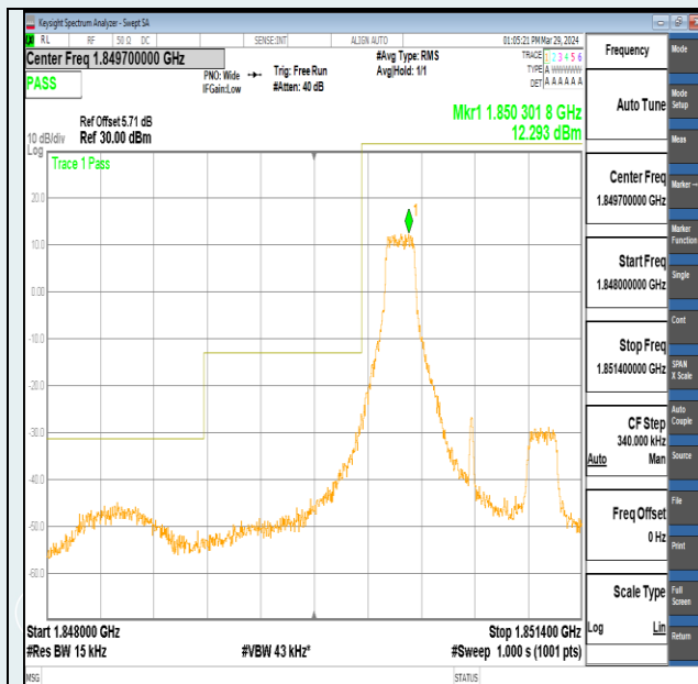
Band2-1.4MHz-16QAM-18607-1RB#0-PASS
