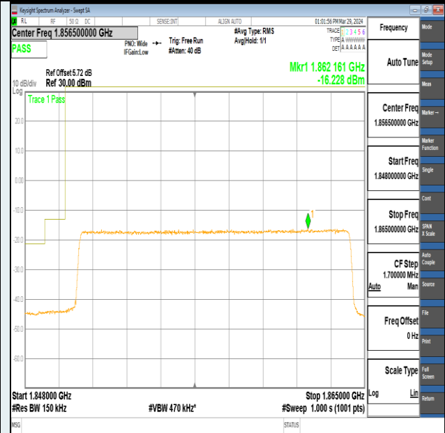
Band2-15MHz-16QAM-18675-1RB#74-PASS
