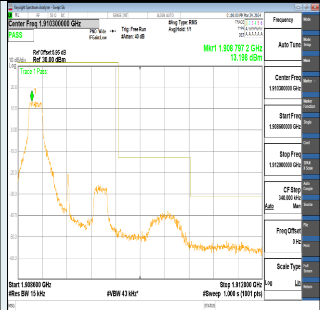
Band2-1.4MHz-16QAM-19193-1RB#0-PASS
