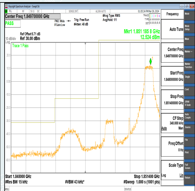
Band2-1.4MHz-16QAM-18607-1RB#5-PASS
