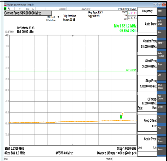
Band2-1.4MHz-QPSK-18900-1RB#5-30~1000-PASS
