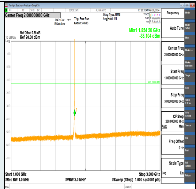
Band2-1.4MHz-QPSK-18607-1RB#5-1000~3000-PASS
