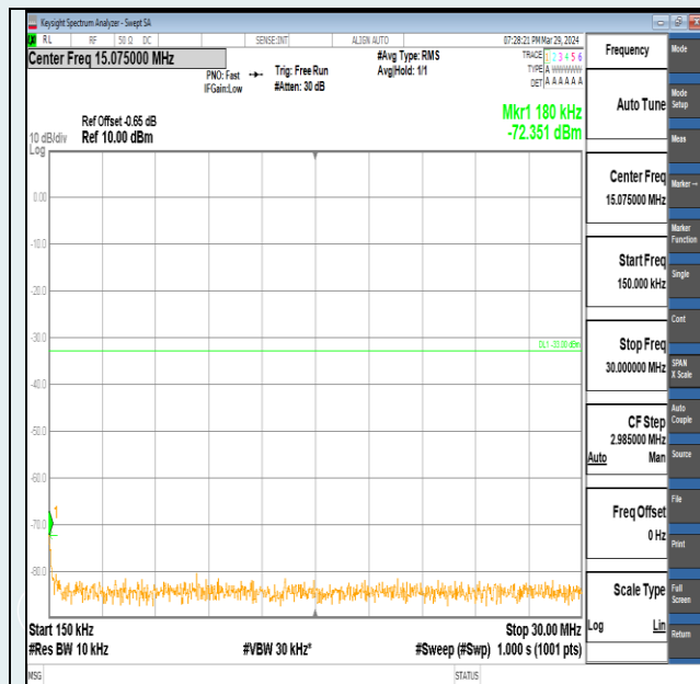
Band2-1.4MHz-QPSK-18607-1RB#5-0.15~30-PASS
