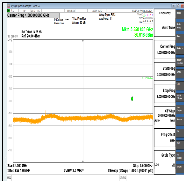
Band2-1.4MHz-QPSK-18607-1RB#0-3000~6000-PASS
