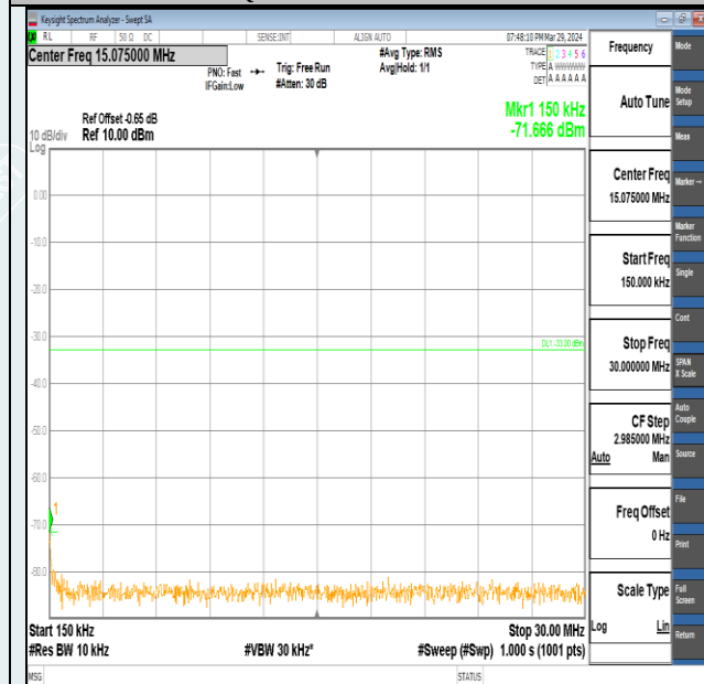
Band2-1.4MHz-QPSK-18900-1RB#5-0.15~30-PASS
