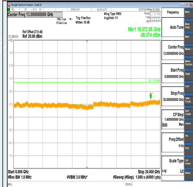
Band2-1.4MHz-QPSK-18607-1RB#0-6000~20000-PASS
