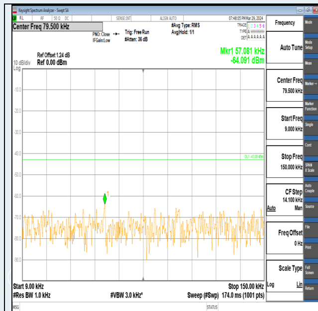
Band2-1.4MHz-QPSK-18900-1RB#5-0.009~0.15-PASS
