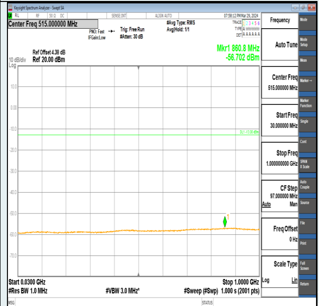
Band2-1.4MHz-QPSK-19193-6RB#0-30~1000-PASS
