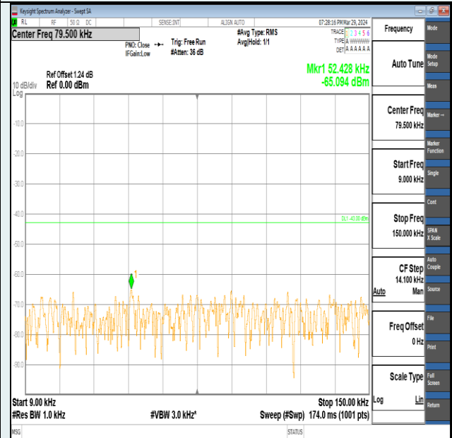
Band2-1.4MHz-QPSK-18607-1RB#5-0.009~0.15-PASS
