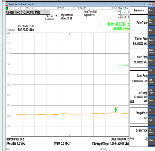
Band2-1.4MHz-QPSK-18607-1RB#5-30~1000-PASS
