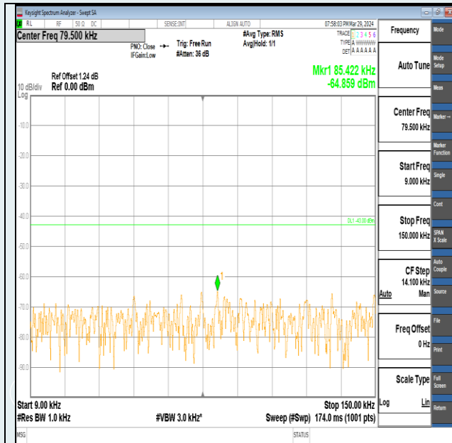
Band2-1.4MHz-QPSK-19193-6RB#0-0.009~0.15-PASS
