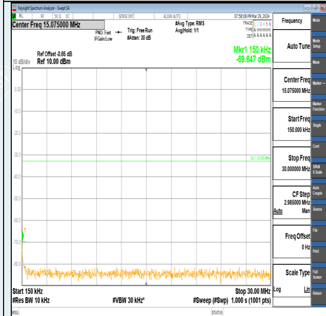
Band2-1.4MHz-QPSK-19193-6RB#0-0.15~30-PASS
