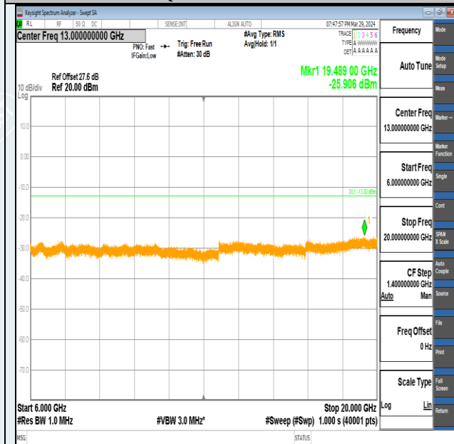
Band2-1.4MHz-16QAM-18900-1RB#0-6000~20000-PASS
