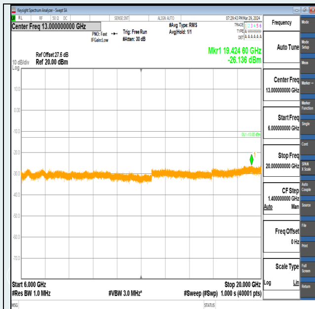
Band2-1.4MHz-16QAM-18607-1RB#5-6000~20000-PASS
