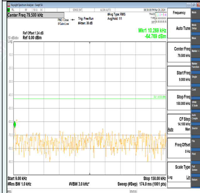
Band2-3MHz-QPSK-18615-1RB#0-0.009~0.15-PASS
