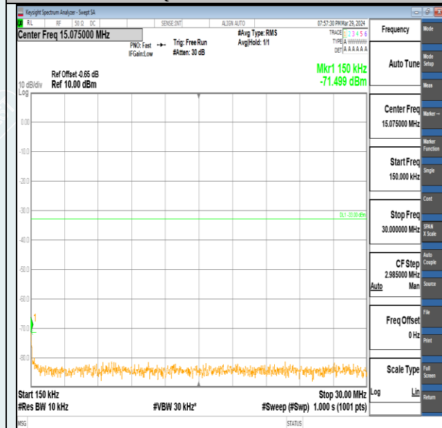
Band2-1.4MHz-16QAM-19193-1RB#5-0.15~30-PASS
