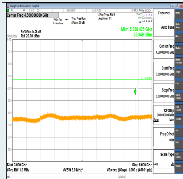
Band2-1.4MHz-16QAM-18900-1RB#0-3000~6000-PASS
