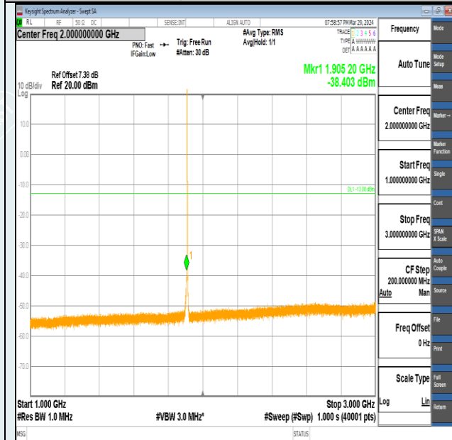
Band2-1.4MHz-16QAM-19193-6RB#0-1000~3000-PASS
