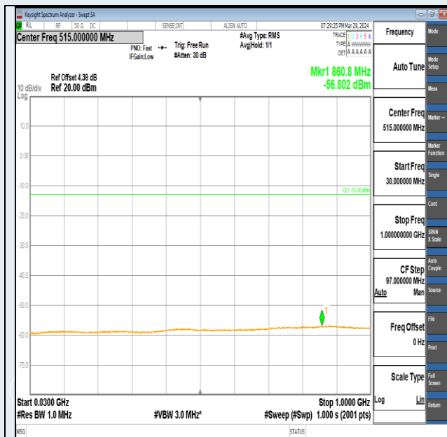
Band2-1.4MHz-16QAM-18607-1RB#5-30~1000-PASS
