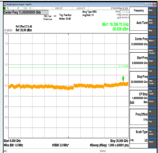
Band2-1.4MHz-16QAM-19193-6RB#0-6000~20000-PASS
