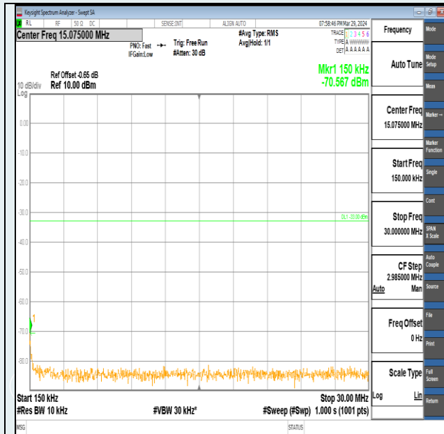
Band2-1.4MHz-16QAM-19193-6RB#0-0.15~30-PASS
