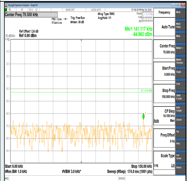
Band2-1.4MHz-16QAM-18900-1RB#5-0.009~0.15-PASS
