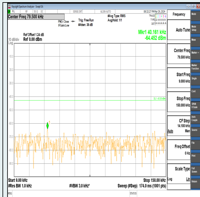
Band2-3MHz-QPSK-18615-15RB#0-0.009~0.15-PASS
