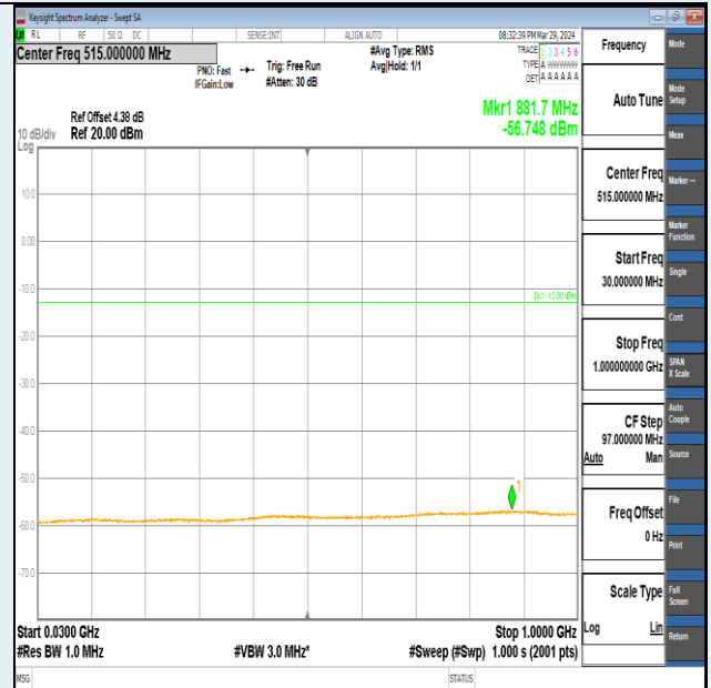
Band2-3MHz-QPSK-18615-15RB#0-30~1000-PASS
