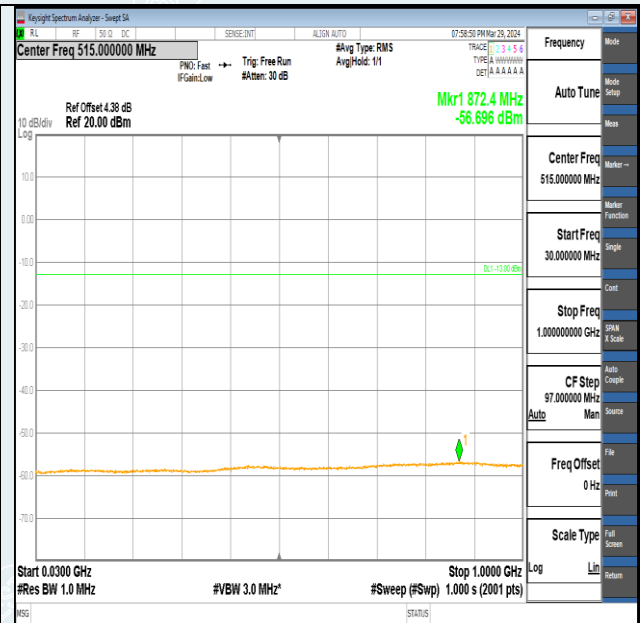
Band2-1.4MHz-16QAM-19193-6RB#0-30~1000-PASS
