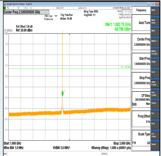
Band2-1.4MHz-16QAM-18900-1RB#5-1000~3000-PASS
