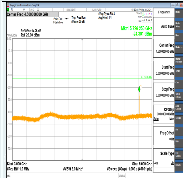
Band2-1.4MHz-16QAM-19193-6RB#0-3000~6000-PASS
