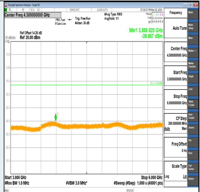
Band2-1.4MHz-16QAM-18607-1RB#5-3000~6000-PASS
