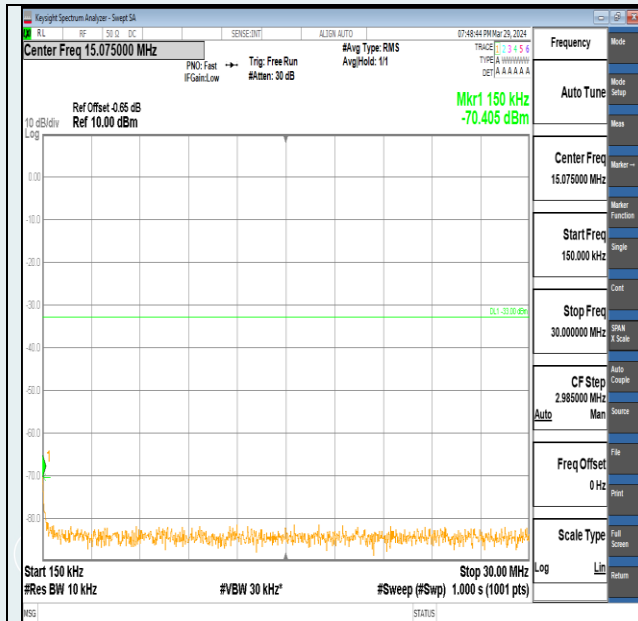
Band2-1.4MHz-16QAM-18900-1RB#5-0.15~30-PASS
