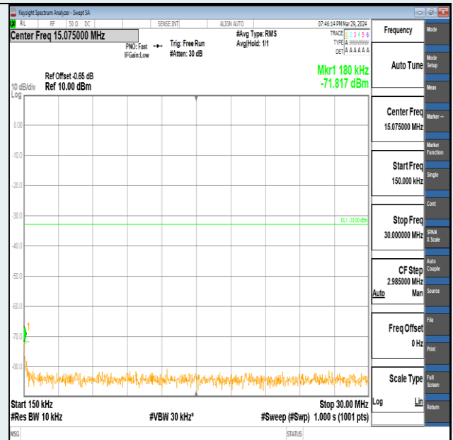
Band2-1.4MHz-16QAM-18607-6RB#0-0.15~30-PASS
