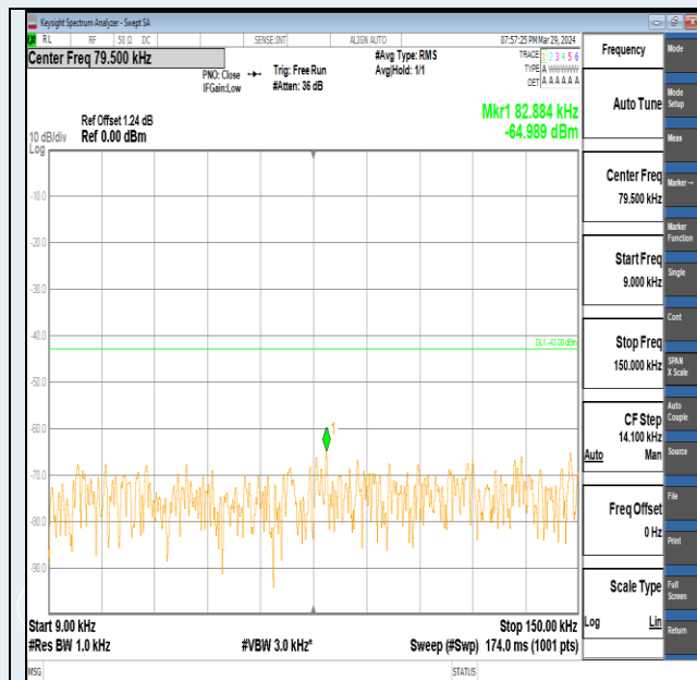
Band2-1.4MHz-16QAM-19193-1RB#5-0.009~0.15-PASS
