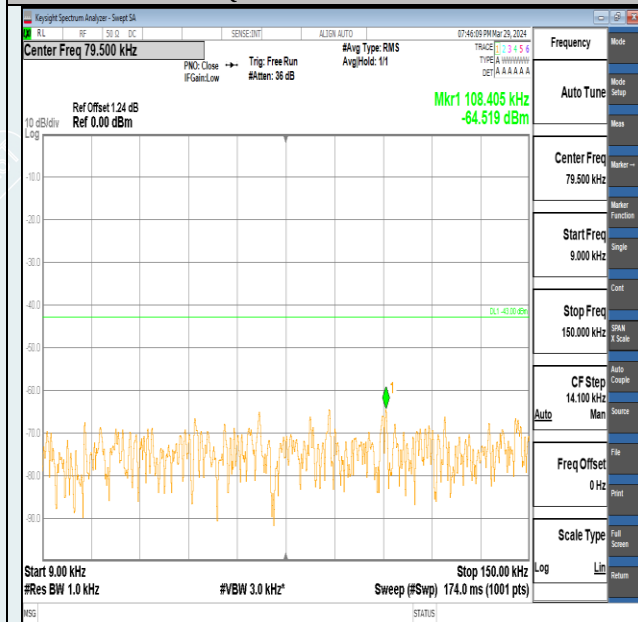
Band2-1.4MHz-16QAM-18607-6RB#0-0.009~0.15-PASS
