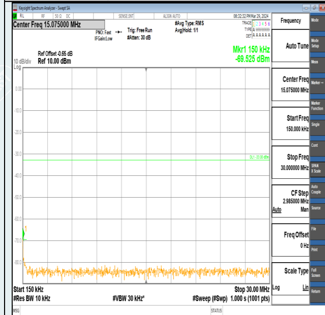
Band2-3MHz-QPSK-18615-15RB#0-0.15~30-PASS
