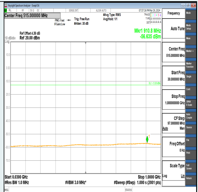
Band2-1.4MHz-16QAM-19193-1RB#5-30~1000-PASS
