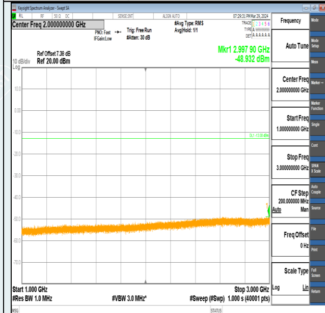
Band2-1.4MHz-16QAM-18607-1RB#5-1000~3000-PASS
