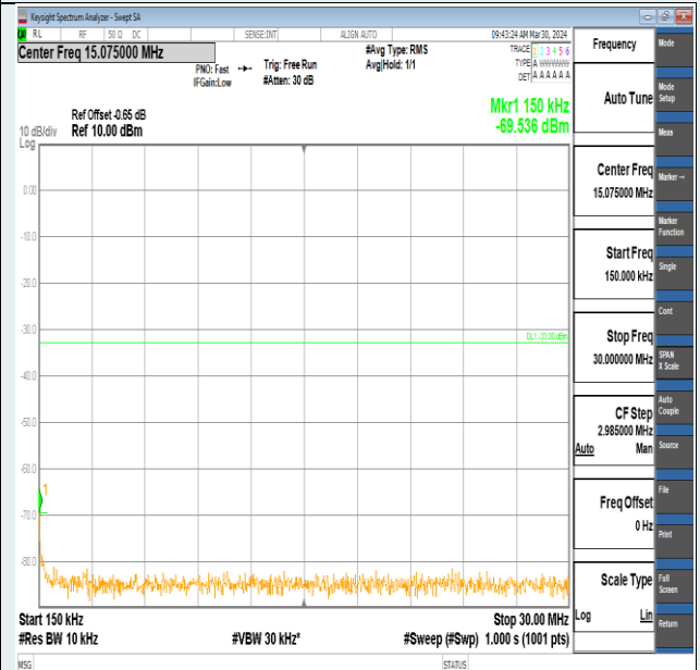
Band2-5MHz-QPSK-18900-1RB#0-0.15~30-PASS
