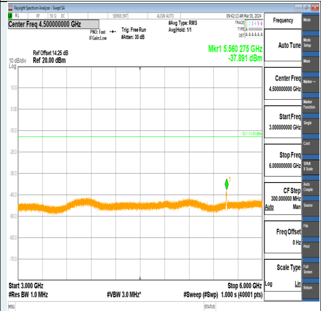
Band2-5MHz-QPSK-18625-25RB#0-3000~6000-PASS
