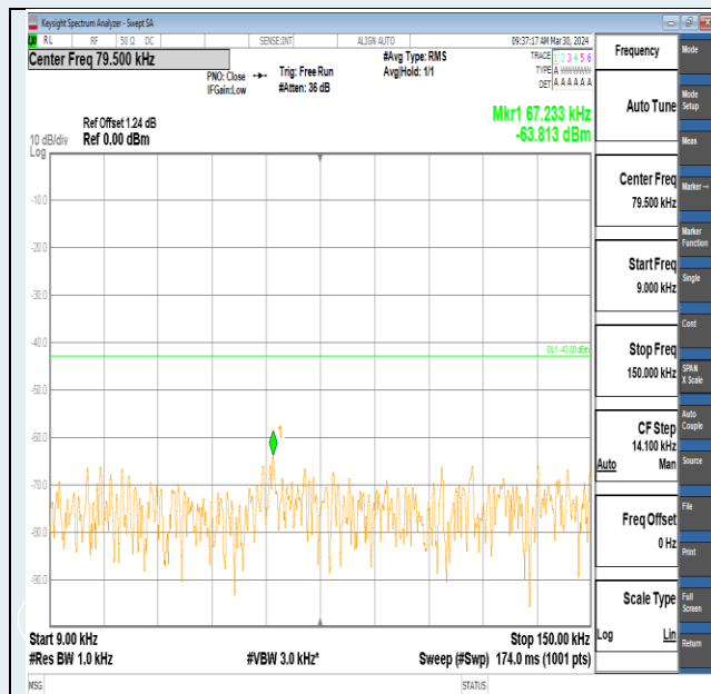
Band2-5MHz-QPSK-18625-1RB#0-0.009~0.15-PASS
