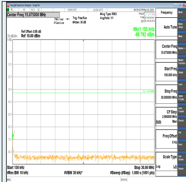
Band2-3MHz-16QAM-19185-1RB#0-0.15~30-PASS
