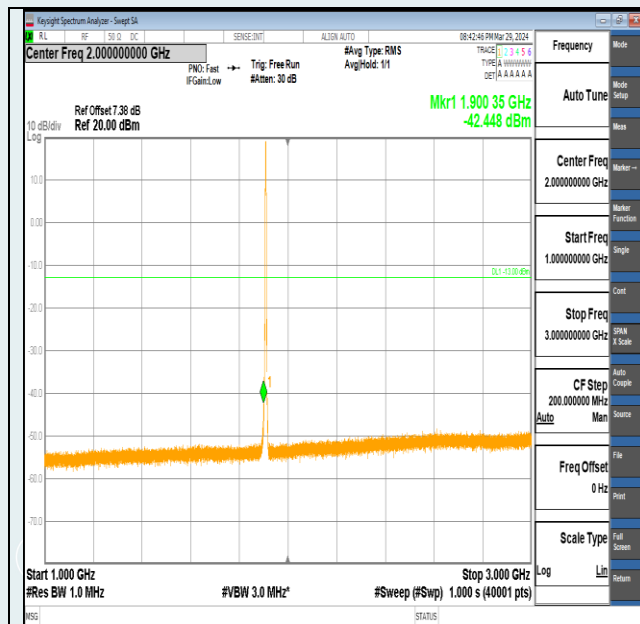
Band2-3MHz-16QAM-19185-15RB#0-1000~3000-PASS
