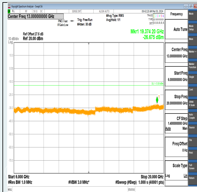
Band2-5MHz-QPSK-18625-25RB#0-6000~20000-PASS
