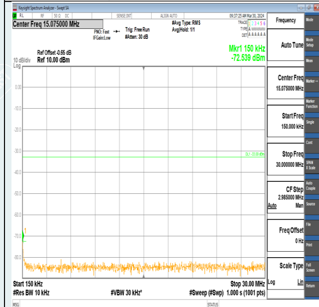
Band2-5MHz-QPSK-18625-1RB#0-0.15~30-PASS
