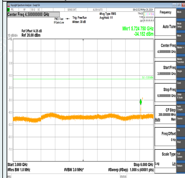
Band2-3MHz-16QAM-19185-15RB#0-3000~6000-PASS
