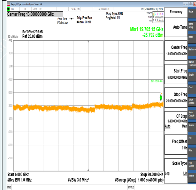
Band2-5MHz-QPSK-18625-1RB#0-6000~20000-PASS
