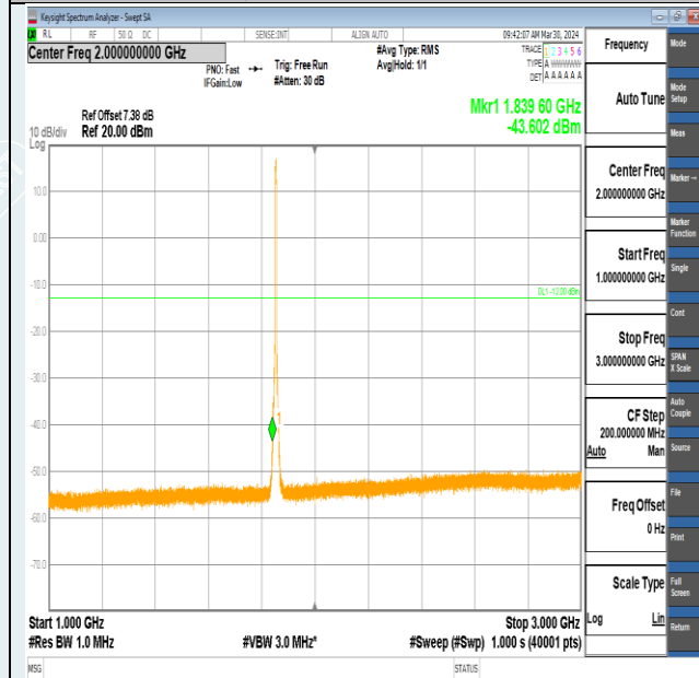
Band2-5MHz-QPSK-18625-25RB#0-1000~3000-PASS
