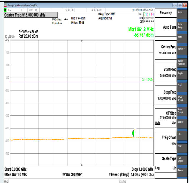
Band2-3MHz-16QAM-18900-15RB#0-30~1000-PASS
