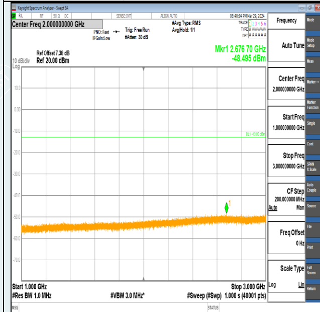
Band2-3MHz-16QAM-19185-1RB#0-1000~3000-PASS
