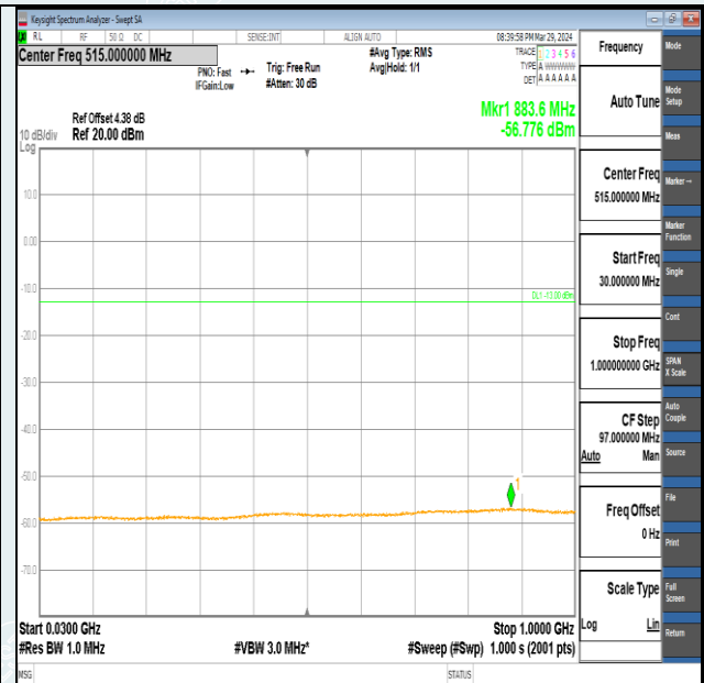
Band2-3MHz-16QAM-19185-1RB#0-30~1000-PASS
