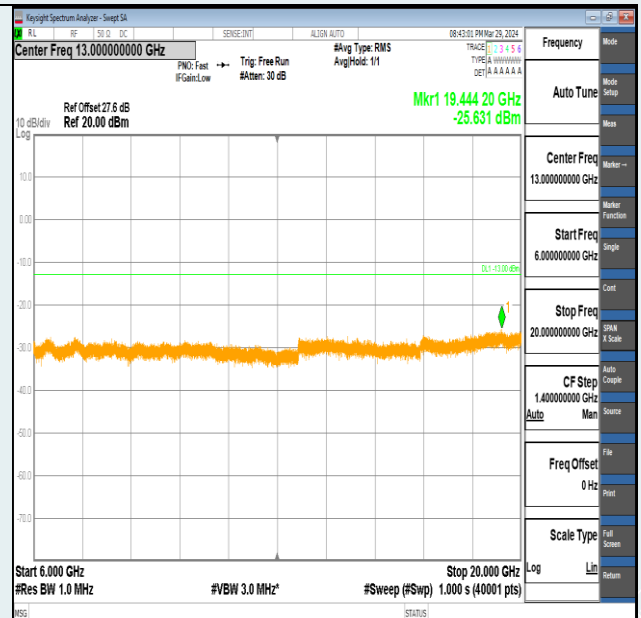
Band2-3MHz-16QAM-19185-15RB#0-6000~20000-PASS
