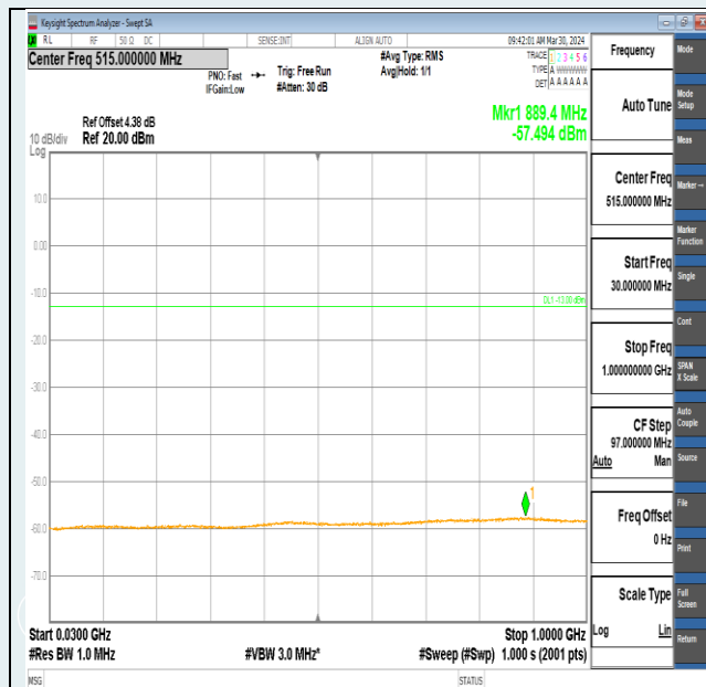
Band2-5MHz-QPSK-18625-25RB#0-30~1000-PASS
