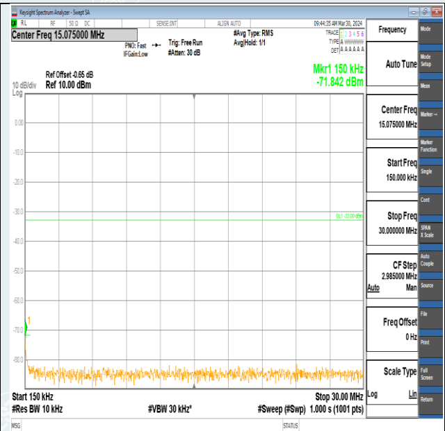
Band2-5MHz-QPSK-18900-1RB#24-0.15~30-PASS
