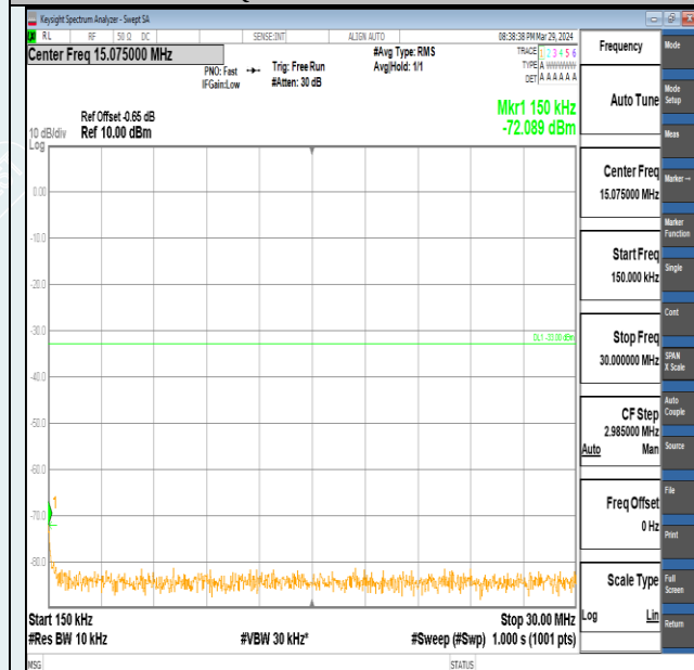
Band2-3MHz-16QAM-18900-15RB#0-0.15~30-PASS
