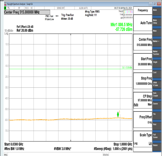
Band2-5MHz-QPSK-18625-1RB#0-30~1000-PASS
