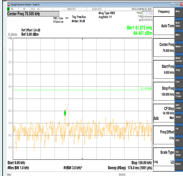
Band2-5MHz-QPSK-18900-1RB#0-0.009~0.15-PASS
