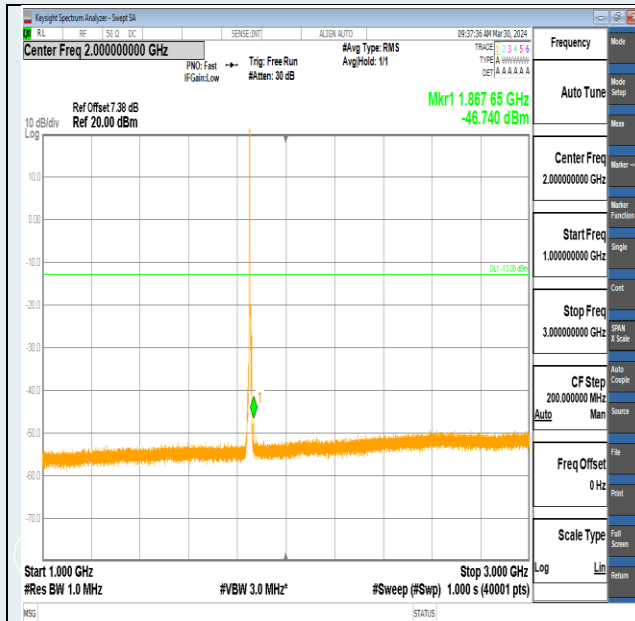
Band2-5MHz-QPSK-18625-1RB#0-1000~3000-PASS
