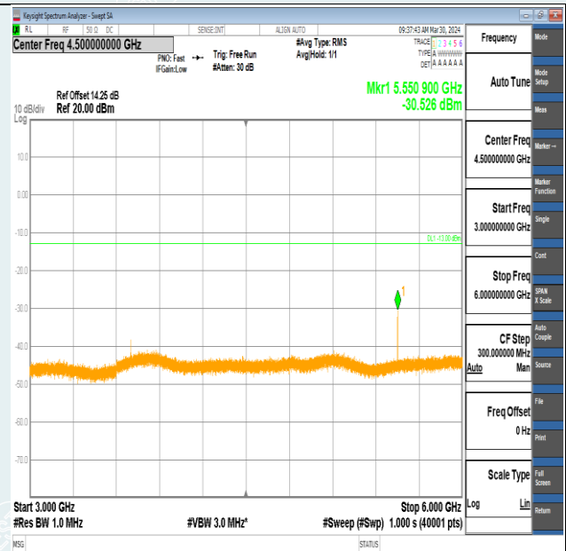
Band2-5MHz-QPSK-18625-1RB#0-3000~6000-PASS
