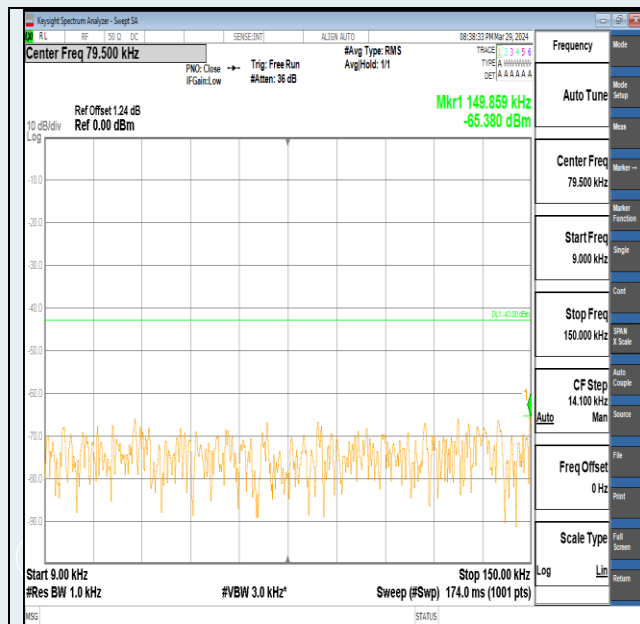
Band2-3MHz-16QAM-18900-15RB#0-0.009~0.15-PASS
