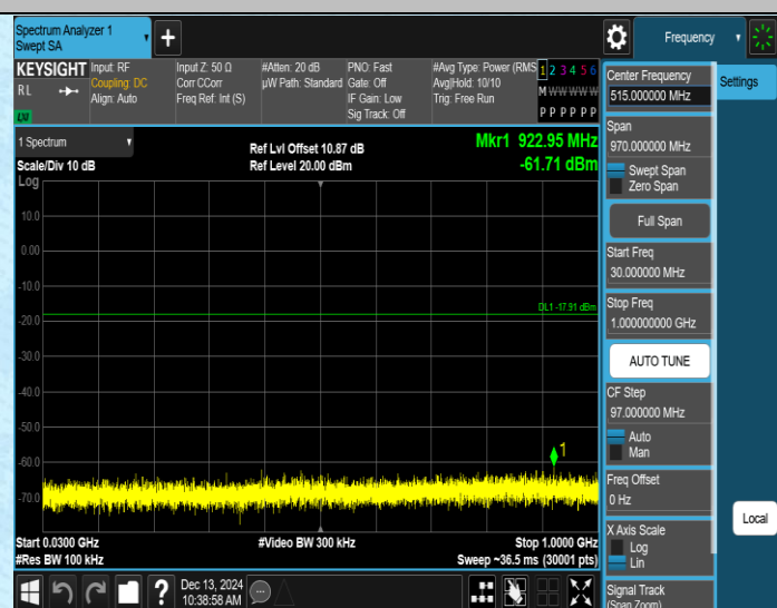
ZIGB-Ant1-2475-30~1000-PASS
