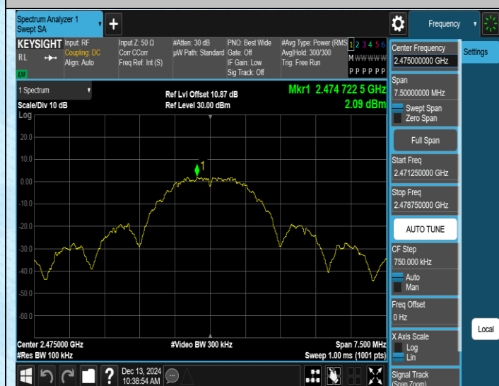
ZIGB-Ant1-2475-0~Reference-PASS
