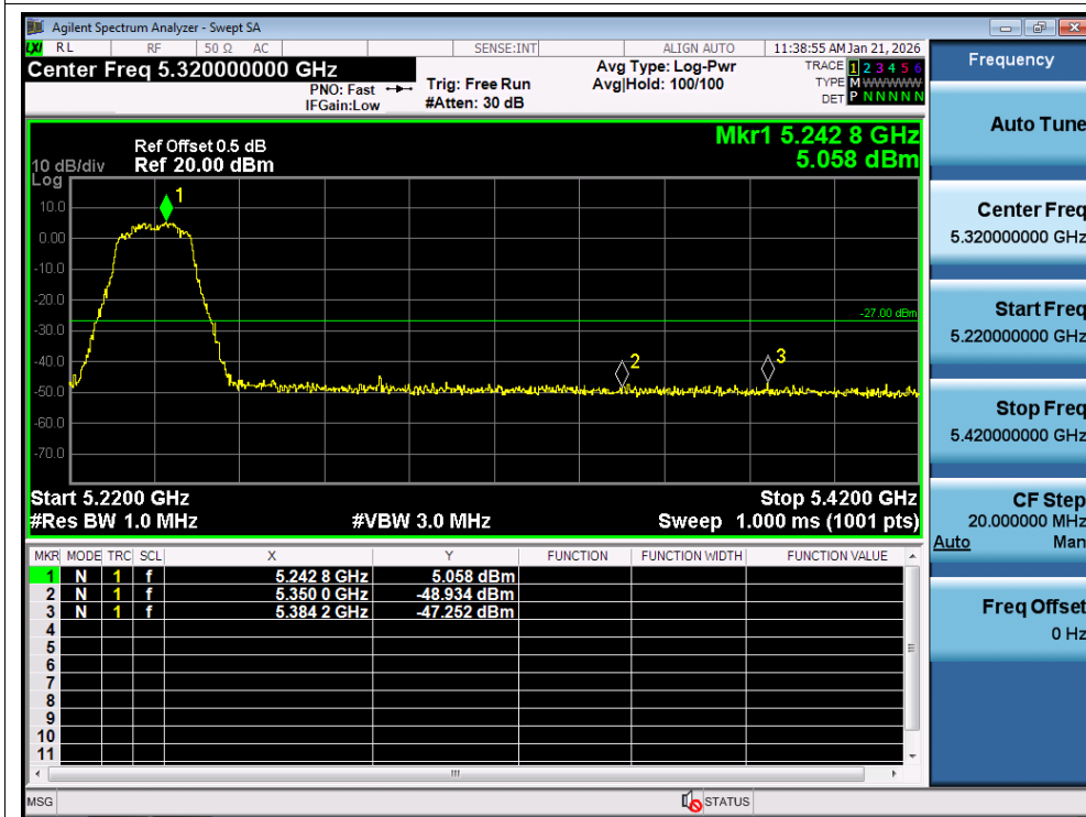
Band Edge NVNT n20 5240MHz High Ant B
