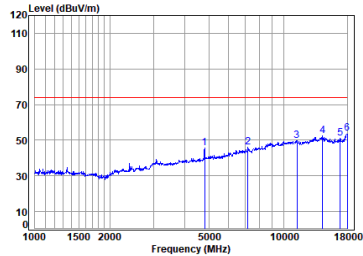
BLE_1M_TX_CH_00_Vertical-Peak
