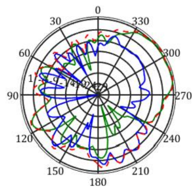
frequency=2450MHz, X-Y Plane
