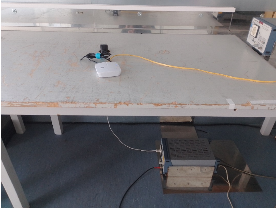
Photo 1: Conducted Emission
