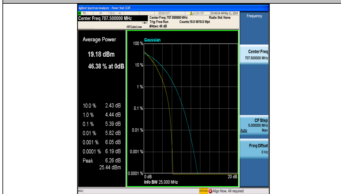
Band12-5MHz-QPSK-23095-25RB#0-PASS
