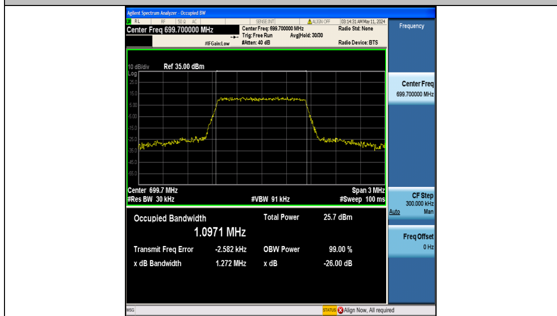
Band12-1.4MHz-16QAM-23017-6RB#0-PASS
