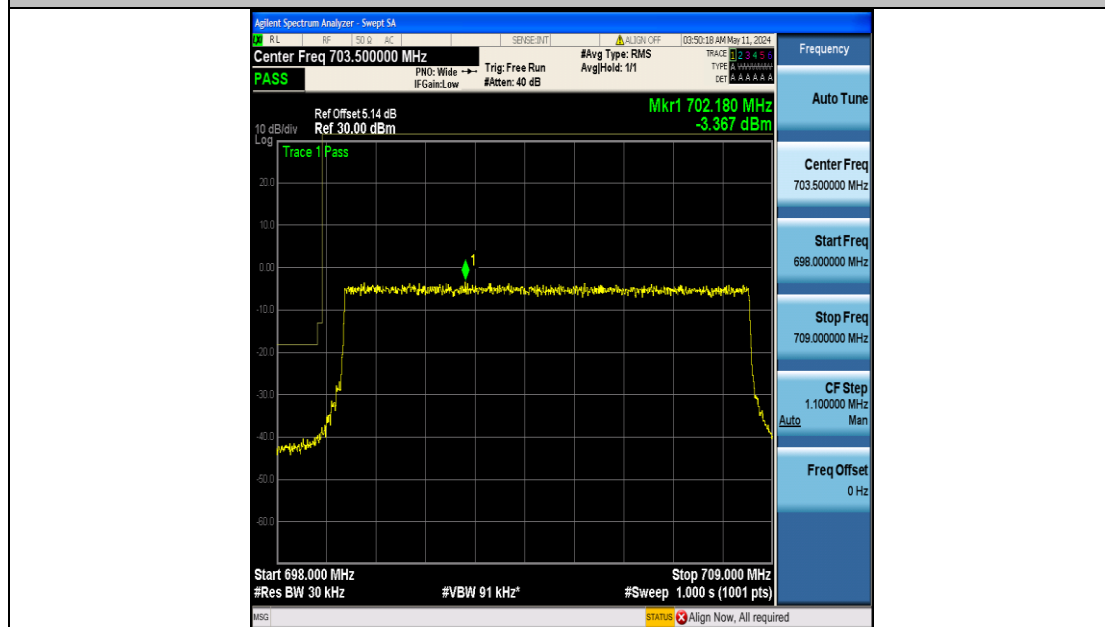
Band12_10MHz_QPSK_23060_50RB#0
