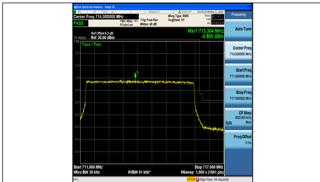
Band12_5MHz_16QAM_23155_25RB#0
