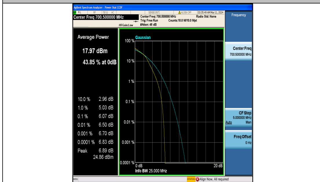
Band12-3MHz-16QAM-23025-15RB#0-PASS
