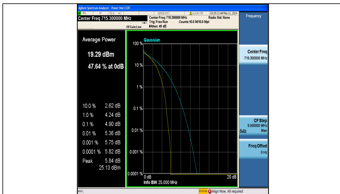
Band12-1.4MHz-QPSK-23173-6RB#0-PASS
