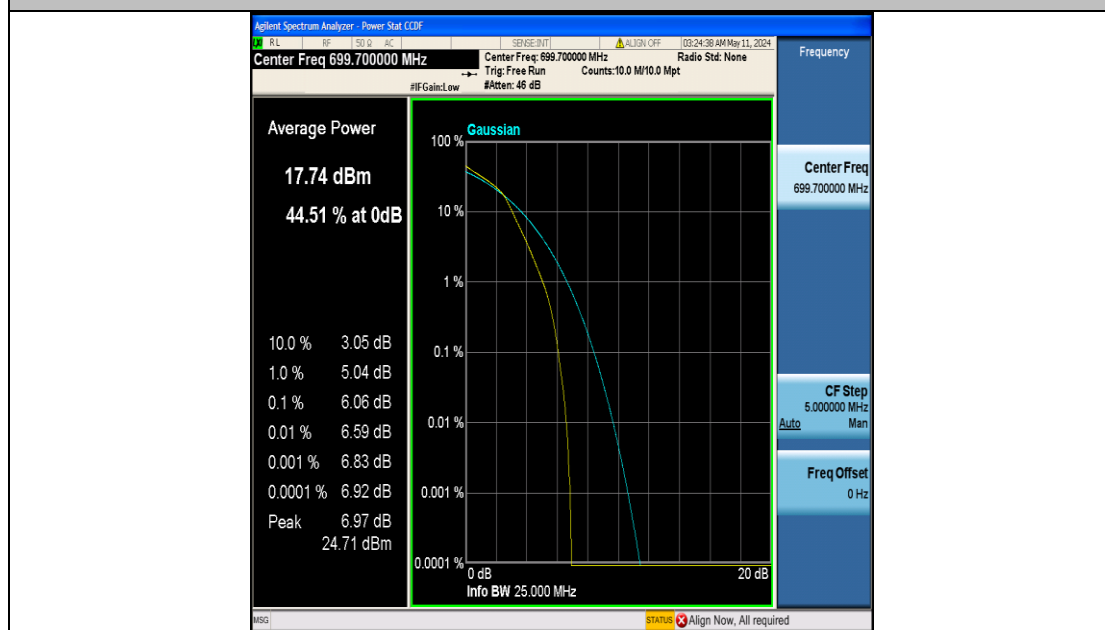
Band12-1.4MHz-16QAM-23017-6RB#0-PASS
