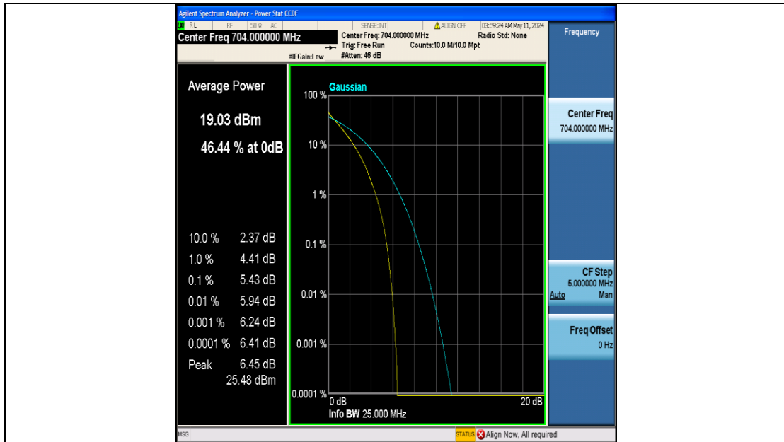
Band12-10MHz-QPSK-23060-50RB#0-PASS
