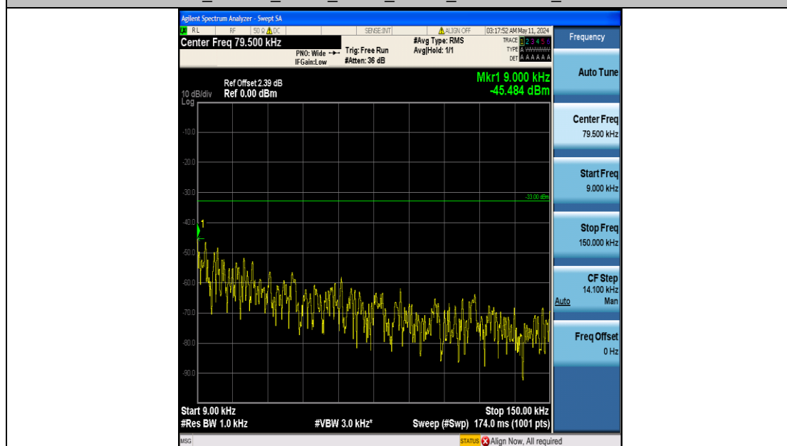
Band12_1.4MHz_QPSK_23095_6RB#0_0.009~0.15_0.009~0.15
