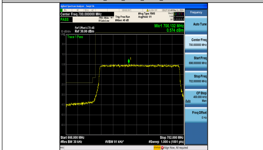
Band12_3MHz_16QAM_23025_15RB#0
