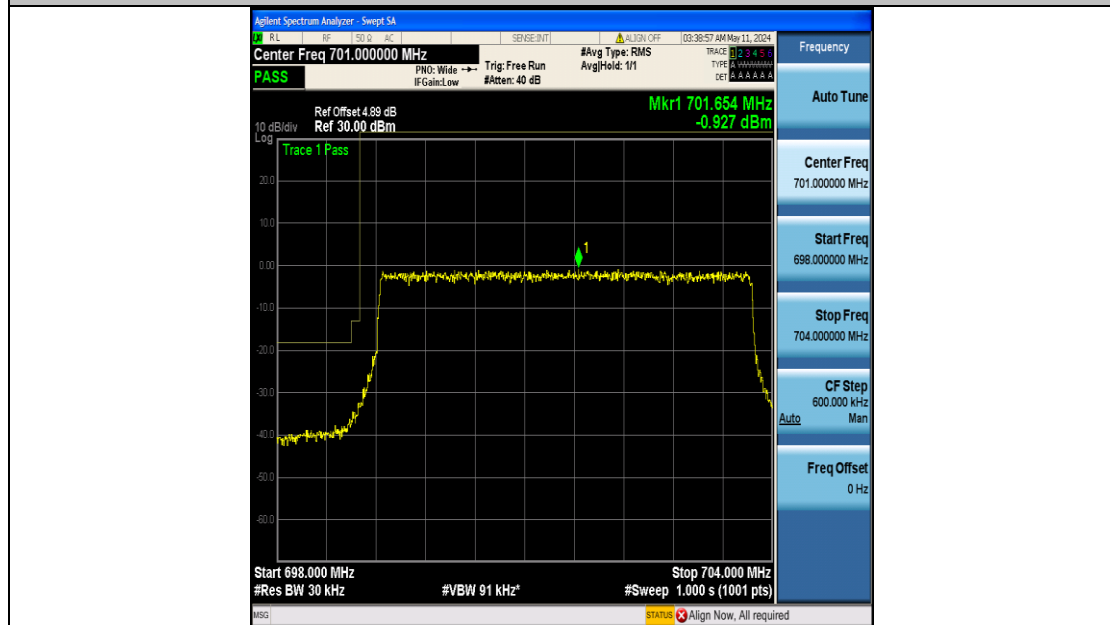
Band12_5MHz_QPSK_23035_25RB#0
