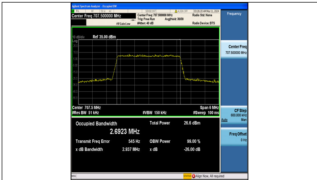
Band12-3MHz-16QAM-23095-15RB#0-PASS
