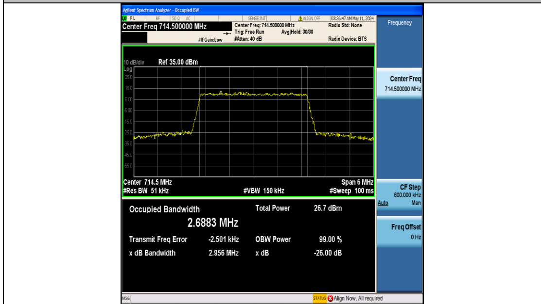
Band12-3MHz-16QAM-23165-15RB#0-PASS
