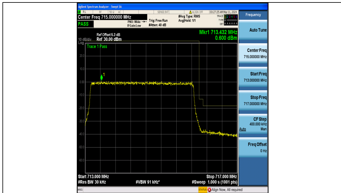
Band12_3MHz_16QAM_23165_15RB#0
