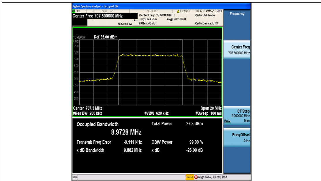
Band12-10MHz-16QAM-23095-50RB#0-PASS
