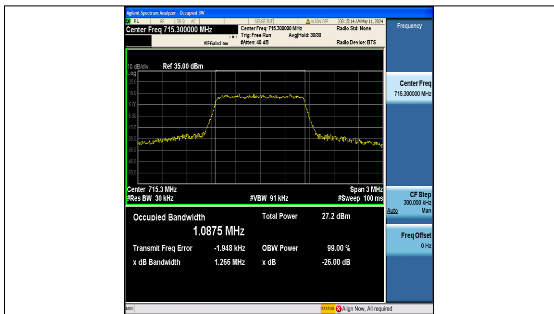
Band12-1.4MHz-QPSK-23173-6RB#0-PASS
