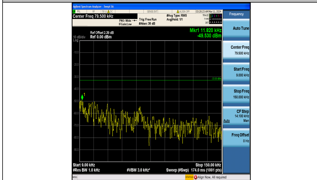
Band12_3MHz_16QAM_23025_15RB#0_0.009~0.15_0.009~0.15
