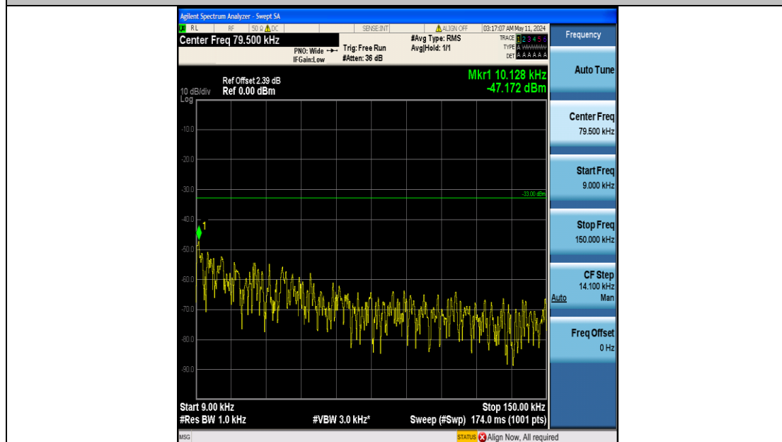
Band12_1.4MHz_16QAM_23017_6RB#0_0.009~0.15_0.009~0.15
