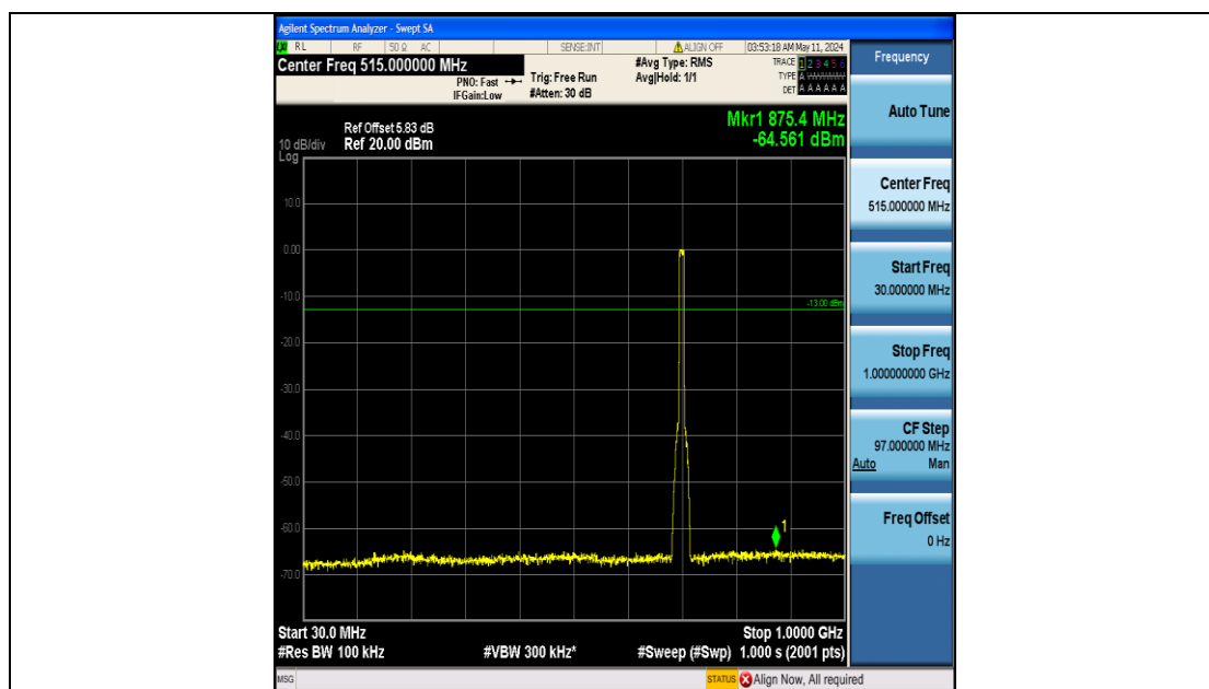
Band12_10MHz_16QAM_23095_50RB#0_30~1000_30~1000
