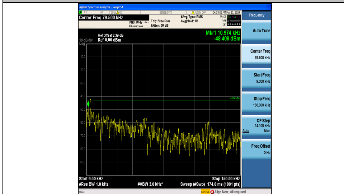
Band25_1.4MHz_QPSK_26683_6RB#0_0.009~0.15_0.009~0.15
