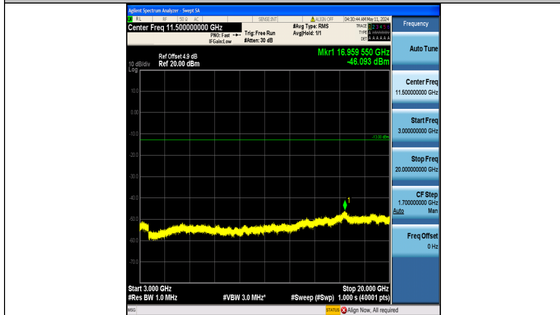
Band25_1.4MHz_QPSK_26047_6RB#0_3000~20000_3000~20000
