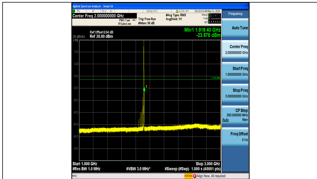
Band25_1.4MHz_QPSK_26683_6RB#0_1000~3000_1000~3000
