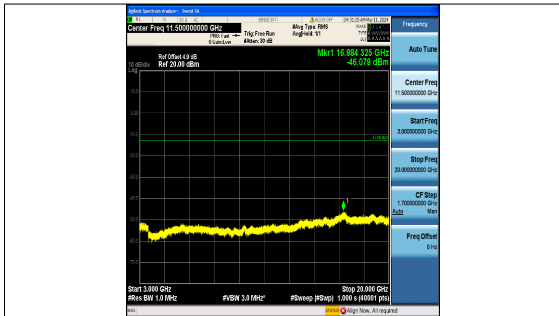
Band25_1.4MHz_16QAM_26047_6RB#0_3000~20000_3000~20000
