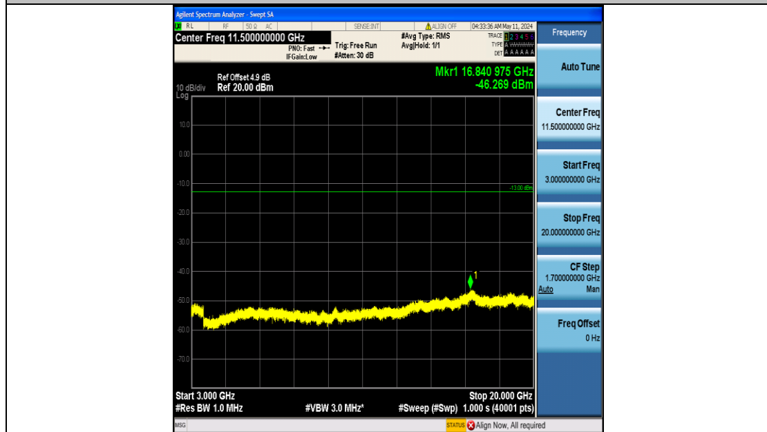
Band25_1.4MHz_QPSK_26683_6RB#0_3000~20000_3000~20000
