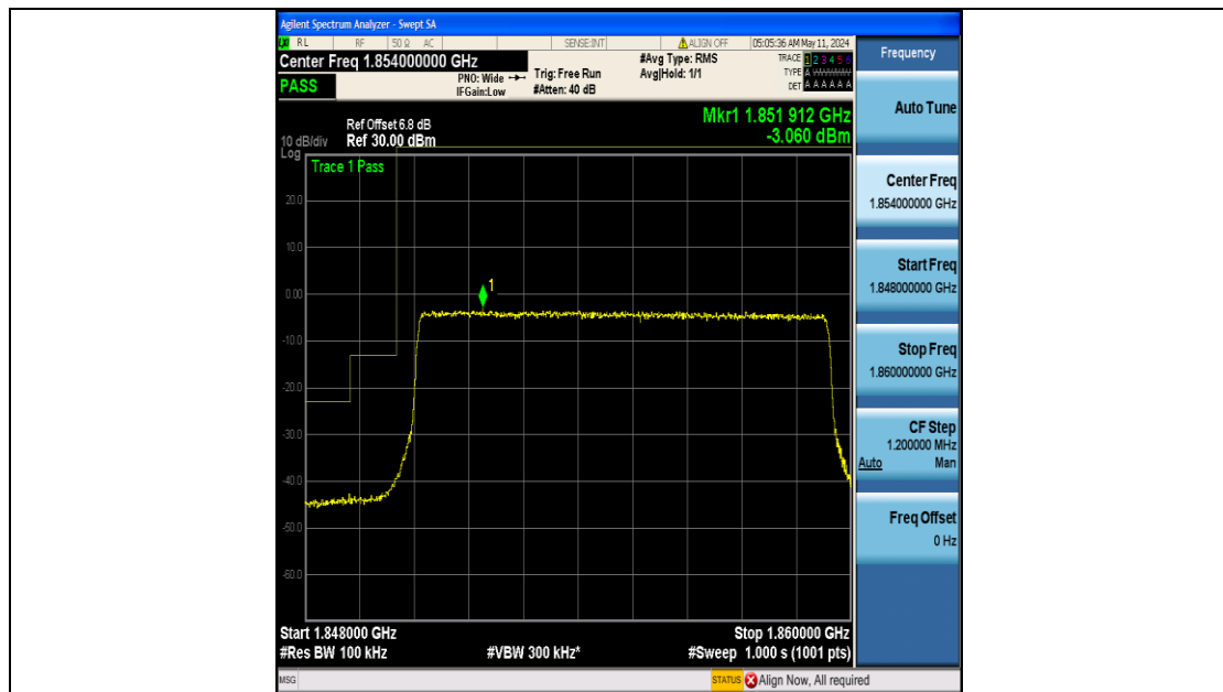
Band25_10MHz_16QAM_26090_50RB#0
