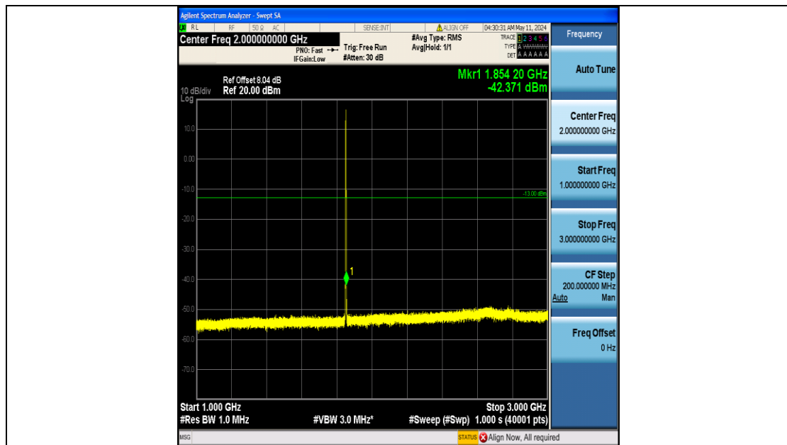
Band25_1.4MHz_QPSK_26047_6RB#0_1000~3000_1000~3000
