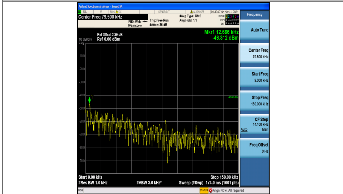
Band25_1.4MHz_16QAM_26365_6RB#0_0.009~0.15_0.009~0.15
