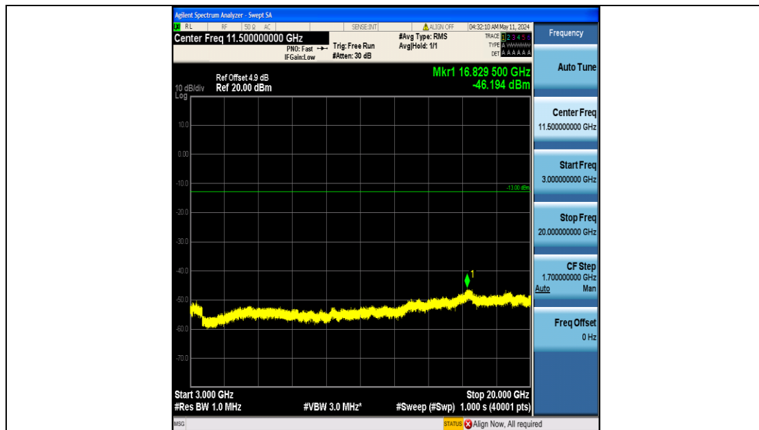
Band25_1.4MHz_QPSK_26365_6RB#0_3000~20000_3000~20000
