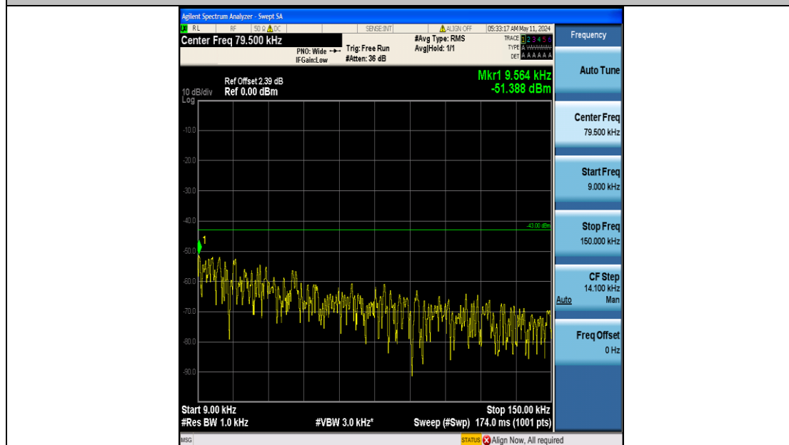
Band25_20MHz_QPSK_26590_100RB#0_0.009~0.15_0.009~0.15
