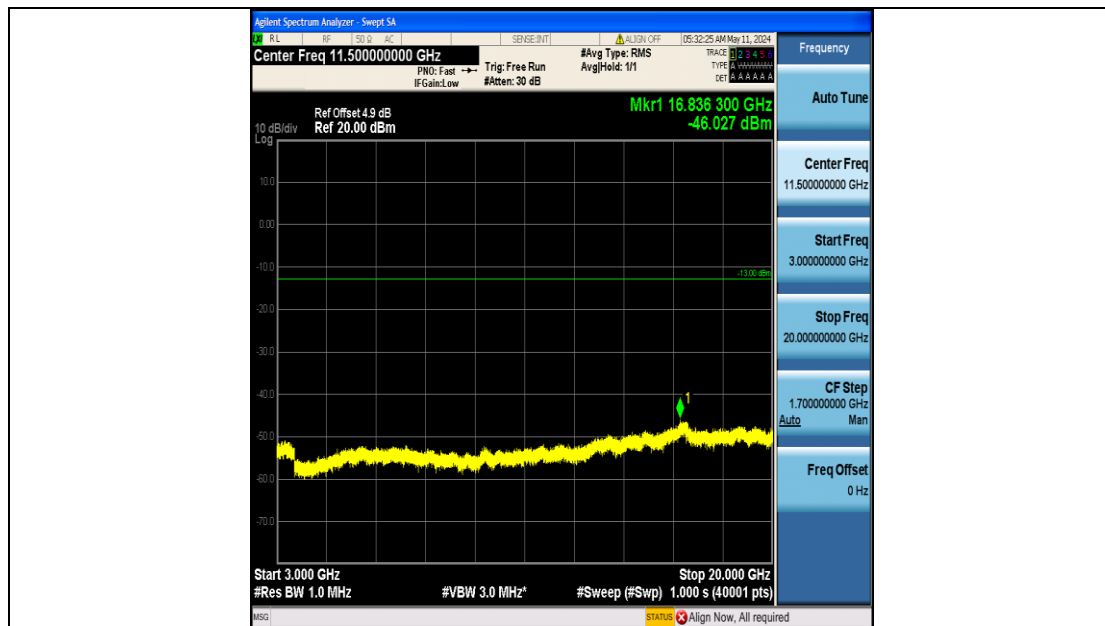
Band25_20MHz_QPSK_26365_100RB#0_3000~20000_3000~20000
