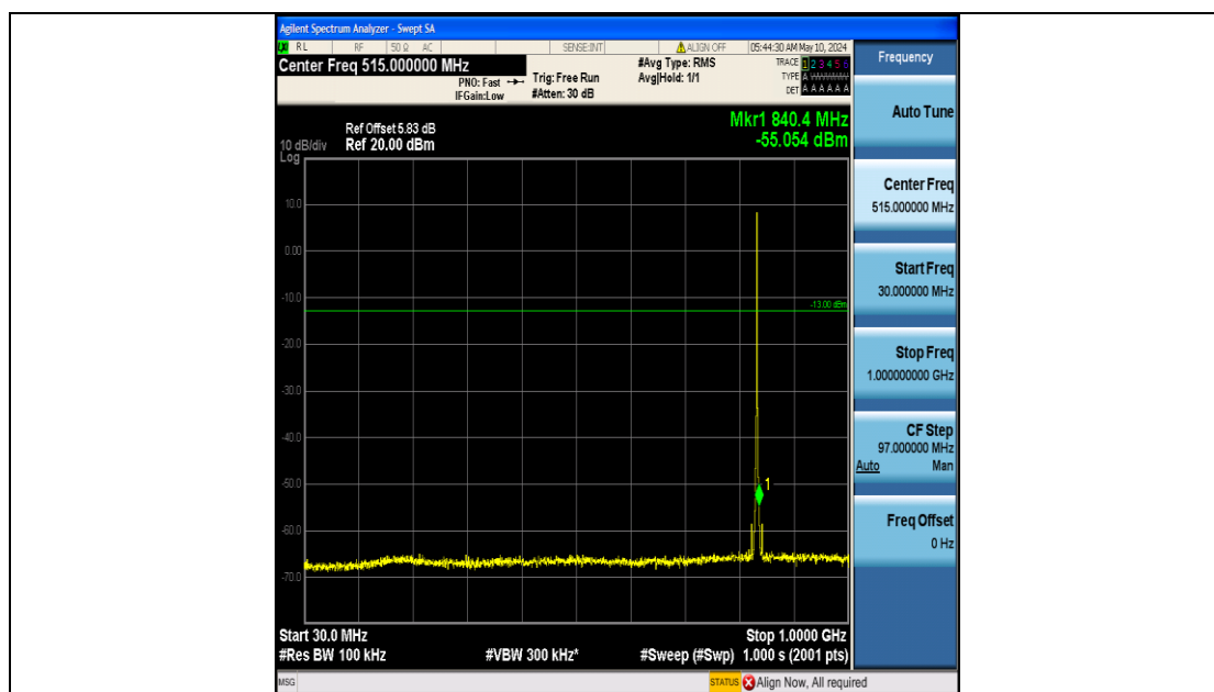
Band26_1.4MHz_16QAM_26915_6RB#0_30~1000_30~1000
