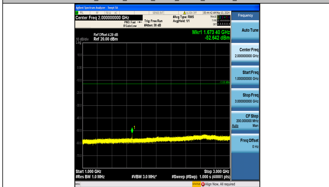
Band26_1.4MHz_16QAM_26915_6RB#0_1000~3000_1000~3000
