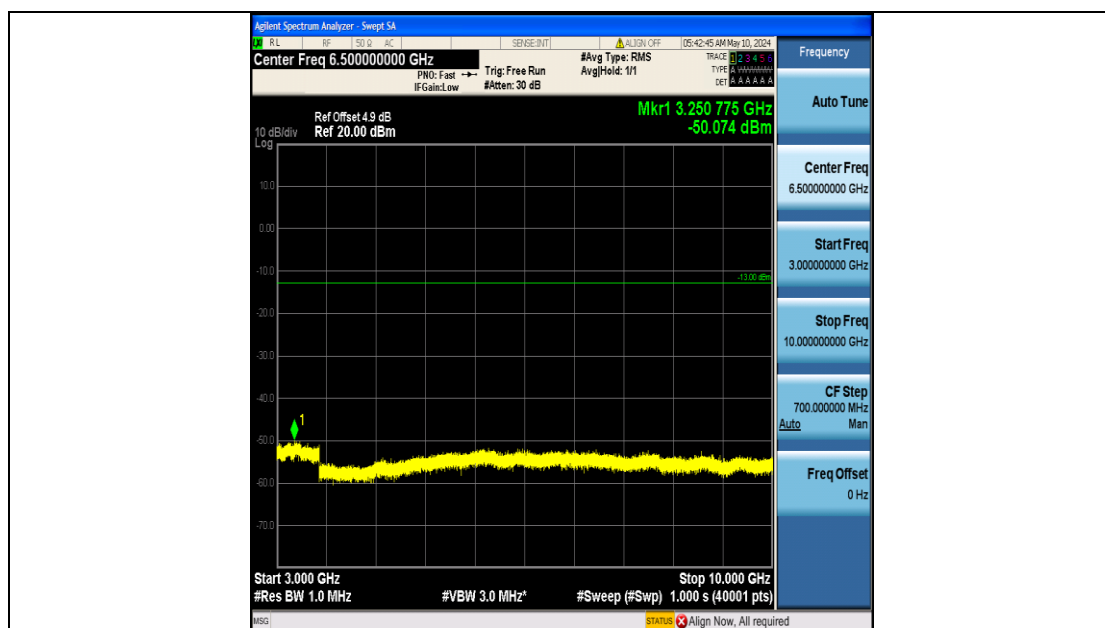
Band26_1.4MHz_QPSK_26797_6RB#0_3000~10000_3000~10000
