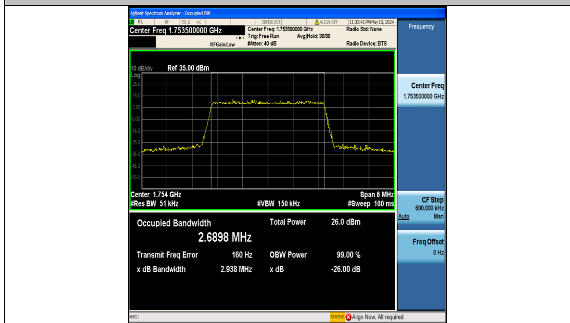
Band4-3MHz-16QAM-20385-15RB#0-PASS
