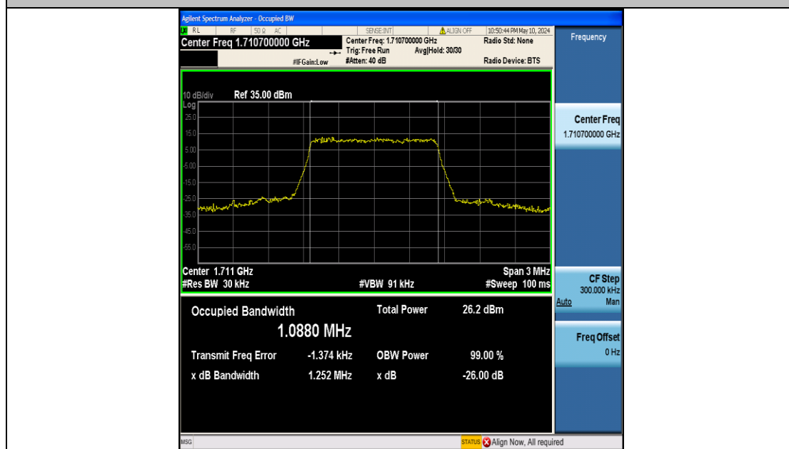
Band4-1.4MHz-16QAM-19957-6RB#0-PASS
