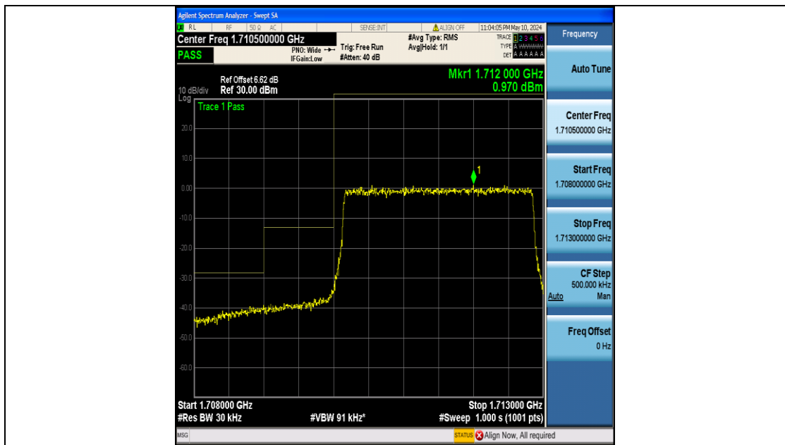
Band4_3MHz_16QAM_19965_15RB#0
