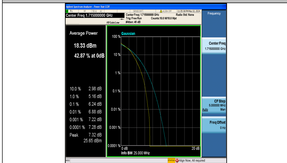
Band4-10MHz-16QAM-20000-50RB#0-PASS
