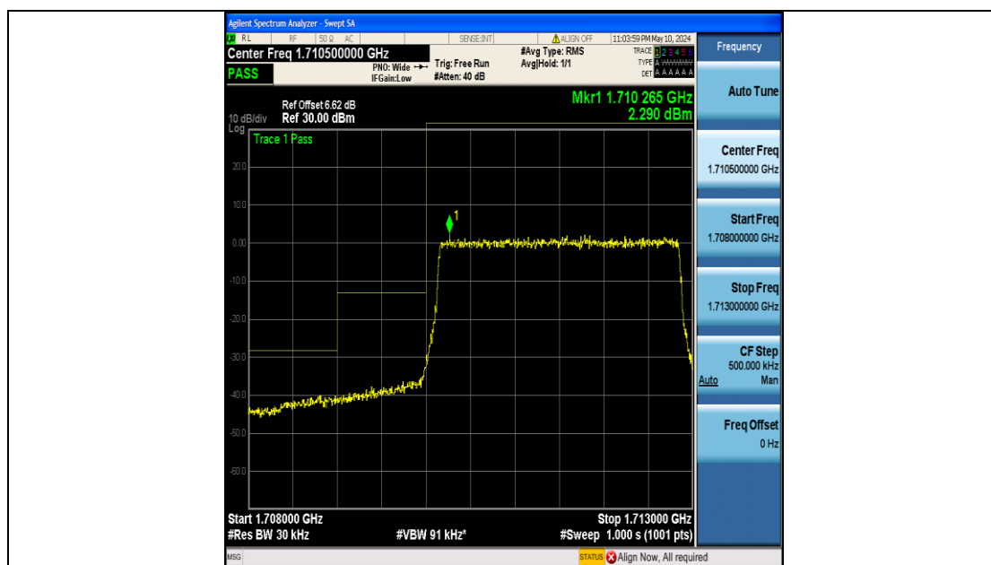
Band4_3MHz_QPSK_19965_15RB#0
