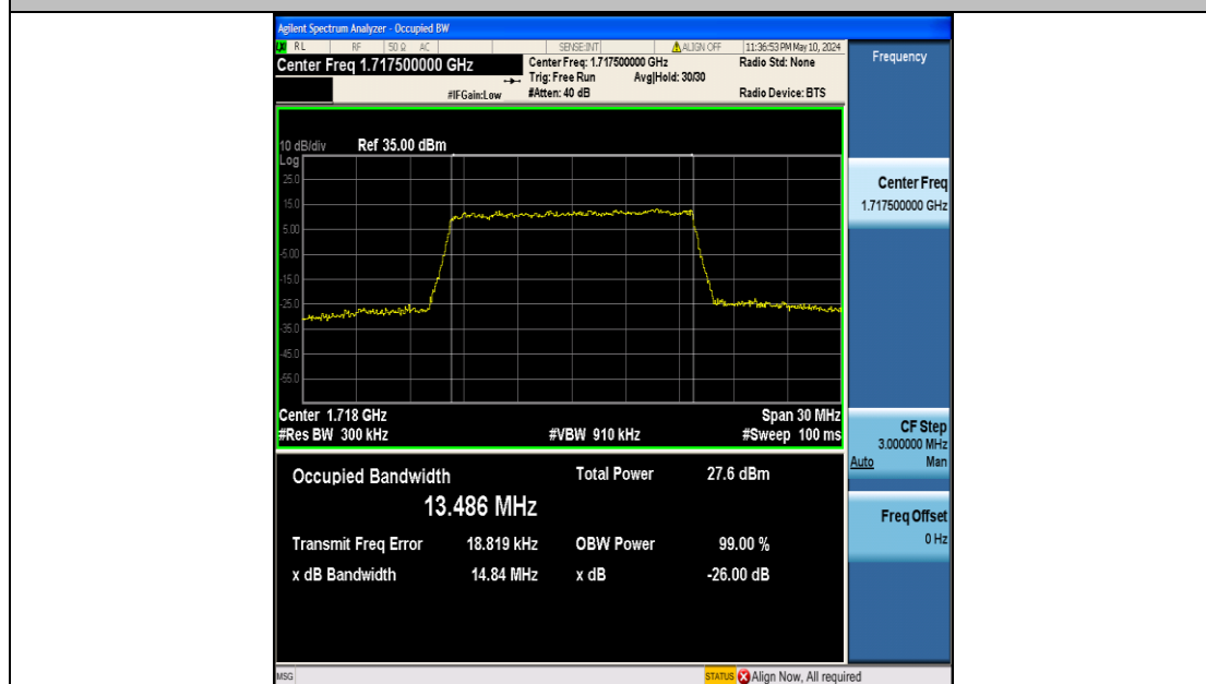
Band4-15MHz-16QAM-20025-75RB#0-PASS
