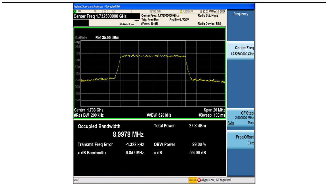
Band4-10MHz-16QAM-20175-50RB#0-PASS
