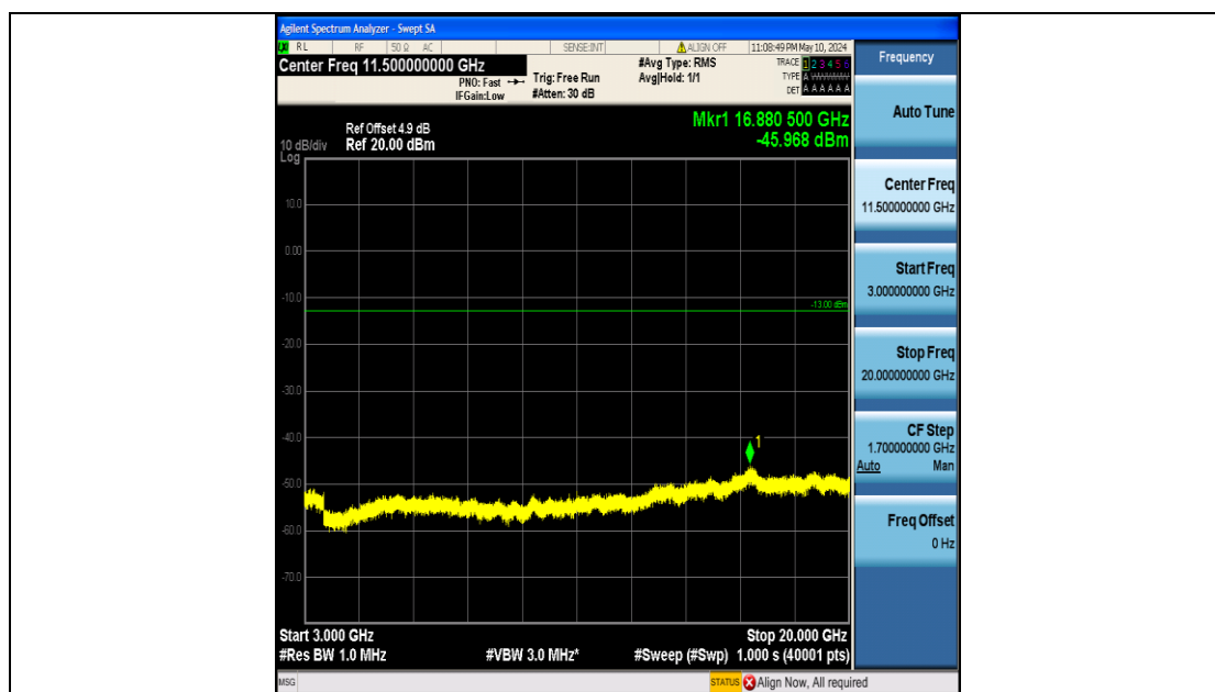
Band4_3MHz_16QAM_20385_15RB#0_3000~20000_3000~20000
