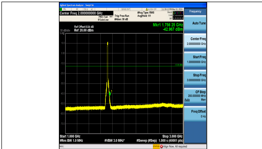
Band4_15MHz_QPSK_20025_75RB#0_1000~3000_1000~3000
