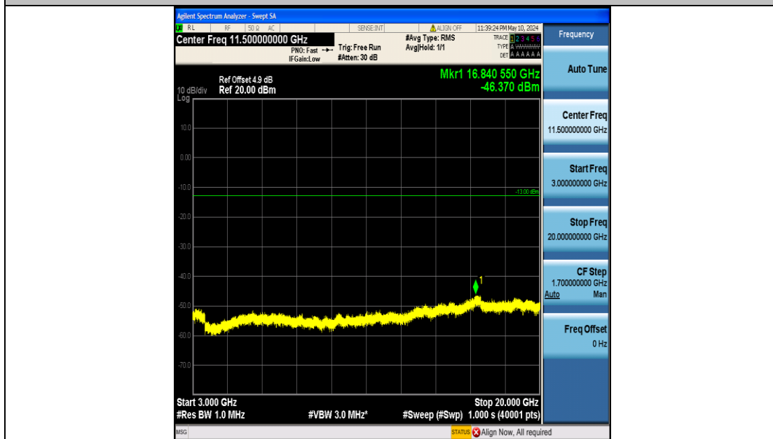
Band4_15MHz_QPSK_20025_75RB#0_3000~20000_3000~20000
