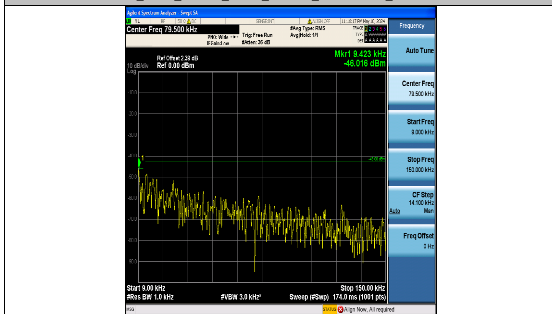
Band4_5MHz_QPSK_19975_25RB#0_0.009~0.15_0.009~0.15
