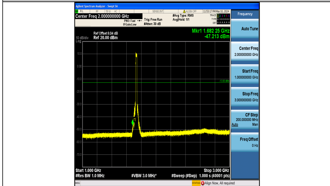
Band4_20MHz_QPSK_20175_100RB#0_1000~3000_1000~3000
