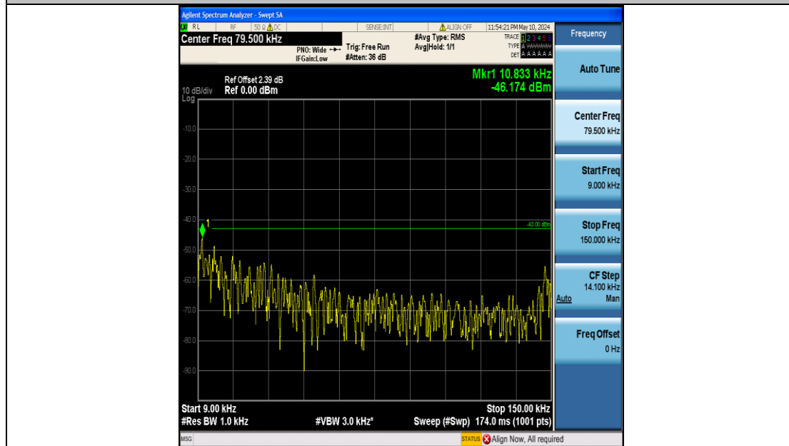
Band4_20MHz_QPSK_20300_100RB#0_0.009~0.15_0.009~0.15
