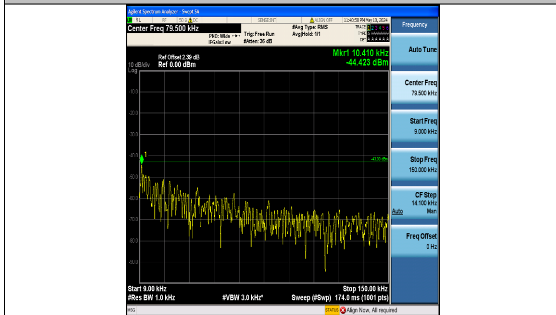
Band4_15MHz_16QAM_20175_75RB#0_0.009~0.15_0.009~0.15
