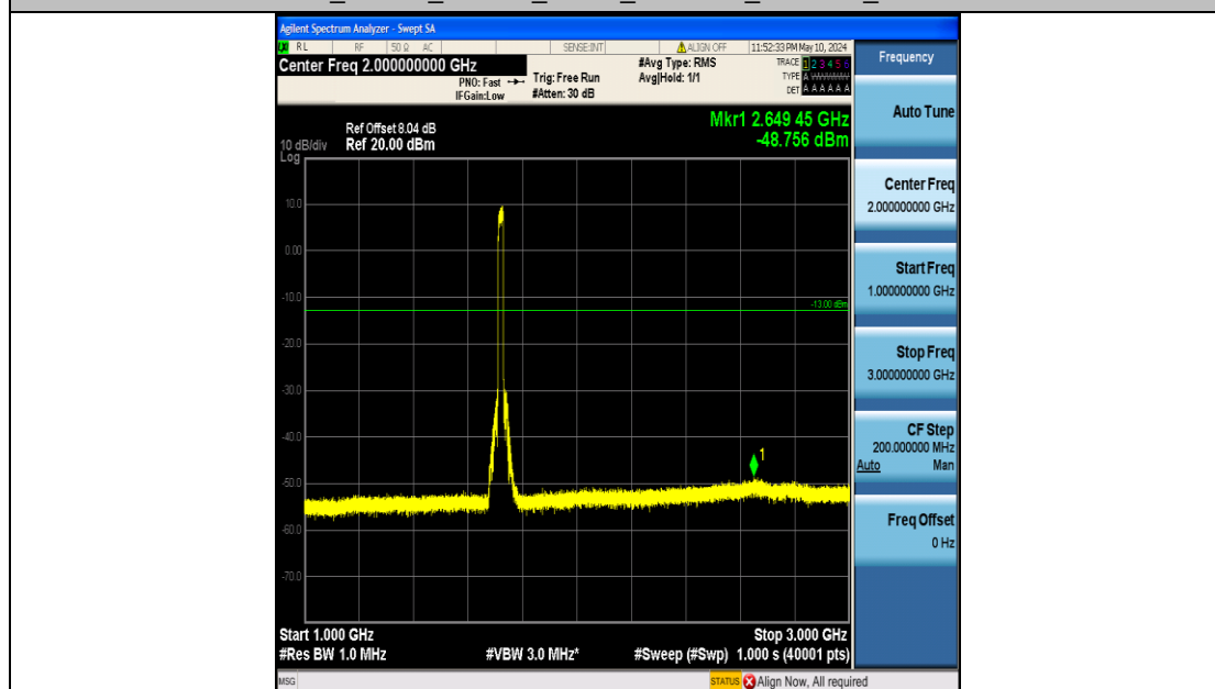
Band4_20MHz_16QAM_20050_100RB#0_1000~3000_1000~3000
