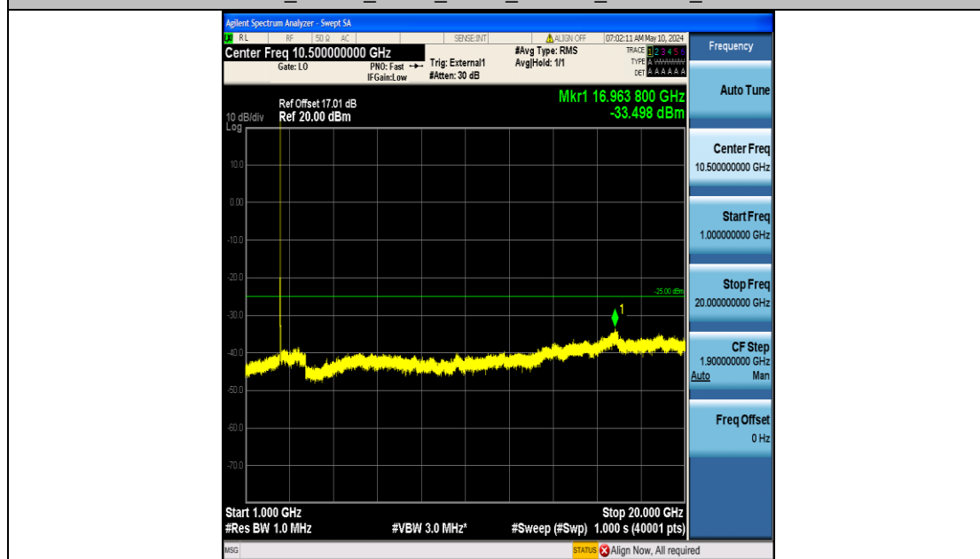
Band41_10MHz_QPSK_39700_50RB#0_1000~20000_1000~20000
