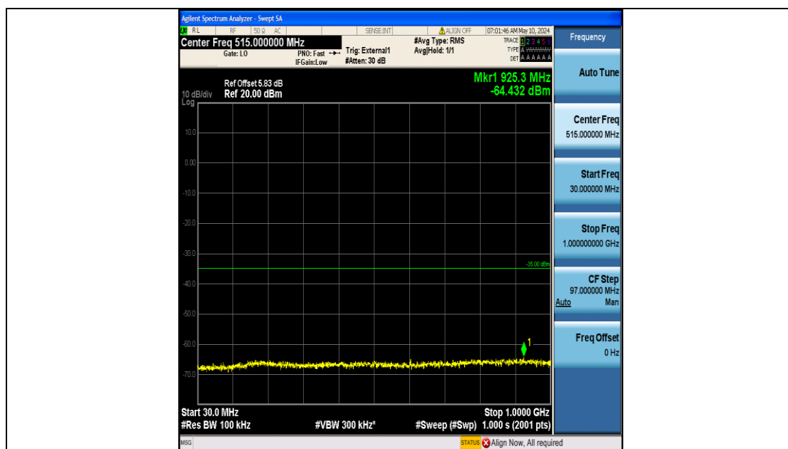
Band41_10MHz_QPSK_39700_50RB#0_30~1000_30~1000
