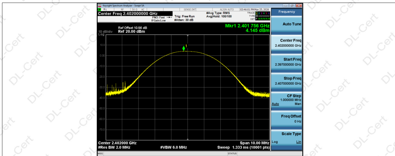
Peak Power NVNT 1-DH5 2402MHz Ant1
