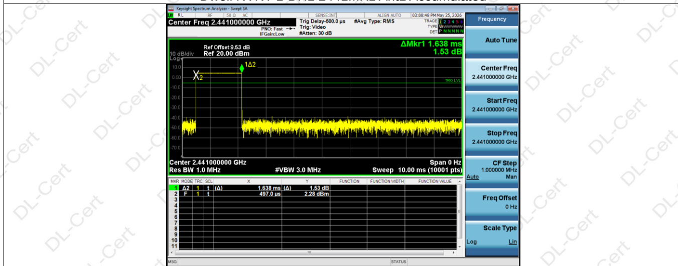
Dwell NVNT 1-DH3 2441MHz Ant1 One Burst
