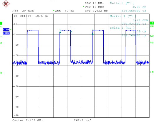
Modulation Type: GFSK(2Mbps)
