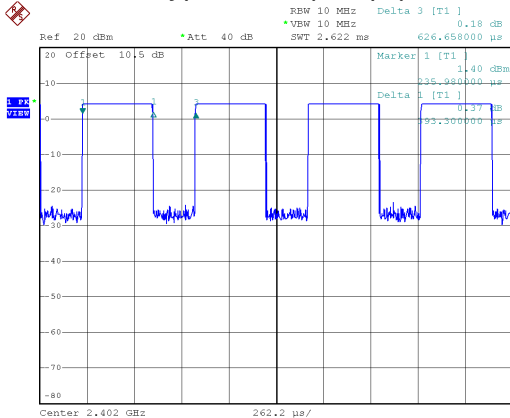
Modulation Type: GFSK(1Mbps)
