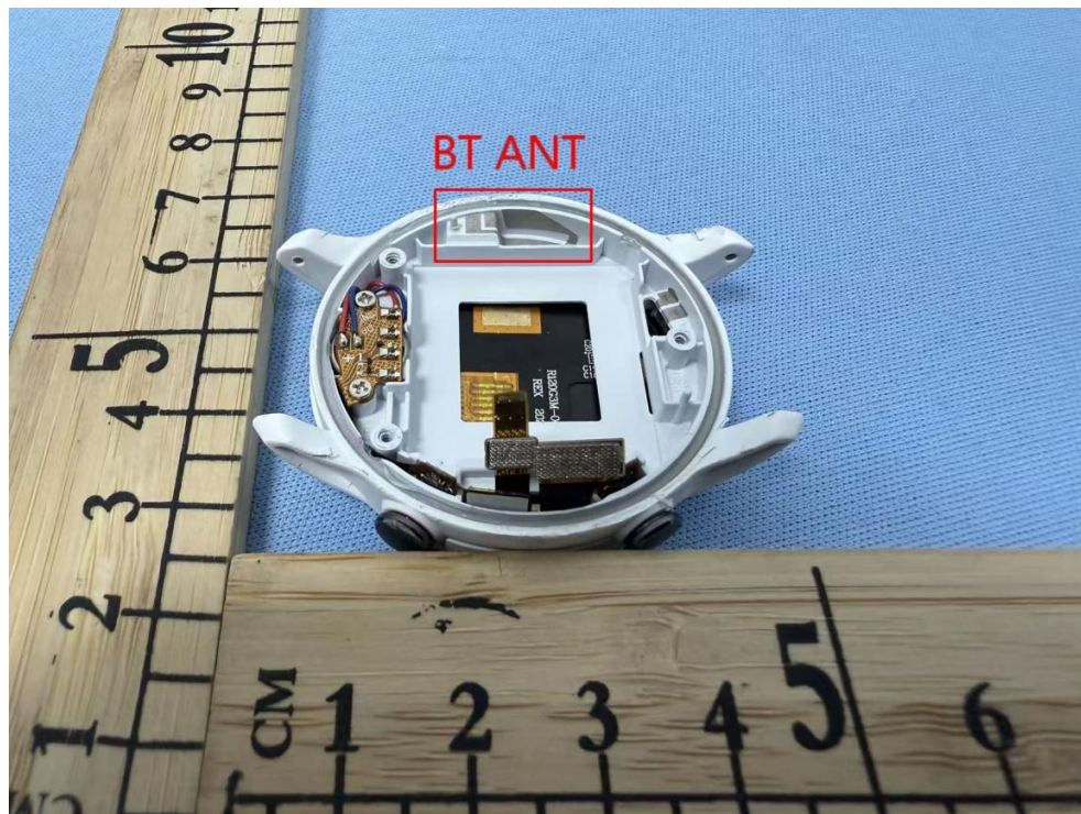
Antenna structure
