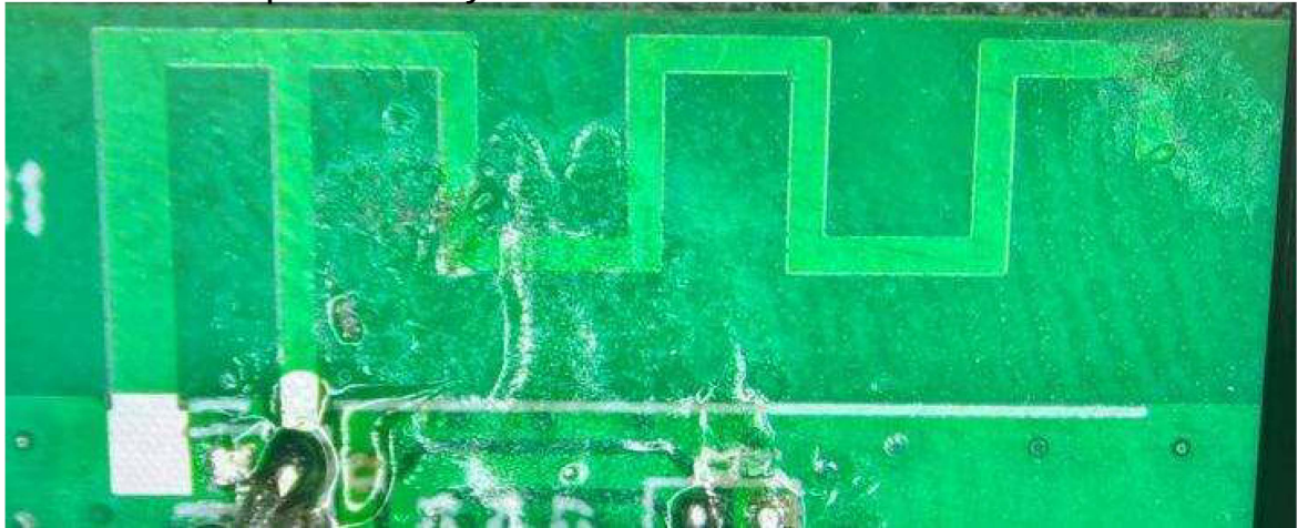
Antenna Sample and Physical Dimensions
