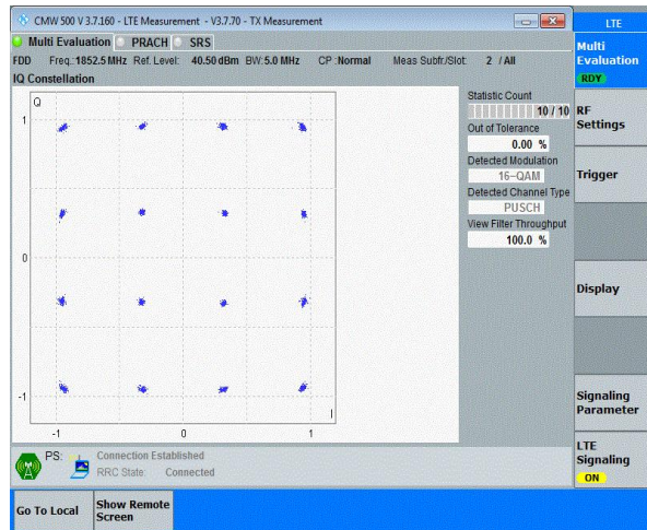
Band2-5MHz-16QAM-18900-25RB#0
