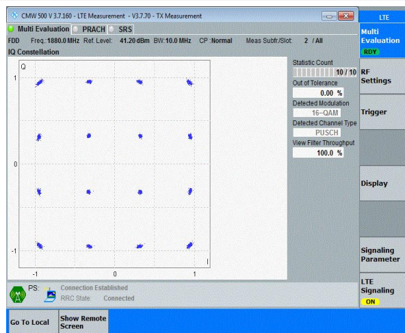
Band2-10MHz-16QAM-19150-50RB#0
