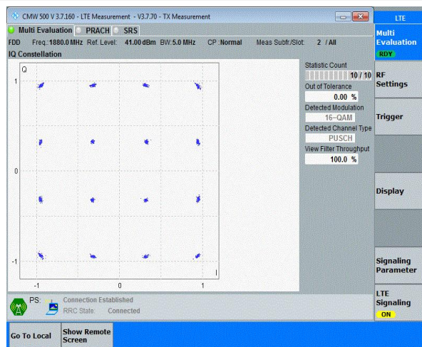
Band2-5MHz-16QAM-19175-25RB#0
