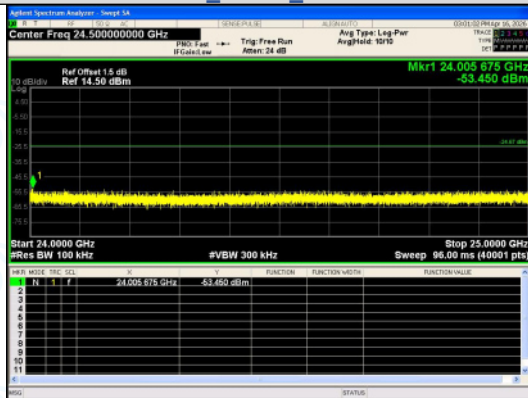
24000.0 MHz - 25000.0 MHz 8DPSK_3-DH5_Channel 0
