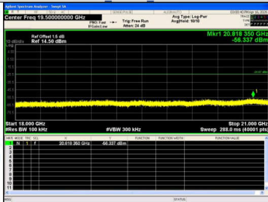
18000.0 MHz - 21000.0 MHz 8DPSK_3-DH5_Channel 0
