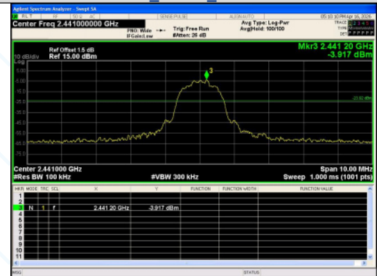
Out Of Band Emission 8DPSK_3-DH5_Channel 39
