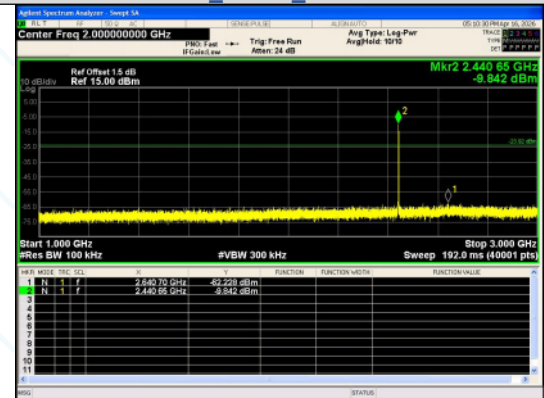
1000.0 MHz - 3000.0 MHz 8DPSK_3-DH5_Channel 39
