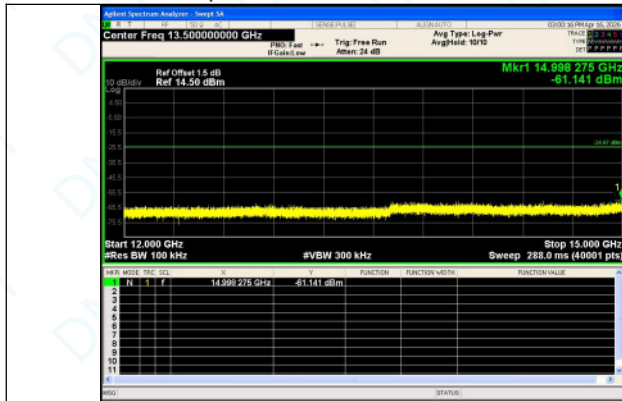
12000.0 MHz - 15000.0 MHz 8DPSK_3-DH5_Channel 0
