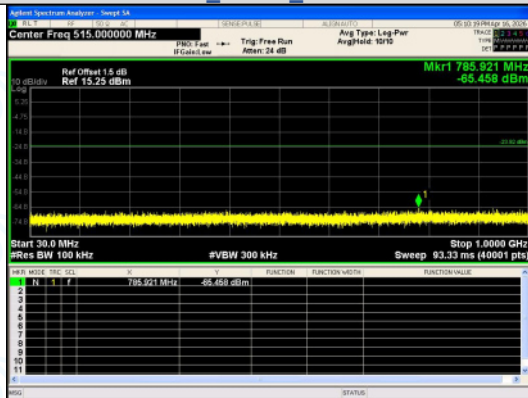
30.0 MHz - 1000.0 MHz 8DPSK_3-DH5_Channel 39
