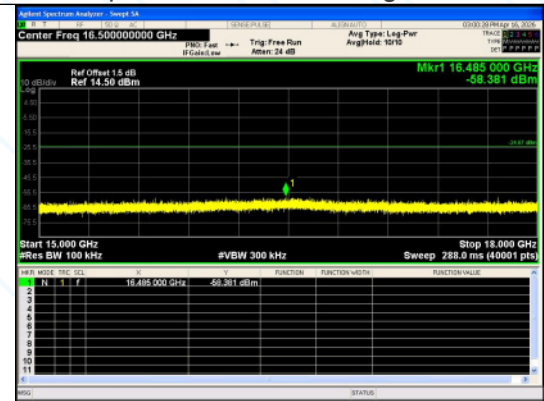
15000.0 MHz - 18000.0 MHz 8DPSK_3-DH5_Channel 0
