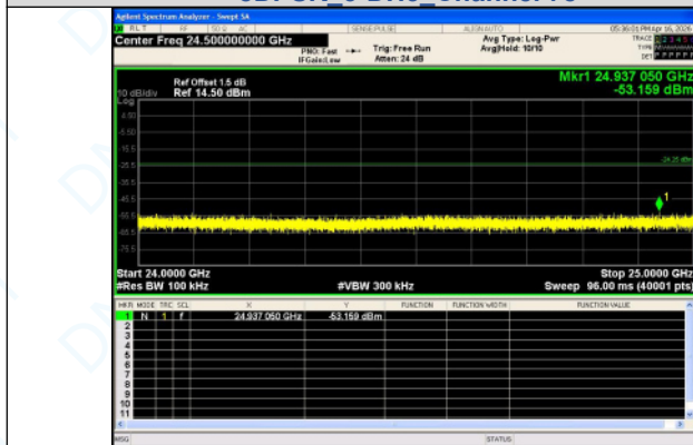
24000.0 MHz - 25000.0 MHz 8DPSK 3-DH5 Channel 78
