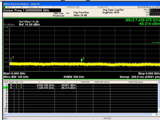
6000.0 MHz - 9000.0 MHz 8DPSK 3-DH5 Channel 78
