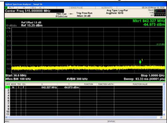
30.0 MHz - 1000.0 MHz 8DPSK 3-DH5 Channel 78
