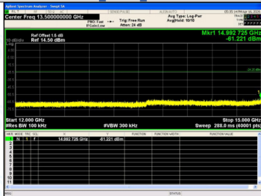
12000.0 MHz - 15000.0 MHz 8DPSK 3-DH5 Channel 78
