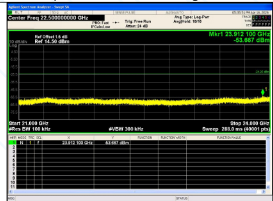
21000.0 MHz - 24000.0 MHz 8DPSK 3-DH5 Channel 78
