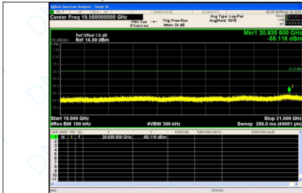
18000.0 MHz - 21000.0 MHz 8DPSK 3-DH5 Channel 78
