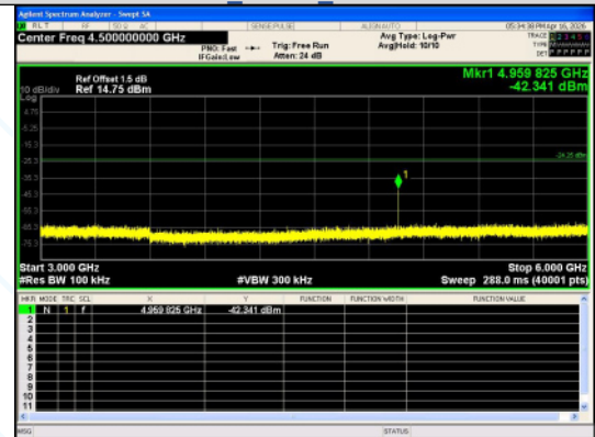
3000.0 MHz - 6000.0 MHz 8DPSK 3-DH5 Channel 78
