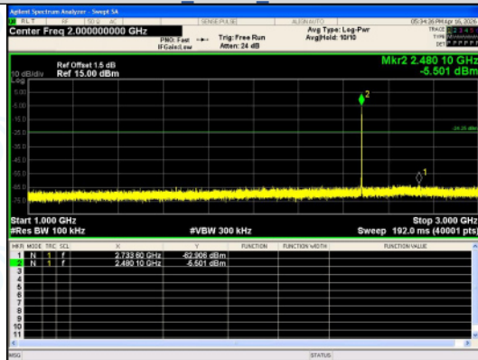
1000.0 MHz - 3000.0 MHz 8DPSK 3-DH5 Channel 78
