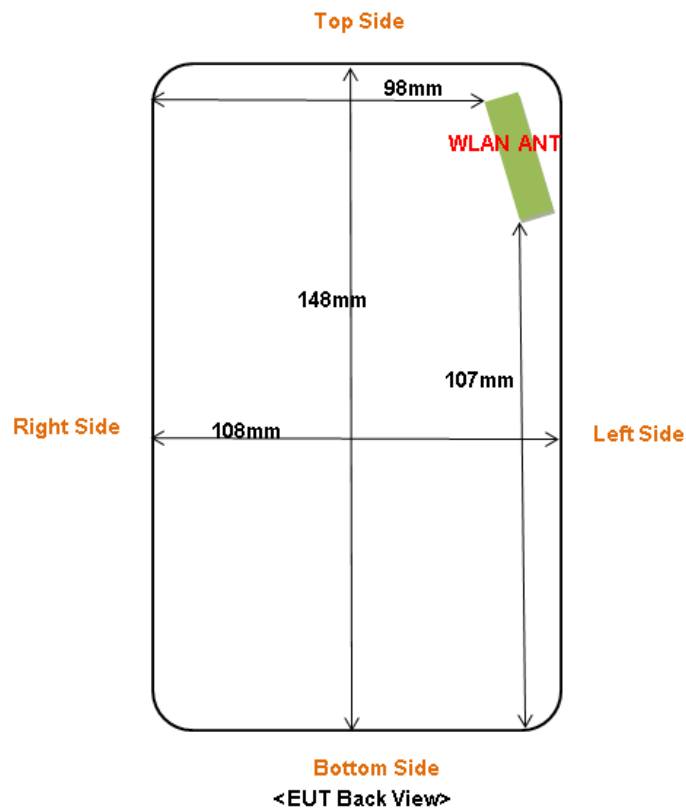
Fig 7.2 Block Diagram for EUT Antenna Position
