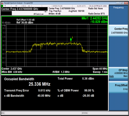
11AX20SISO-Ant1-2437
