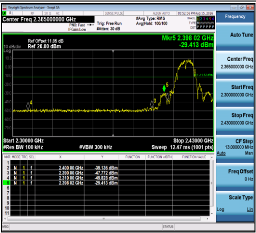
11B-Ant1-2412-PASS
