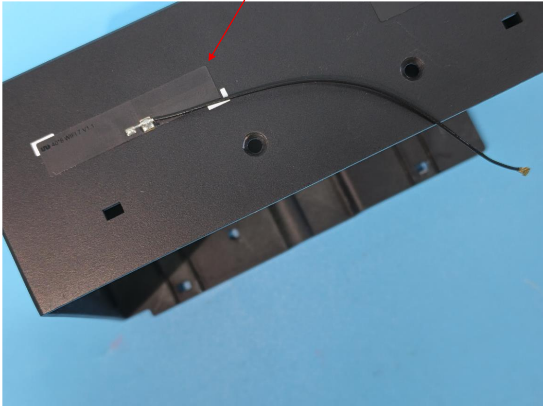
Wi-Fi Chain 1 Antenna
