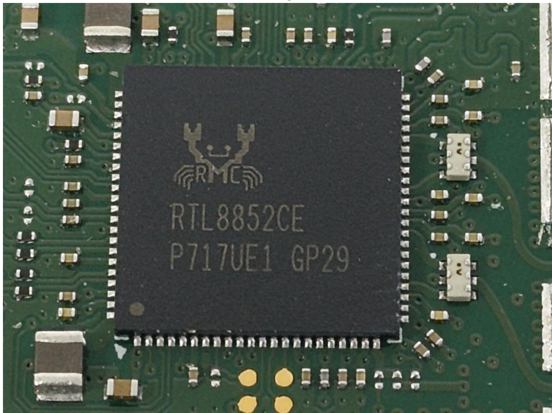
RF Chipset
