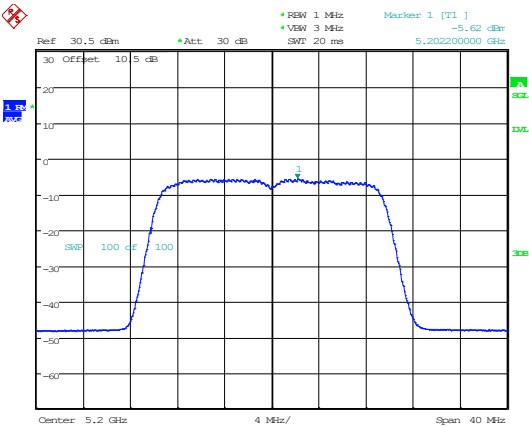
802.11ax20_5200MHz_RU_Full_Chain 1
