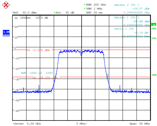
802.11a_5240MHz_Chain 0
