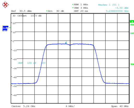
802.11a_5240MHz_Chain 1
