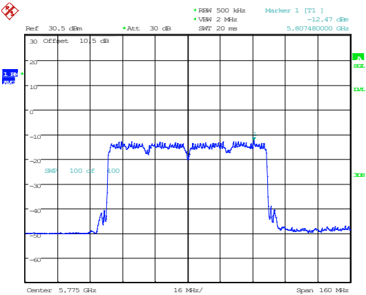
802.11ax80_5775MHz_RU_Full_Chain 0
