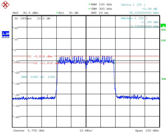
802.11ax40_5755MHz_RU_Full_Chain 0
