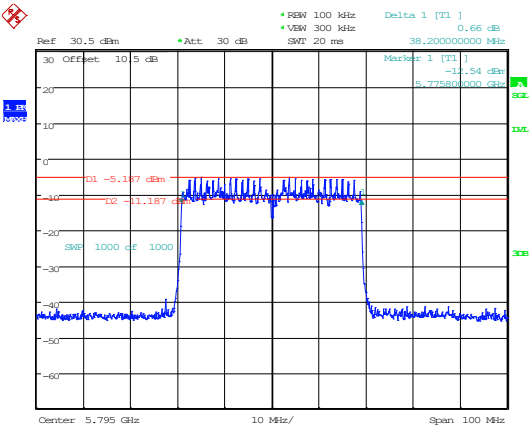
802.11ax40_5795MHz_RU_Full_Chain 0
