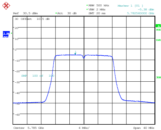
802.11a_5785MHz_Chain 1
