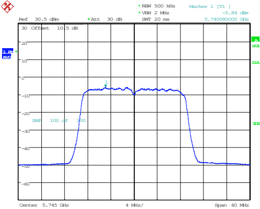
802.11ac20_5745MHz_Chain 1
