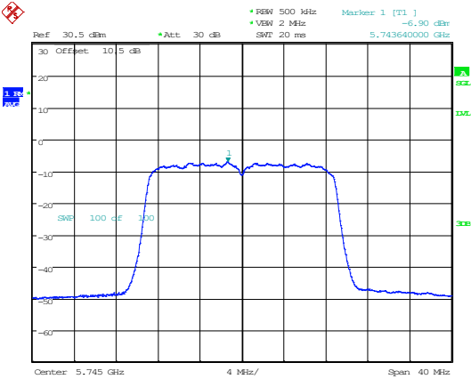
802.11ac20_5745MHz_Chain 0
