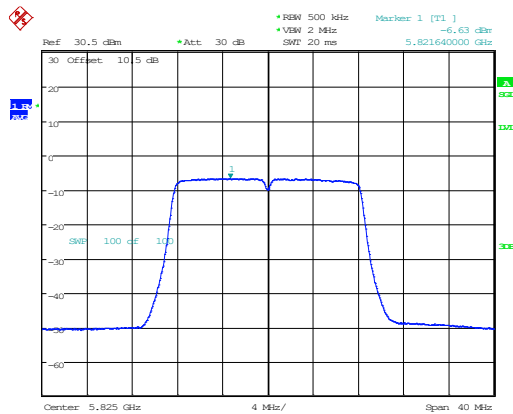
802.11a_5825MHz_Chain 1
