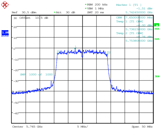
802.11ac20_5745MHz_Chain 0
