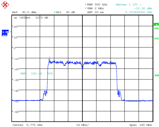
802.11ax80_5775MHz_RU_Full_Chain 1
