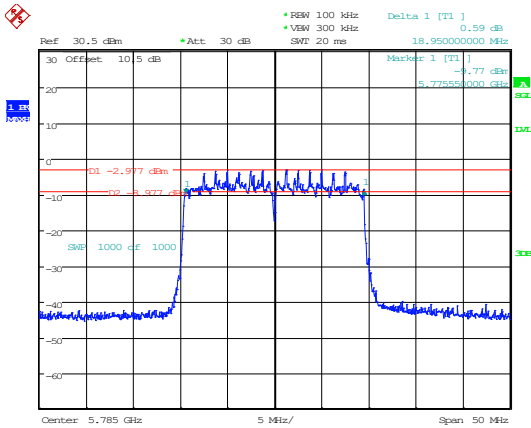
802.11ax20_5785MHz_RU_Full_Chain 0
