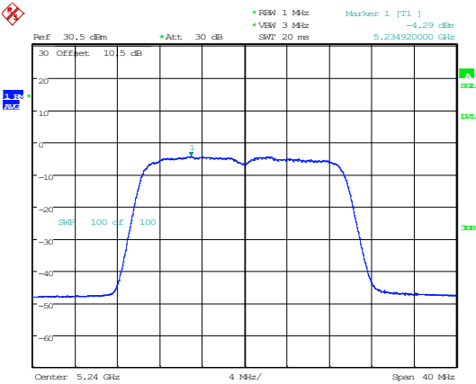
802.11ax20_5240MHz_RU_Full_Chain 0
