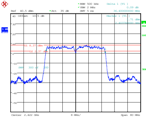
802.11n40_2422MHz_Chain 0
