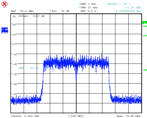
802.11ax40_2422MHz_RU_Full_Chain 0
