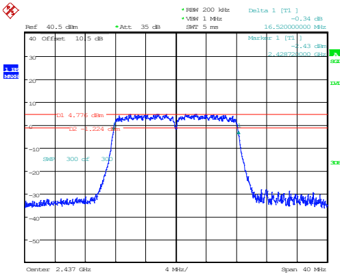
802.11g_2437MHz_Chain 1
