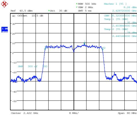
802.11n40_2422MHz_Chain 0
