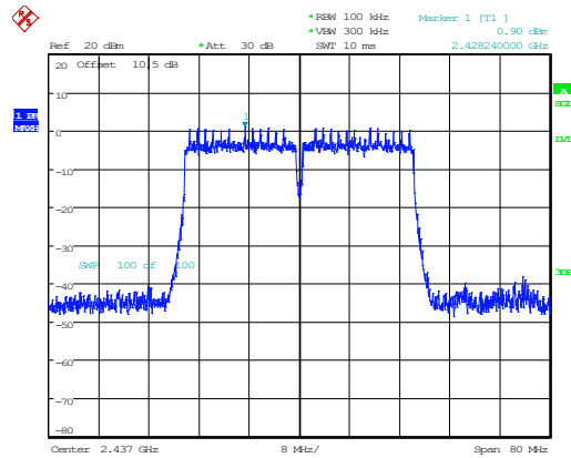
802.11n40_2437MHz_Chain 0
