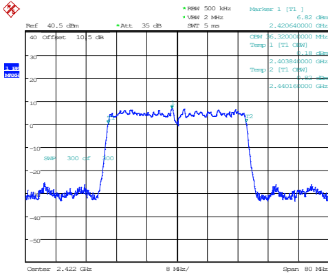
802.11n40_2422MHz_Chain 1
