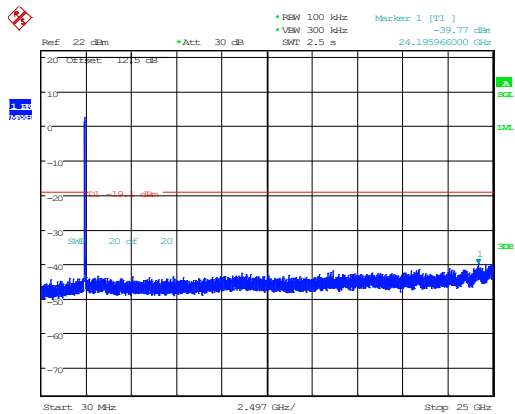
802.11n40_2437MHz_Chain 0
