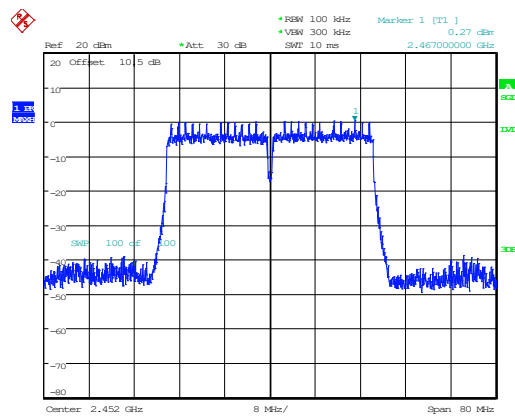
802.11n40_2452MHz_Chain 1
