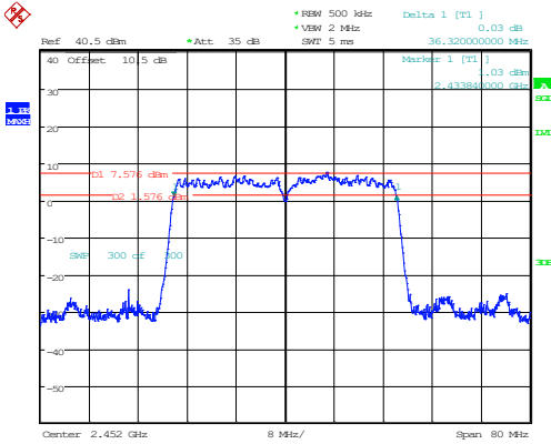
802.11n40_2452MHz_Chain 0
