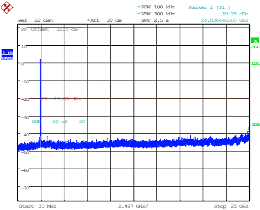
802.11ax40_2437MHz_RU_Full_Chain 1
