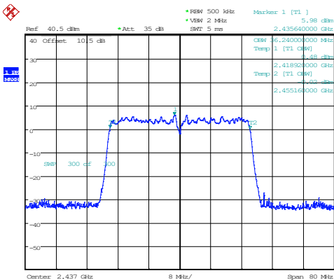
802.11n40_2437MHz_Chain 1
