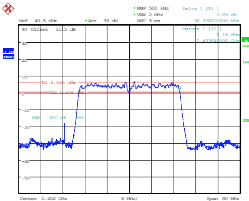
802.11n40_2452MHz_Chain 1
