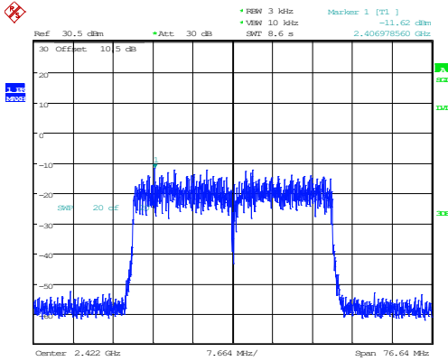
802.11ax40_2422MHz_RU_Full_Chain 1
