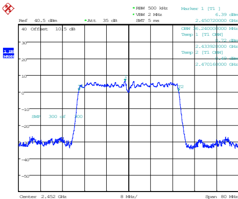
802.11n40_2452MHz_Chain 1
