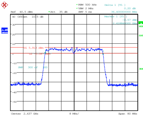
802.11n40_2437MHz_Chain 1
