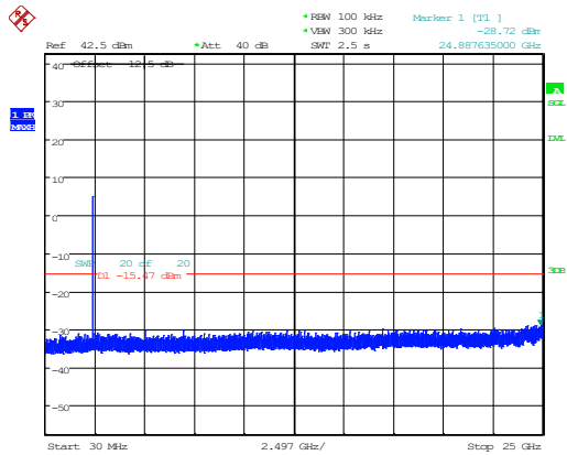
802.11g_2412MHz_Chain 1
