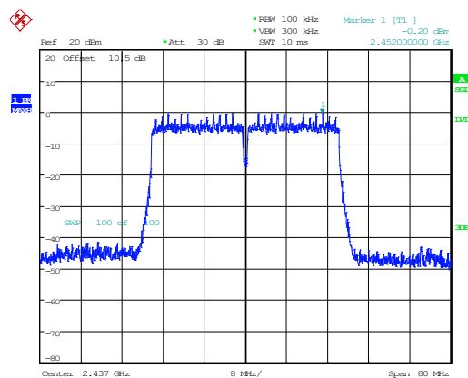
802.11n40_2437MHz_Chain 1
