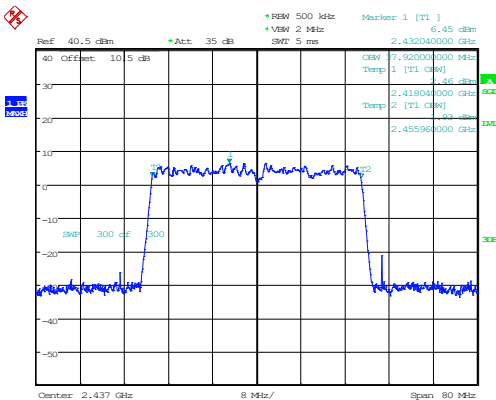
802.11ax40_2437MHz_RU_Full_Chain 1
