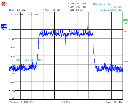
802.11ax40_2437MHz_RU_Full_Chain 1
