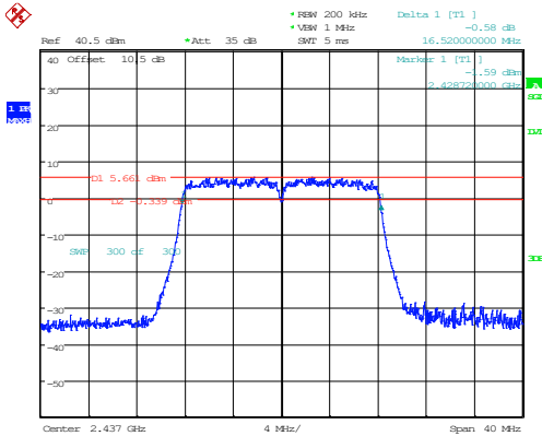
802.11g_2437MHz_Chain 0
