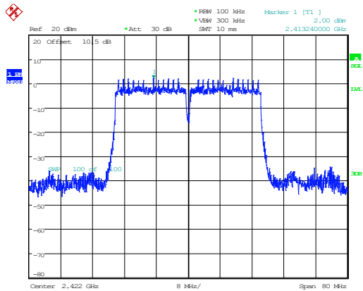
802.11n40_2422MHz_Chain 0
