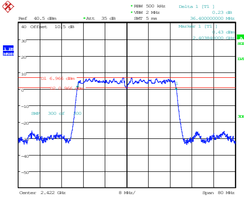
802.11n40_2422MHz_Chain 1
