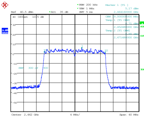
802.11ax20_2462MHz_RU_Full_Chain 1
