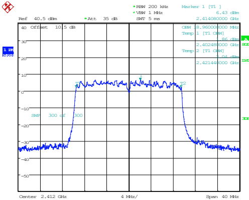
802.11ax20_2412MHz_RU_Full_Chain 0
