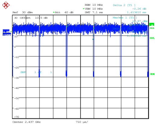
802.11g_2437MHz_Chain 0
