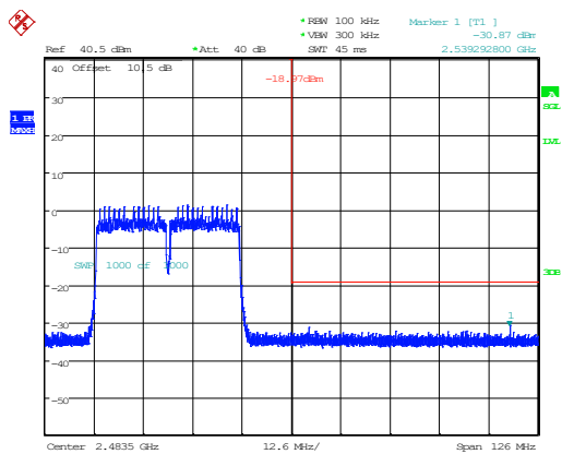
802.11n40_2452MHz_Chain 0
