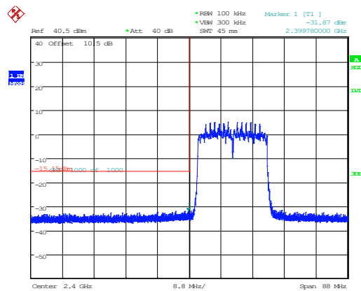
802.11ax20_2412MHz_RU_Full_Chain 0
