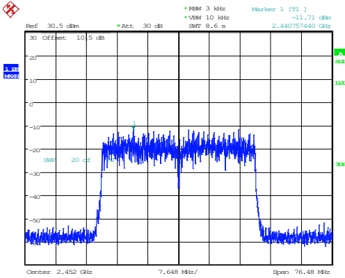
802.11ax40_2452MHz_RU_Full_Chain 0
