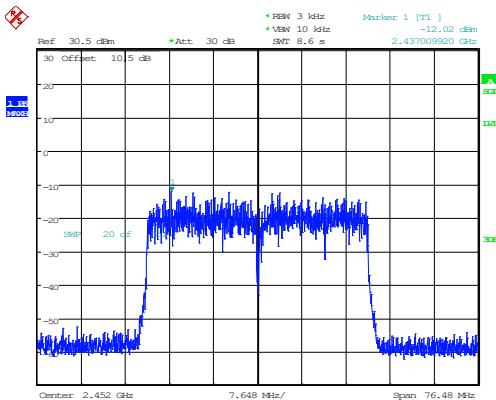
802.11ax40_2452MHz_RU_Full_Chain 1
