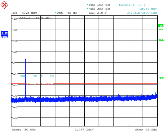
802.11ax40_2422MHz_RU_Full_Chain 1
