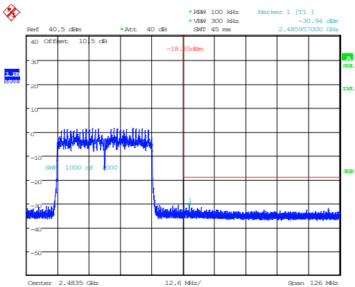
802.11ax40_2452MHz_RU_Full_Chain 0
