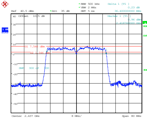
802.11n40_2437MHz_Chain 0
