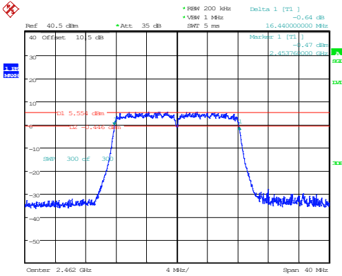
802.11g_2462MHz_Chain 0
