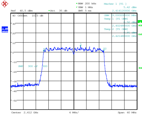
802.11ax20_2412MHz_RU_Full_Chain 1
