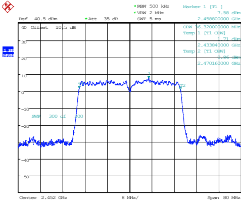
802.11n40_2452MHz_Chain 0
