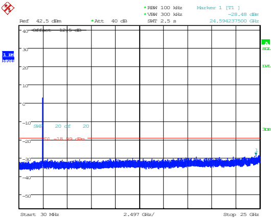
802.11ax40_2452MHz_RU_Full_Chain 1
