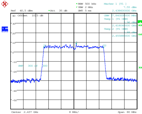
802.11ax40_2437MHz_RU_Full_Chain 0
