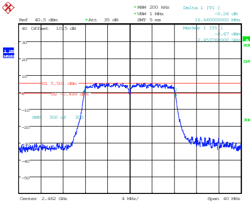
802.11g_2462MHz_Chain 1
