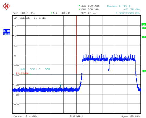
802.11n40_2422MHz_Chain 1
