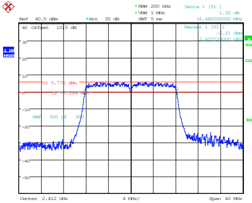
802.11g_2412MHz_Chain 1
