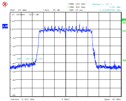
802.11ax20_2412MHz_RU_Full_Chain 1
