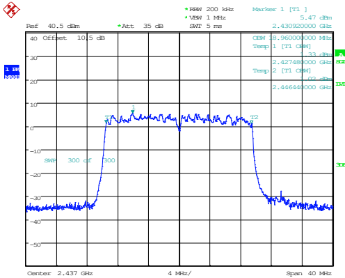
802.11ax20_2437MHz_RU_Full_Chain 0
