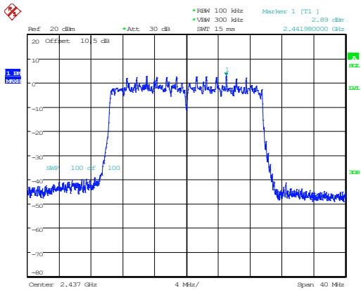
802.11ax20_2437MHz_RU_Full_Chain 1
