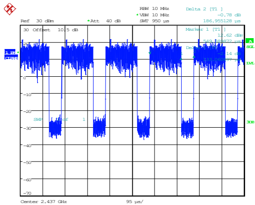
802.11ax20_2437MHz_RU_Full_Chain 0
