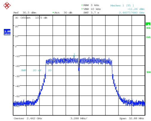
802.11g_2462MHz_Chain 0
