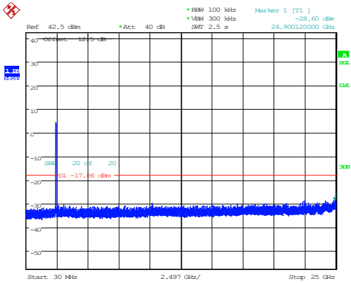
802.11ax40_2422MHz_RU_Full_Chain 0
