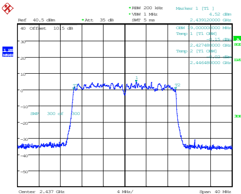
802.11ax20_2437MHz_RU_Full_Chain 1
