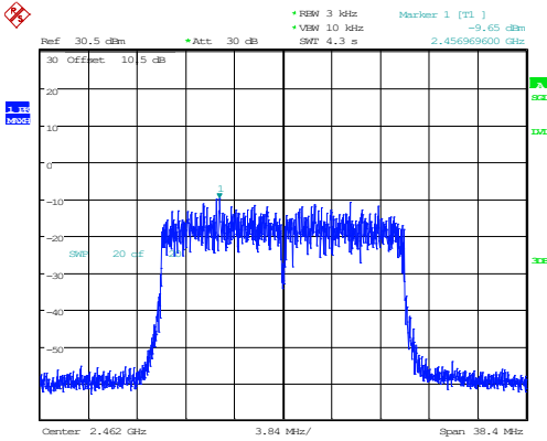
802.11ax20_2462MHz_RU_Full_Chain 0
