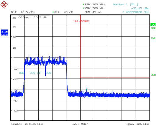
802.11ax40_2452MHz_RU_Full_Chain 1
