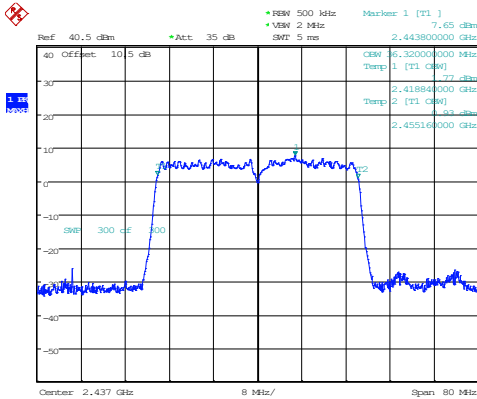
802.11n40_2437MHz_Chain 0
