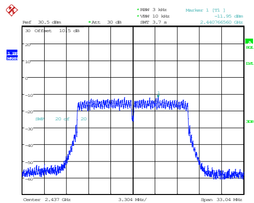
802.11g_2437MHz_Chain 1
