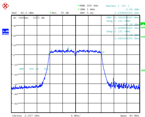
802.11g_2437MHz_Chain 1
