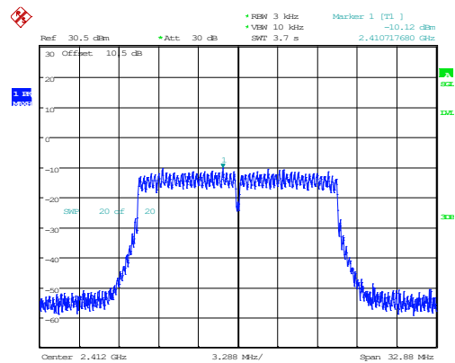
802.11g_2412MHz_Chain 0
