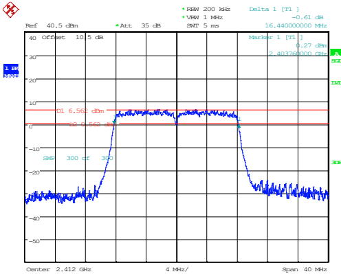
802.11g_2412MHz_Chain 0
