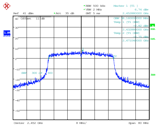
802.11ax40_2452MHz_RU_Full
