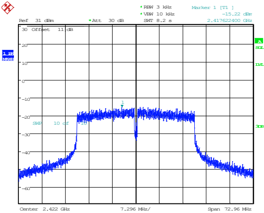
802.11n40_2422MHz
