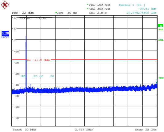
802.11ax20_2437MHz_RU_Full
