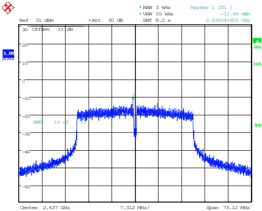
802.11n40_2437MHz
