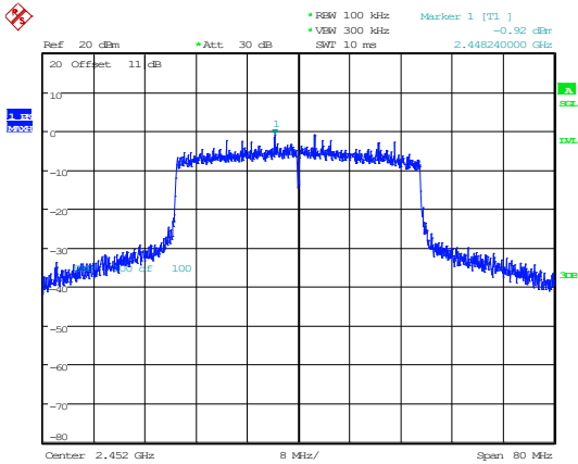
802.11ax40_2452MHz_RU_Full
