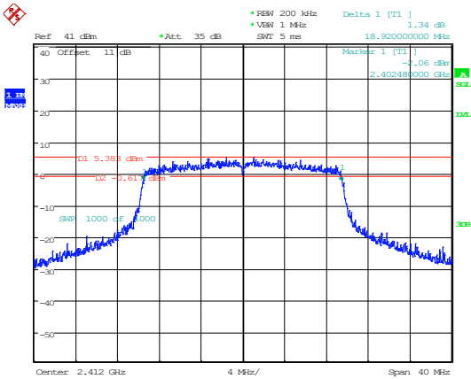
802.11ax20_2412MHz_RU_Full
