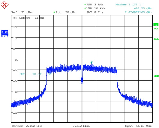
802.11n40_2452MHz
