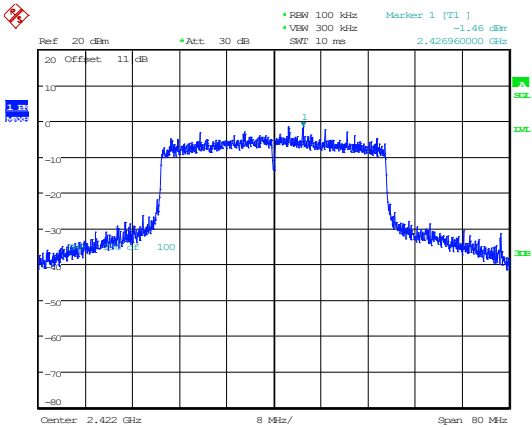
802.11ax40_2422MHz_RU_Full
