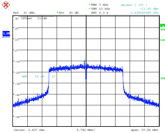
802.11ax20_2437MHz_RU_Full
