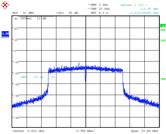
802.11ax20_2412MHz_RU_Full
