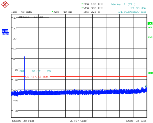
802.11ax20_2462MHz_RU_Full
