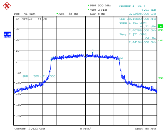
802.11ax40_2422MHz_RU_Full
