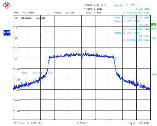
802.11ax20_2437MHz_RU_Full
