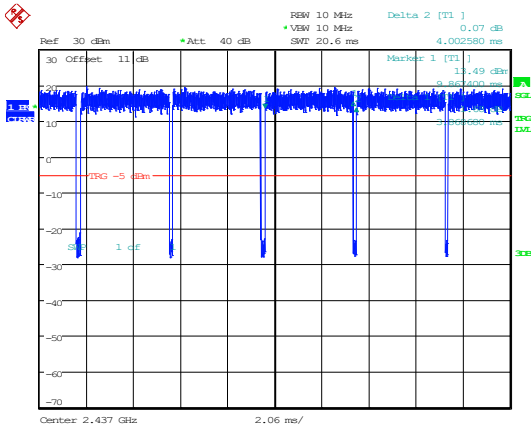
802.11ax40_2437MHz_RU_Full
