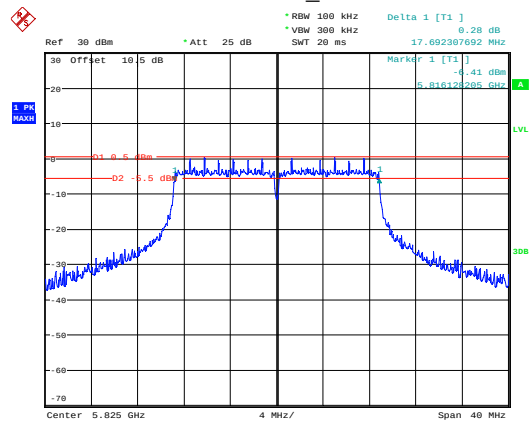
802.11 n20_5825MHz
