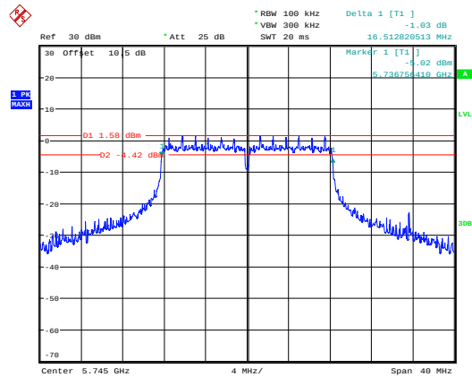
802.11 a_5745MHz
