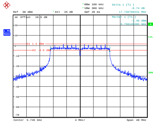
802.11 n20_5745MHz
