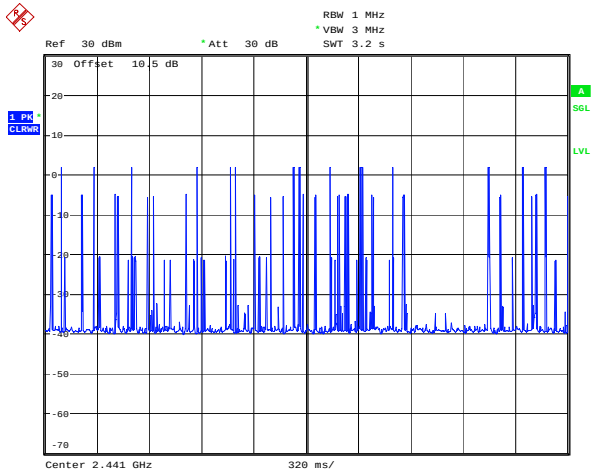
BDR_DH3_Hopping
