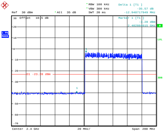
2EDR_DH1_Hopping_Lower
