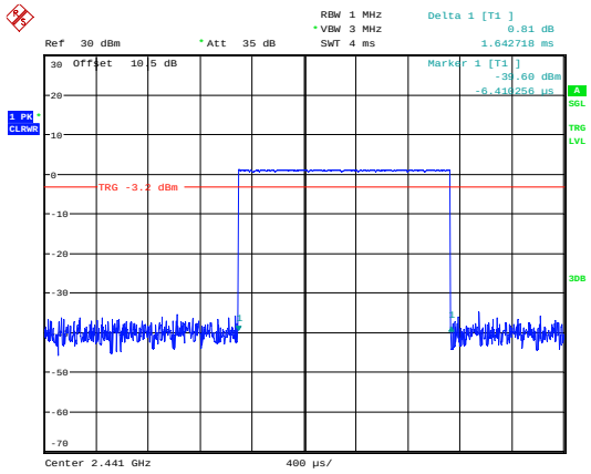
BDR_DH3_Hopping
