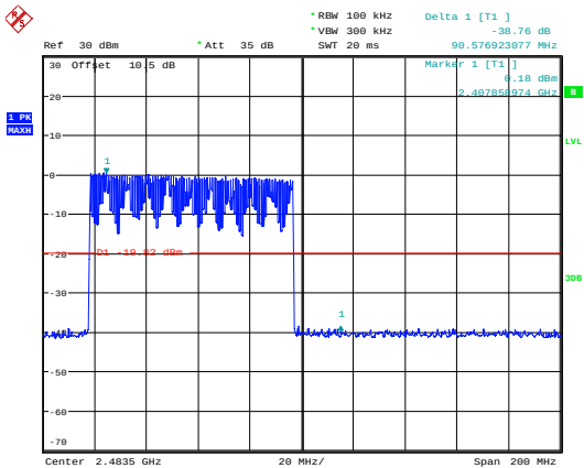
BDR_DH1_Hopping_Upper
