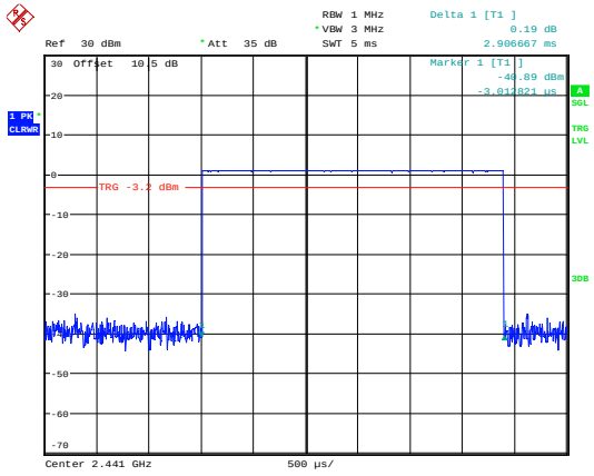
BDR_DH5_Hopping
