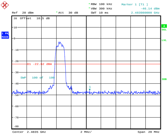
2EDR_DH1_High
