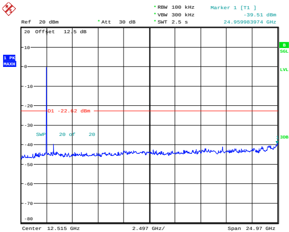
2EDR_DH1_High
