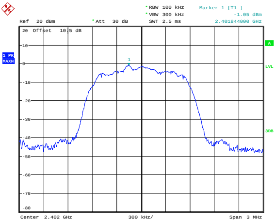
3EDR_DH1_Low
