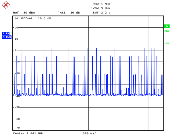
BDR_DH5_Hopping
