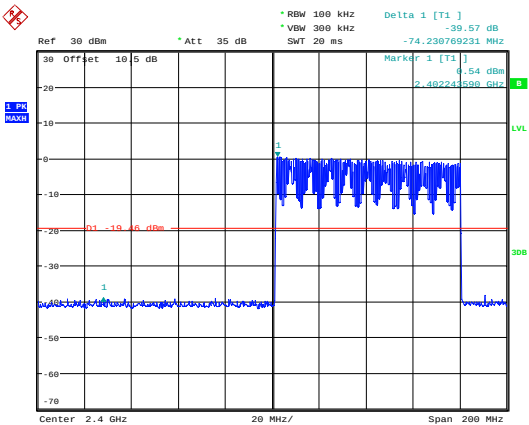
BDR_DH1_Hopping_Lower
