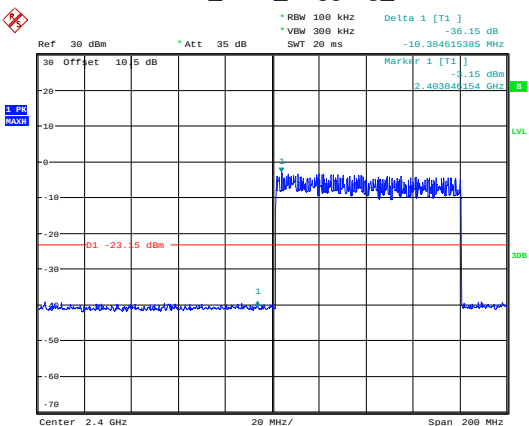
3EDR_DH1_Hopping_Lower
