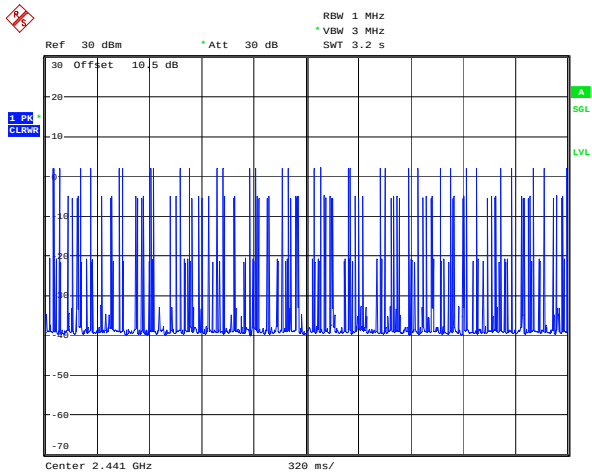
BDR_DH1_Hopping
