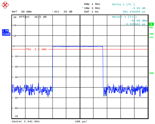
BDR_DH1_Hopping
