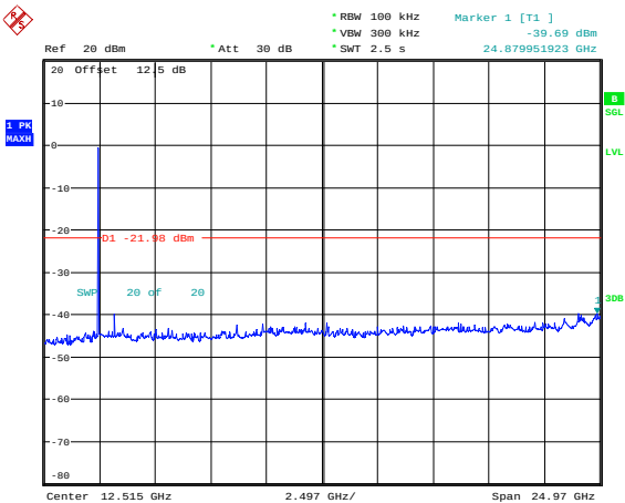
2EDR_DH1_Middle
