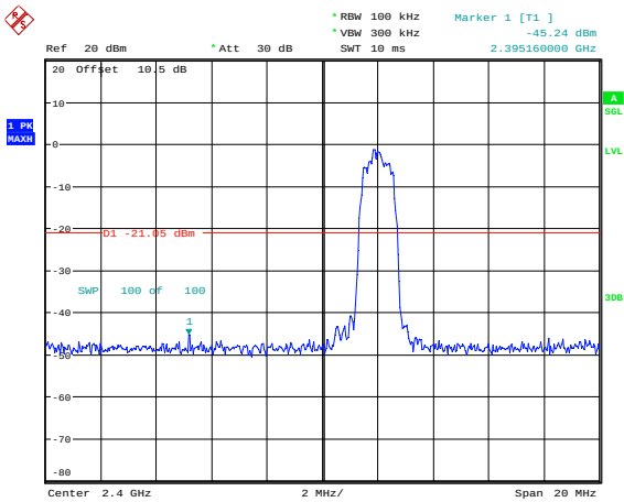
3EDR_DH1_Low
