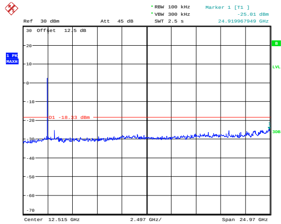
BLE_1M_Middle_Channel
