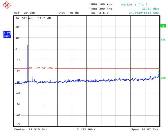
BLE_1M_Low_Channel
