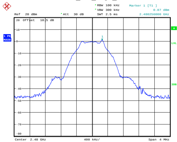
BLE_1M_High_Channel
